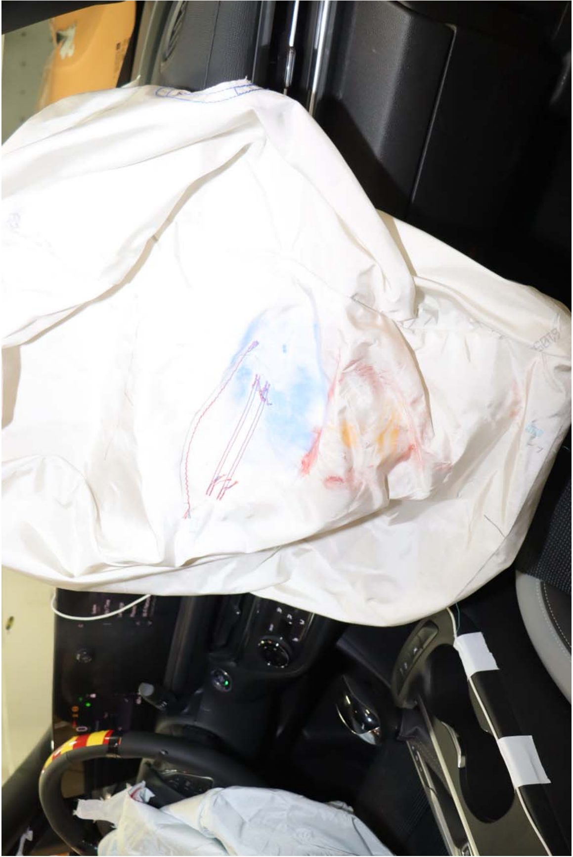
Photo No. 59. Post-Test Passenger Dummy Airbag Contact
