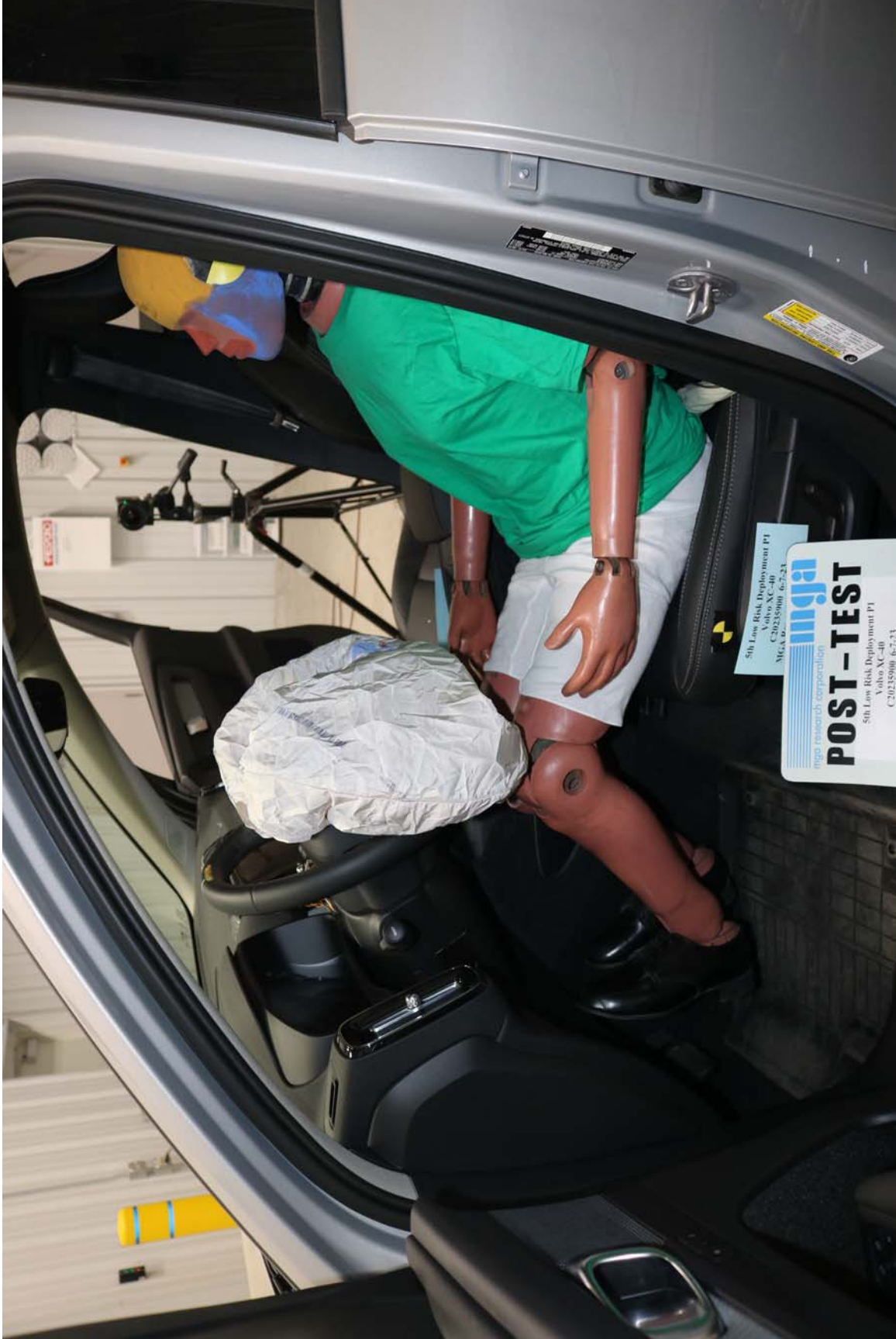
Photo No. 2 - Post-Test 5th Fem. P1 Driver Dummy Left Side View
