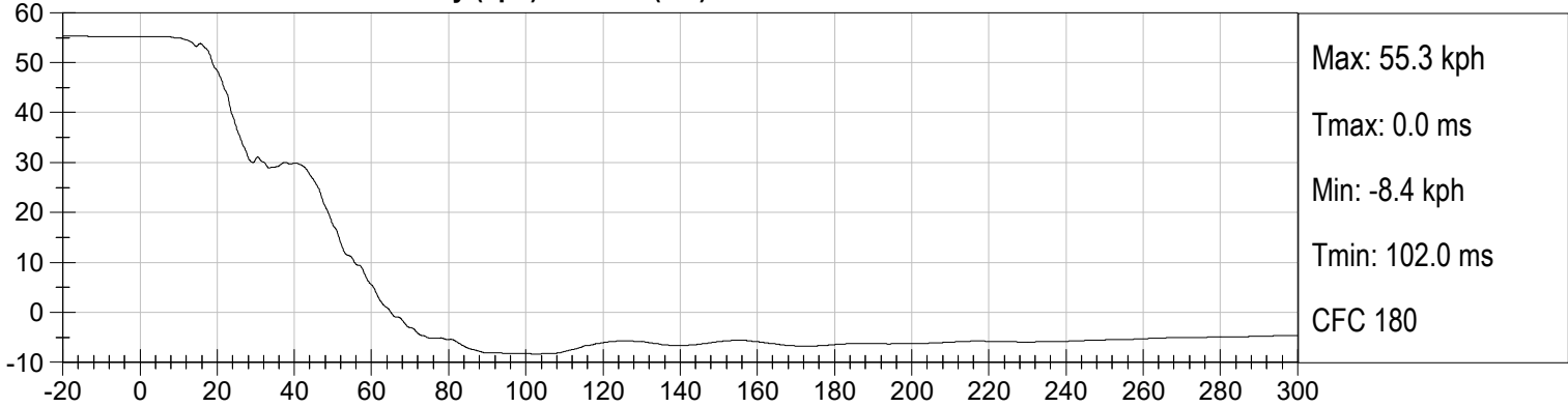
TRUNK Z (g) vs Time (ms)
