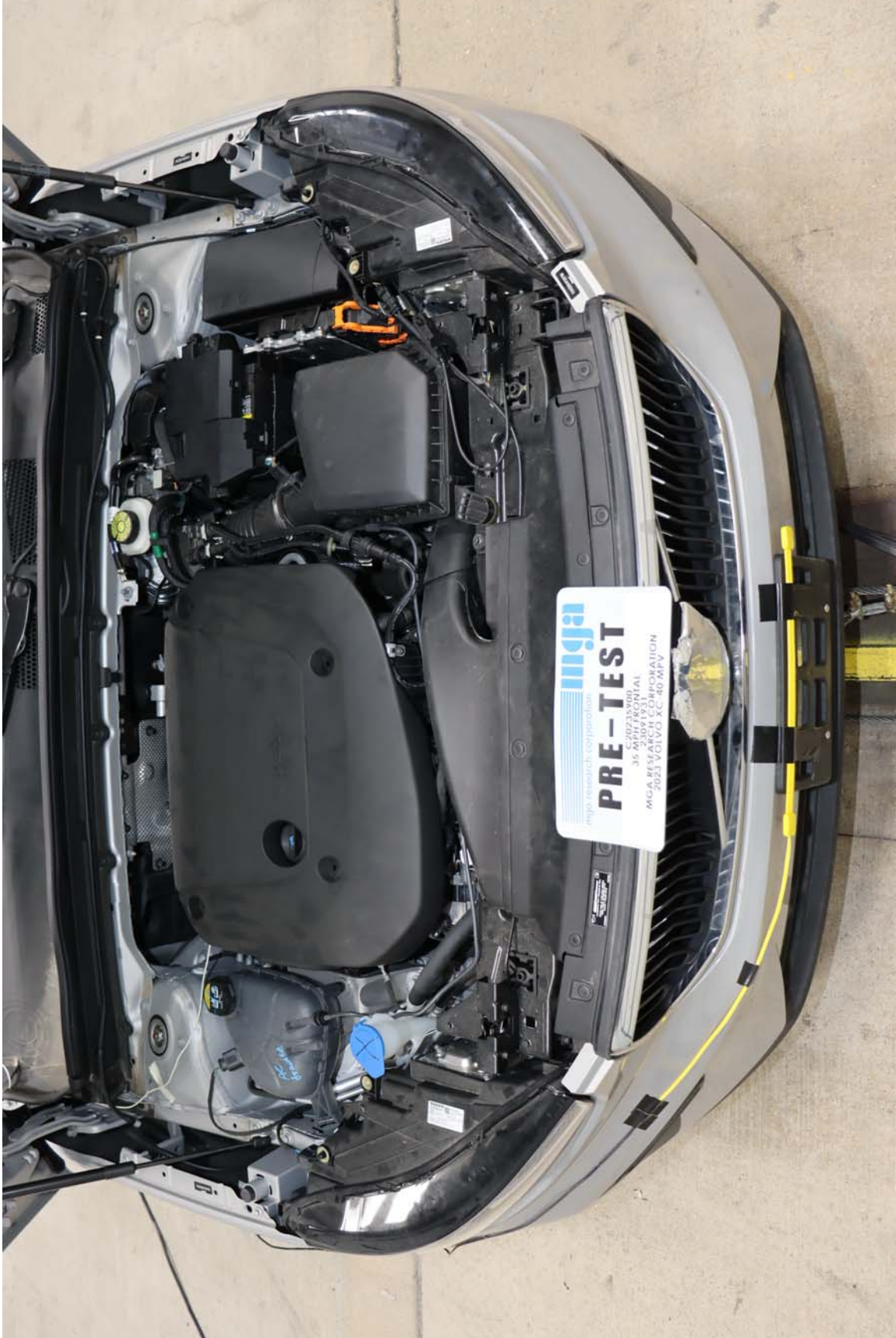
Photo No. 21 - Pre-Test Engine Compartment View
