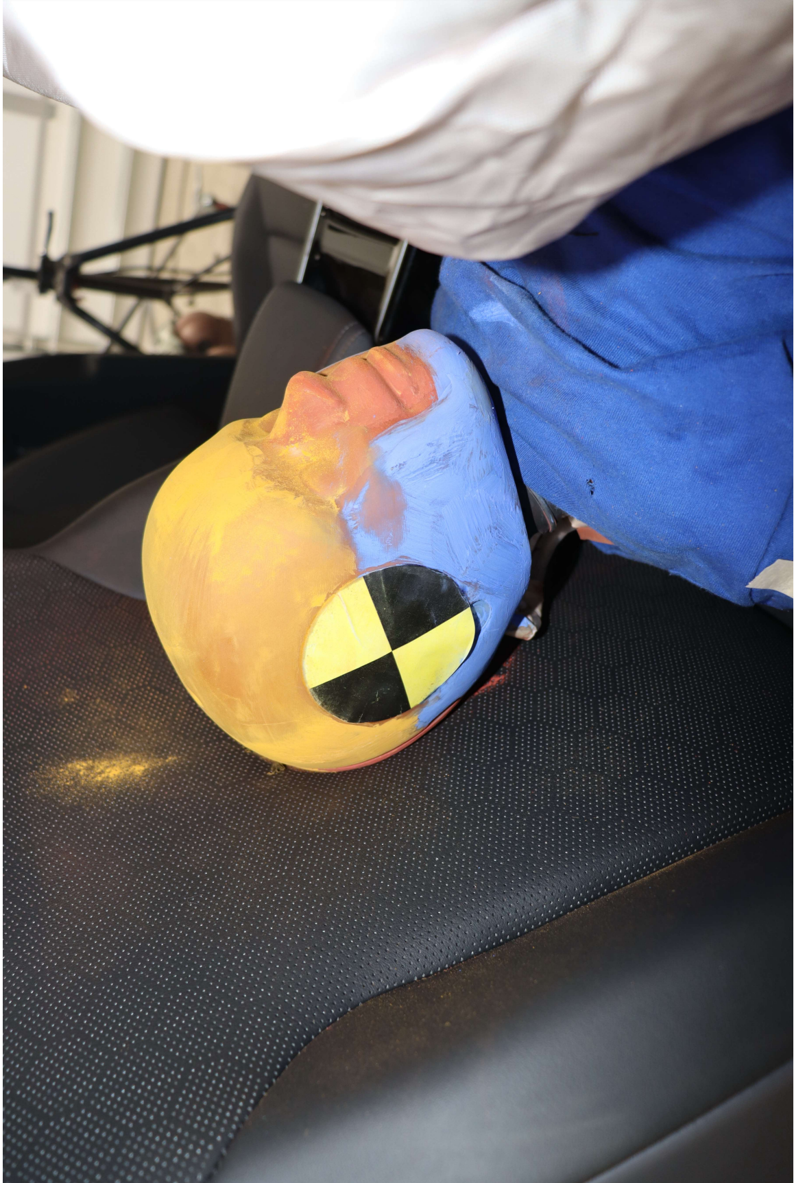
Photo No. 27 - Post-Test 3YO P2 Passenger Dummy Head Contact (seat back)
