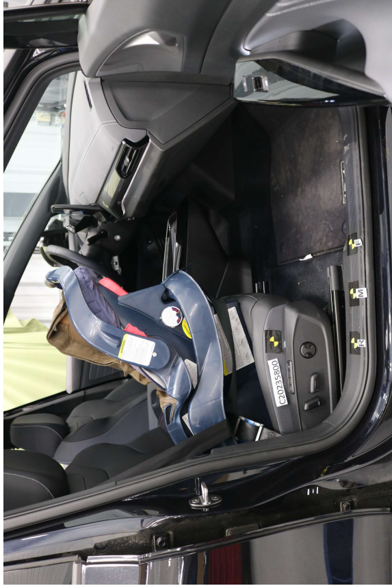
Graco Snuggly WBBase, Belted, Rear Facing, Rearward Seat Track
