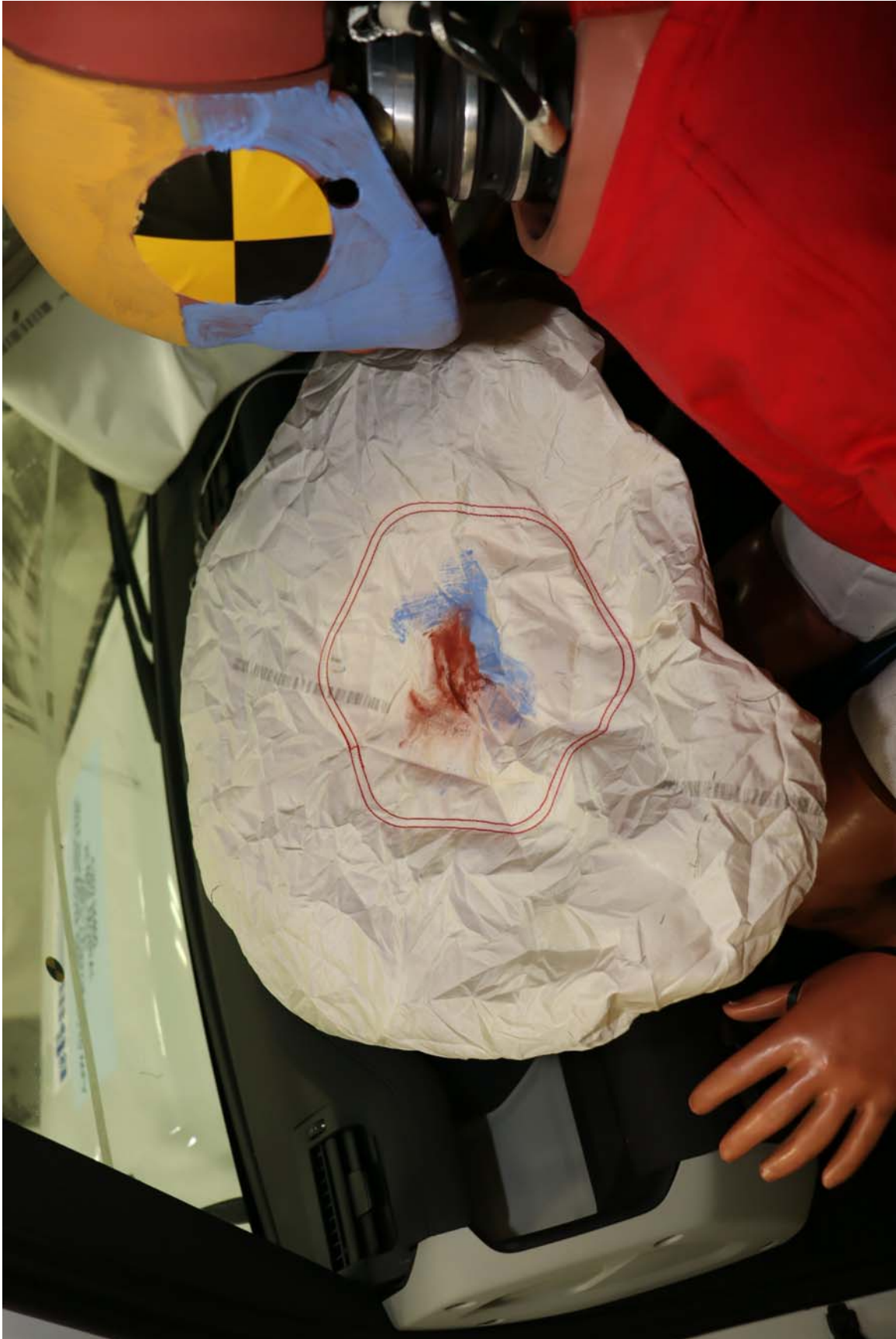
Photo No. 45. Post-Test Driver Dummy Airbag Contact
