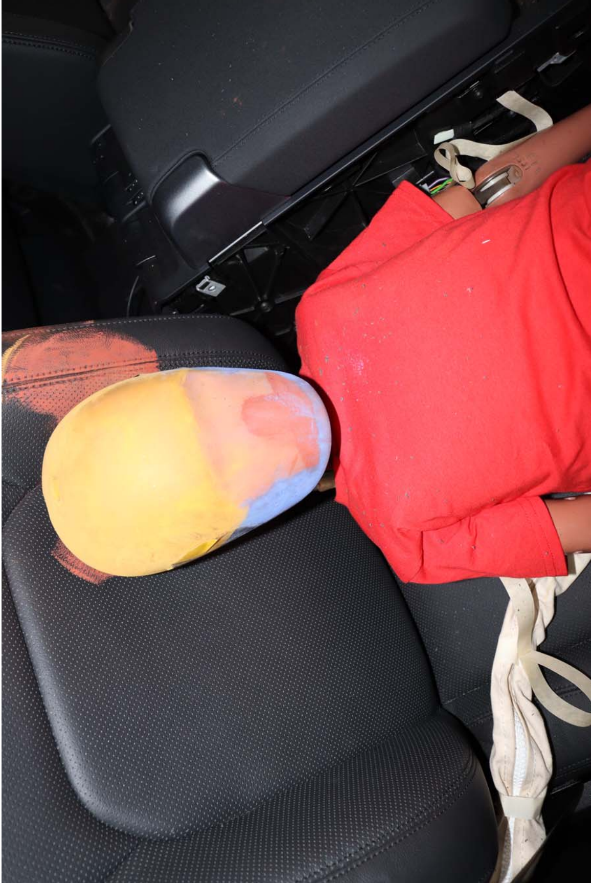
Photo No. 35 - Post-Test 6YO P1 Passenger Dummy Head Contact (seat)
