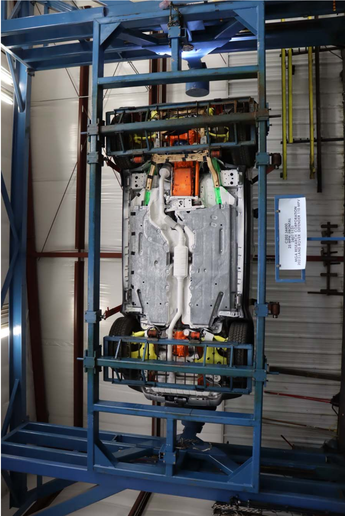
Photo No. 65. Rollover 270 Degrees
