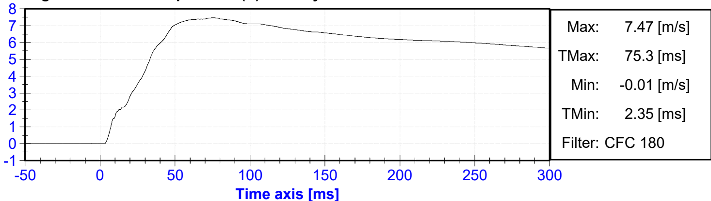
Right Rear Occ. Compartment(Y) Velocity vs. Time
