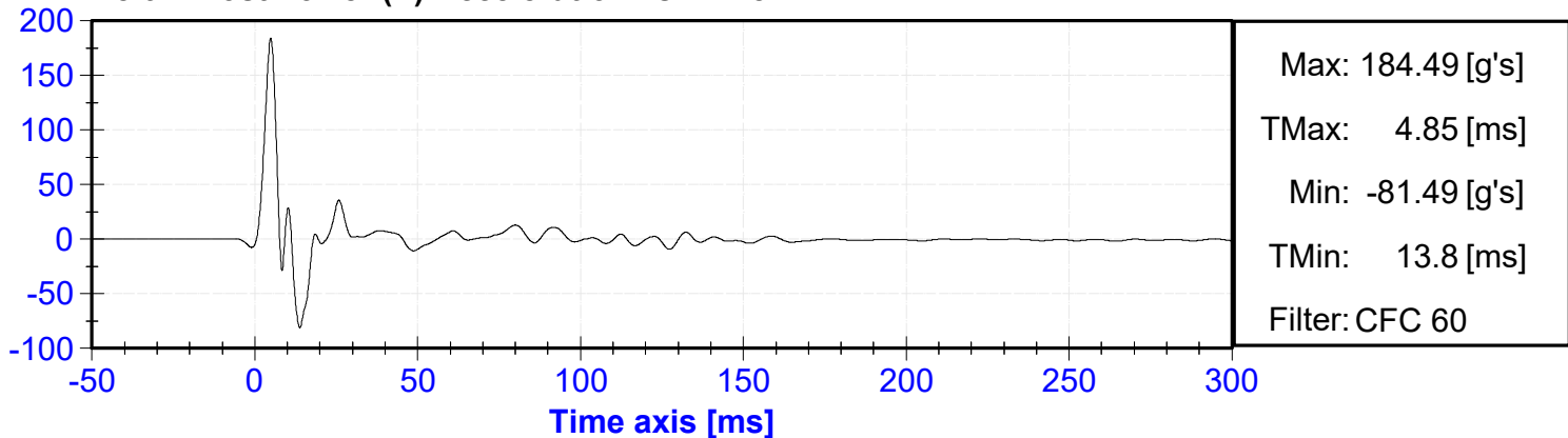
Left B-Post Lower (Y) Acceleration vs. Time
