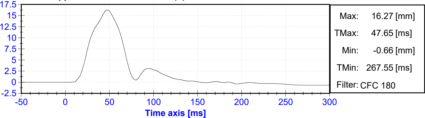
ES-2re Middle Thorax Rib Deflection Rate vs. Time
