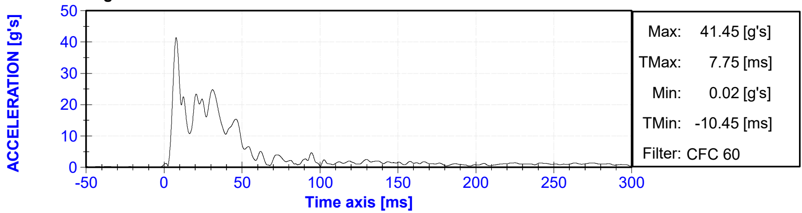
Rear Floorpan Above Axle (X) Acceleration vs. Time
