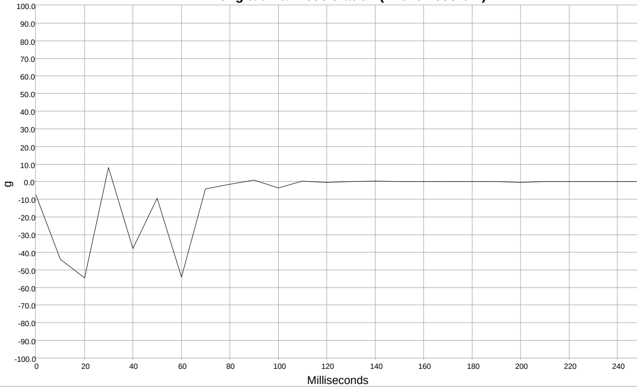
Longitudinal Acceleration (Event Record 1)
