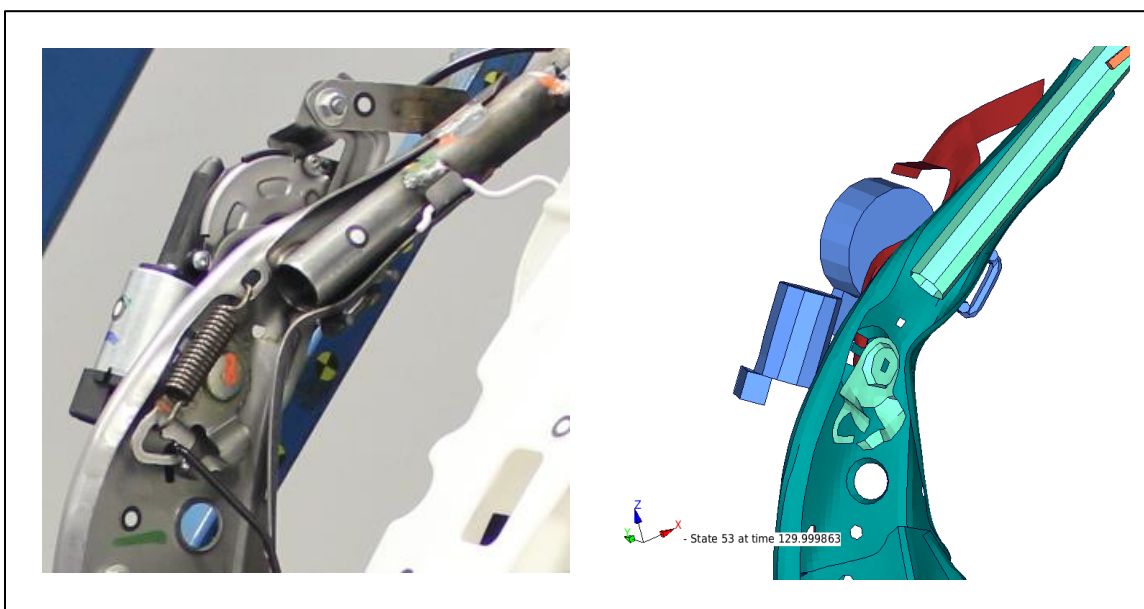
Figure 21: Similar deformation of RHS Seat Frame Test vs FEA – Power Seat
