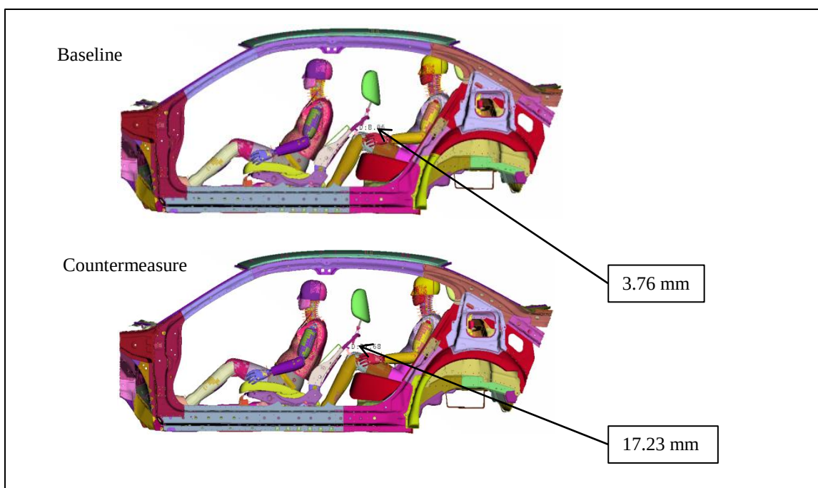
Figure 56: Seat back to Knee clearance (Baseline and Countermeasure – Power Seat)
