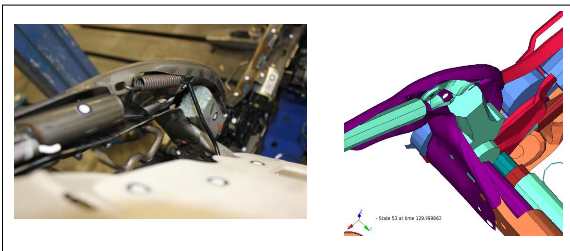
Figure 20: Similar deformation of LHS Seat Frame Test vs FEA – Power Seat
