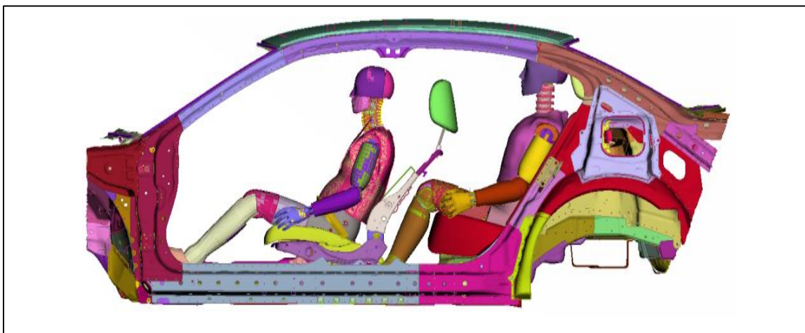
Figure 70: Illustration of Front Seat Interaction on 90 th %ile Rear Seat Occupant
