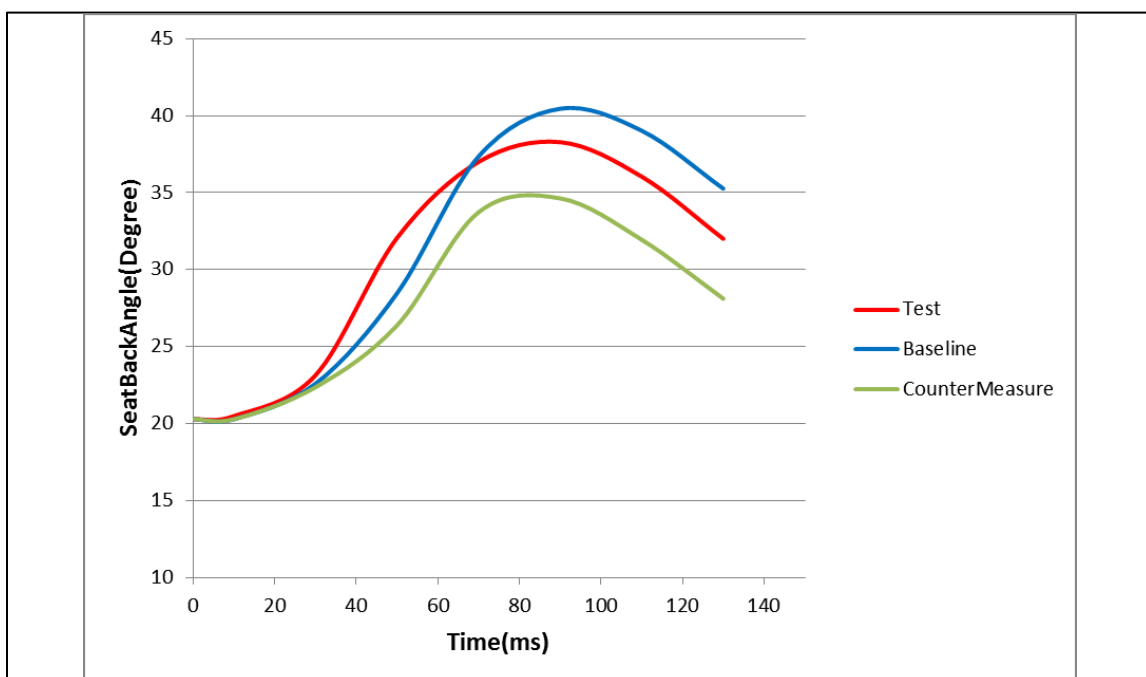
Figure 46: Seat back Rotation Comparison (Manual Seat)
