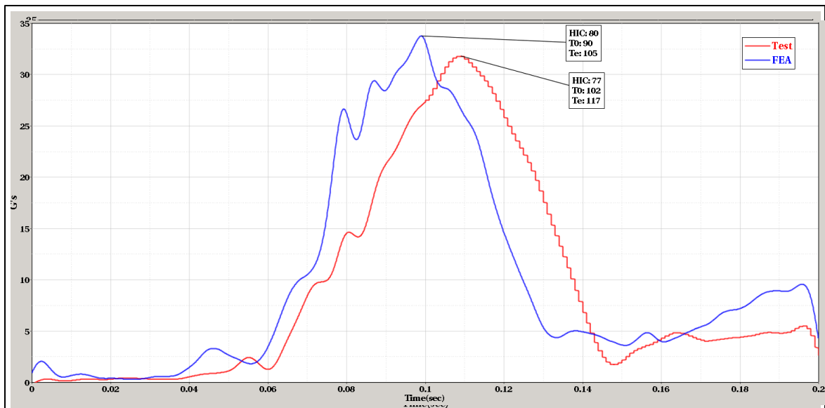
Figure 35: Head Acceleration – Manual Seat
