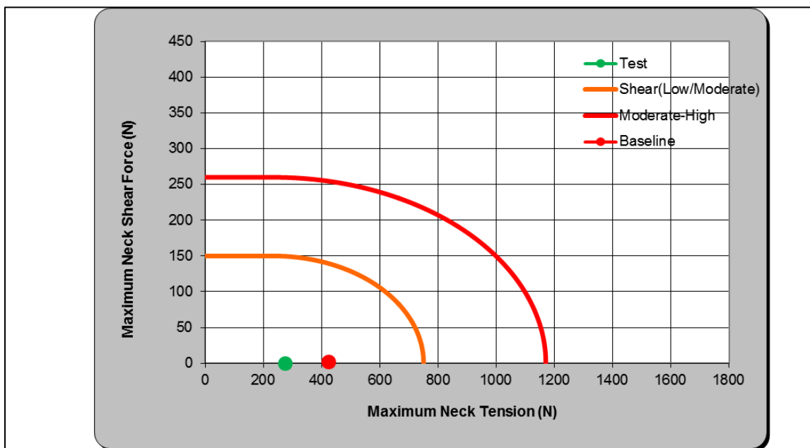
Figure 62: IIHS Vehicle Seat Head Restraint Test – Neck Injury Rating, Baseline vs. Test
