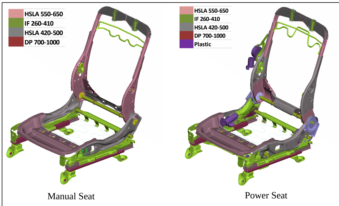
Figure 10: MY 2014 Detailed FE Models
