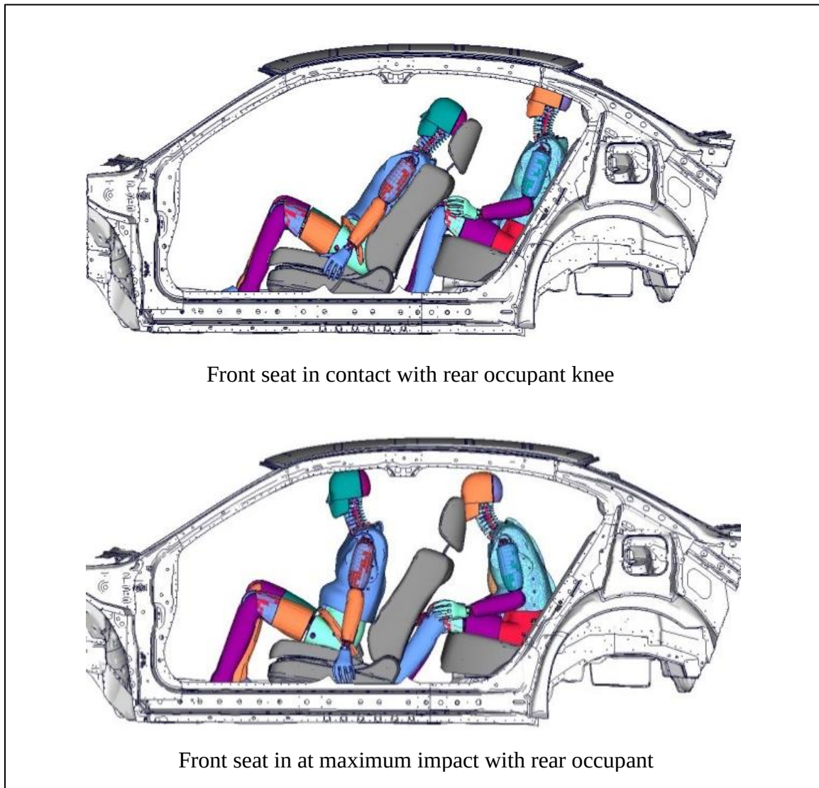
Figure 42: Front Seat Back and Rear Seat Occupant Interaction – Manual Seat
