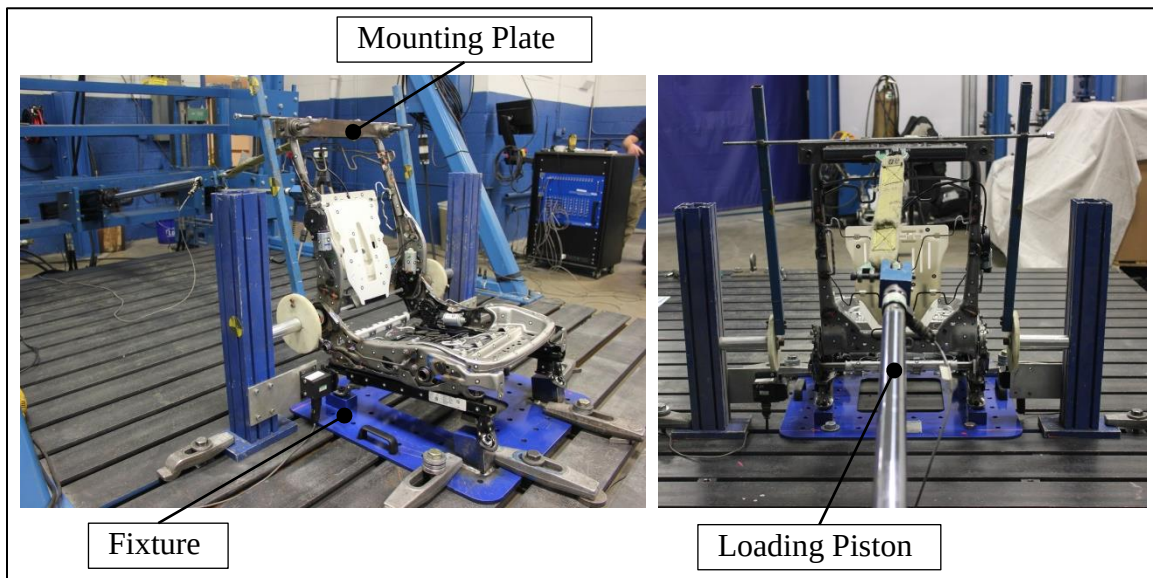
Figure 6: Seat Back Pull Test Setup – Power Seat
