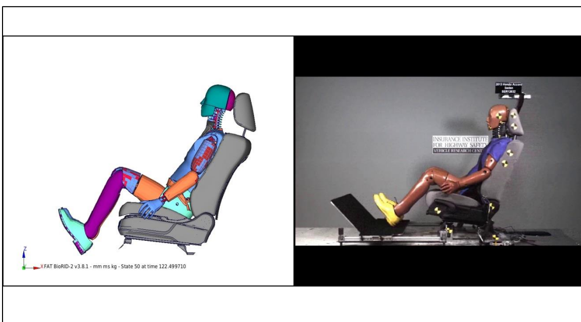
Figure 61: IIHS Vehicle Seat Head Restraint Test – Baseline vs. Test (Manual Seat)
