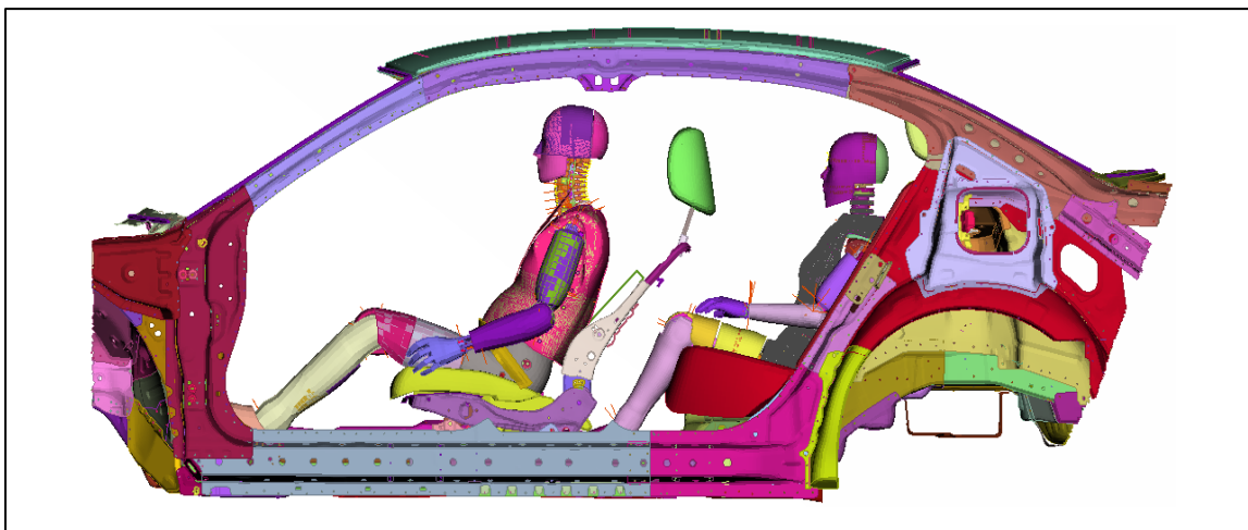
Figure 69: Illustration of Front Seat Interaction on 5 th %ile Rear Seat Occupant
