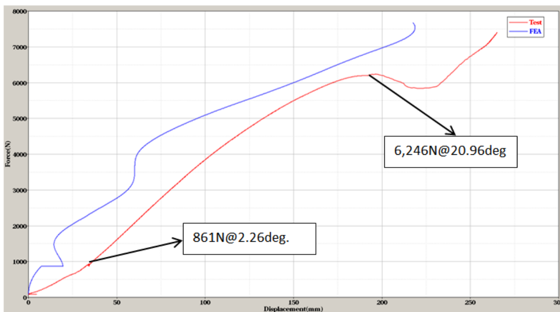
Figure 23: Force vs. Displacement Curves – Power Seat
