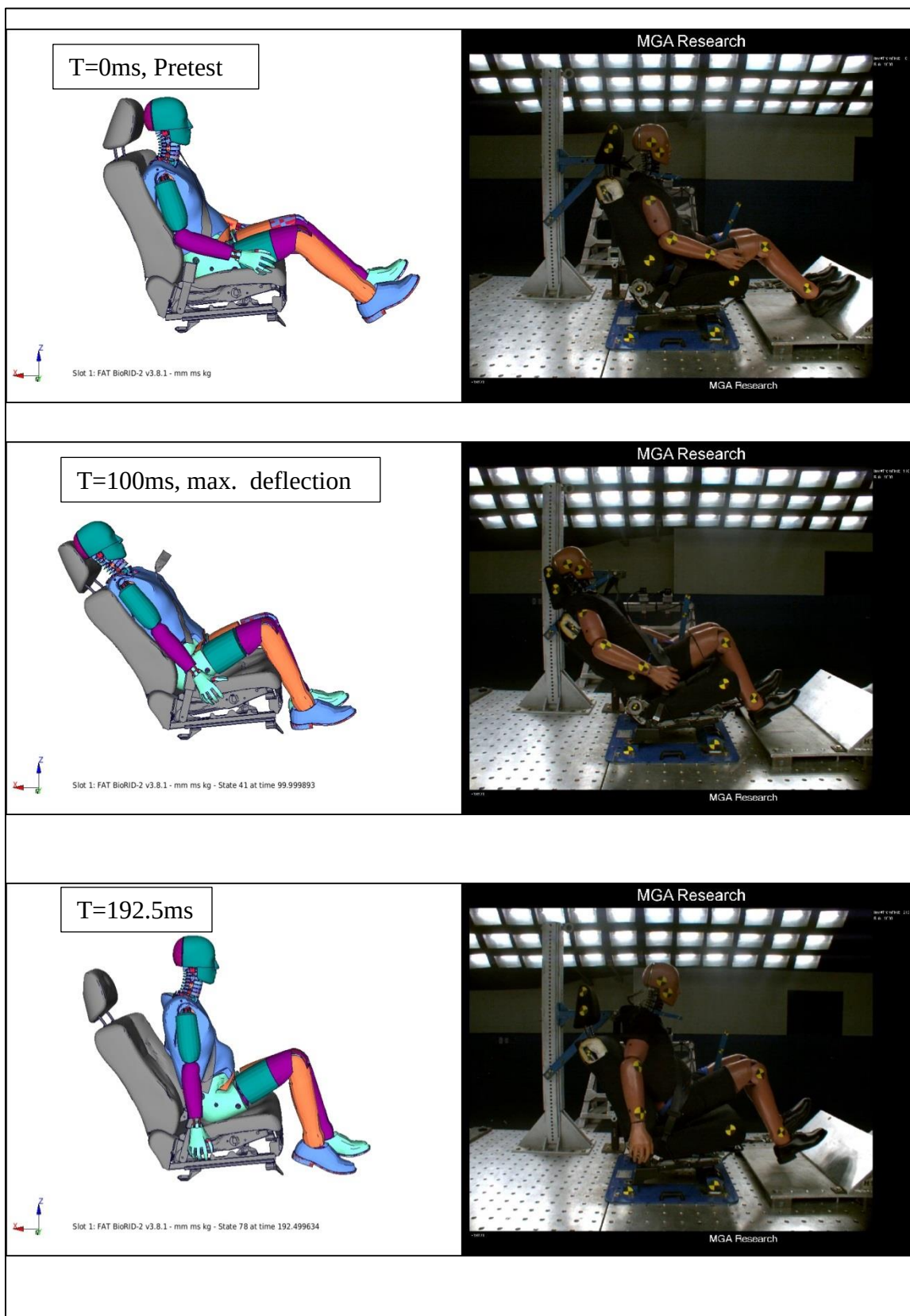
Figure 33: FMVSS301 Sled Test FEA and Test – Manual Seat
