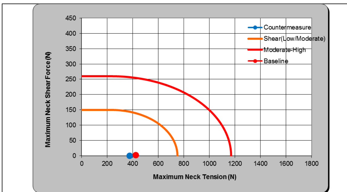
Figure 65: IIHS Neck Injury Rating Chart – Countermeasure vs. Baseline (Manual Seat)
