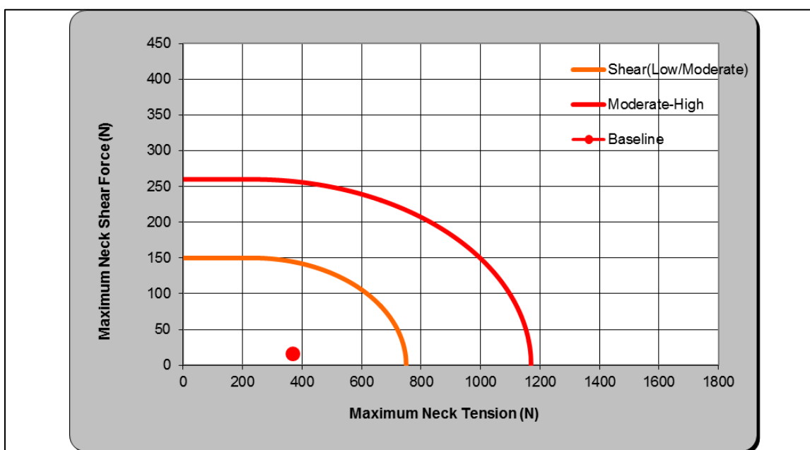
Figure 64: IIHS Vehicle Seat Head Restraint Test – Neck Injury Rating, Baseline (Power Seat)
