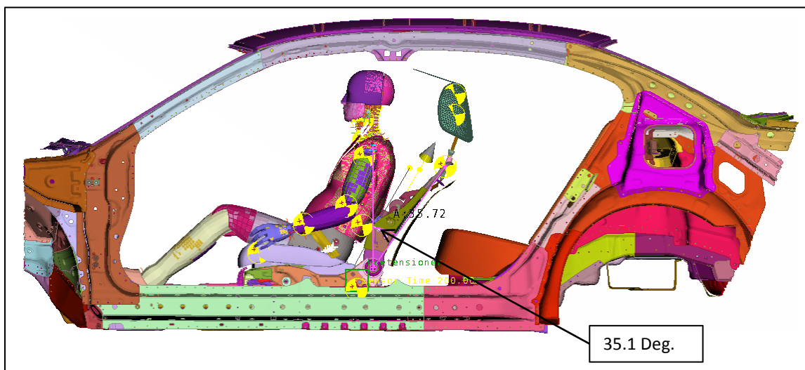
Figure 55: Seat back Angle (Countermeasure – Power Seat)
