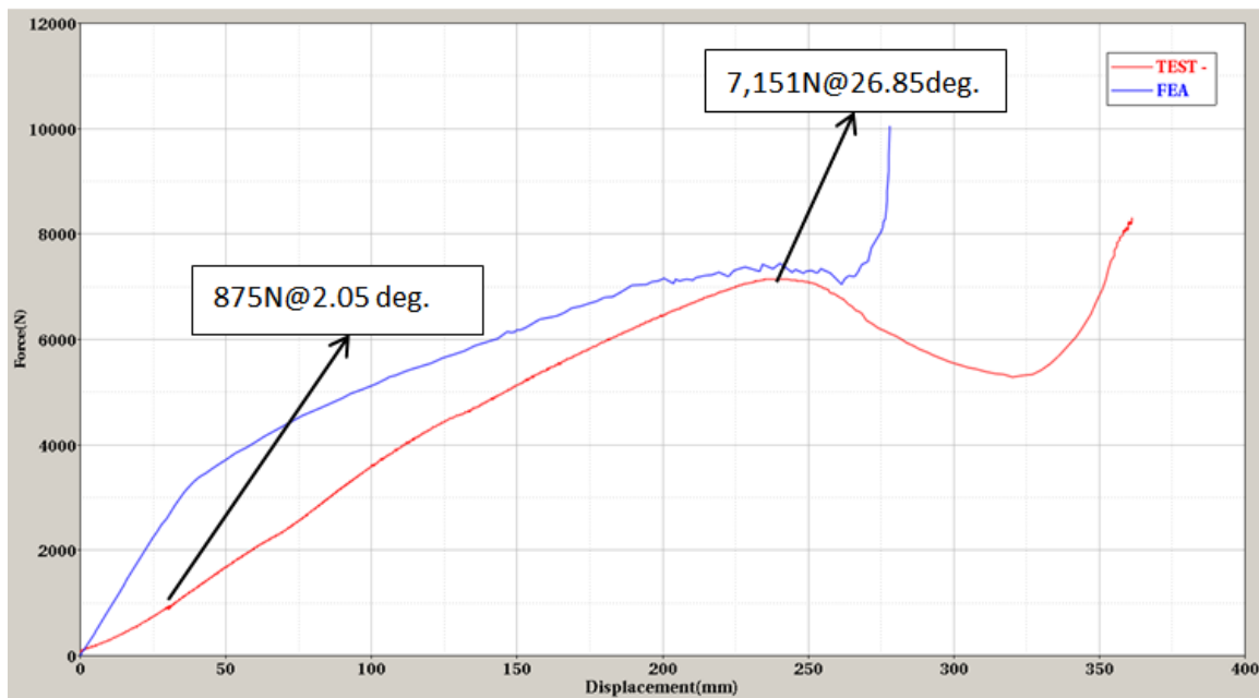
Figure 17: Force vs. Displacement Curves – Manual Seat
