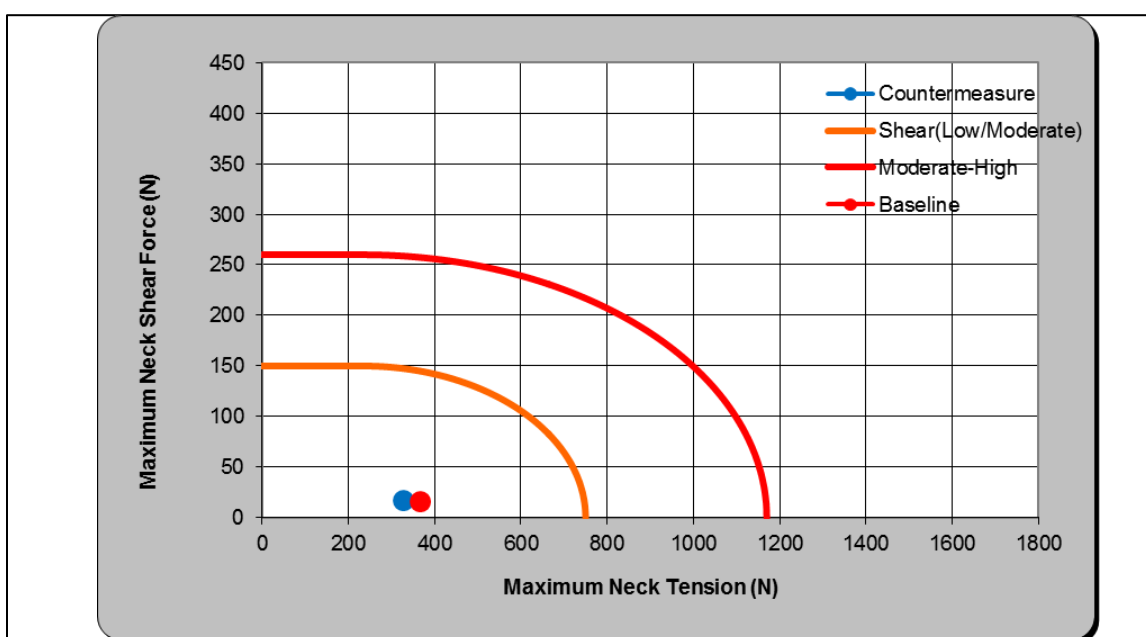
Figure 66: IIHS Neck Injury Rating Chart – Countermeasure vs. Baseline (Power Seat)
