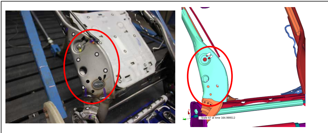
Figure 15: Similar deformation of RHS Seat Frame Test vs FEA – Manual Seat
