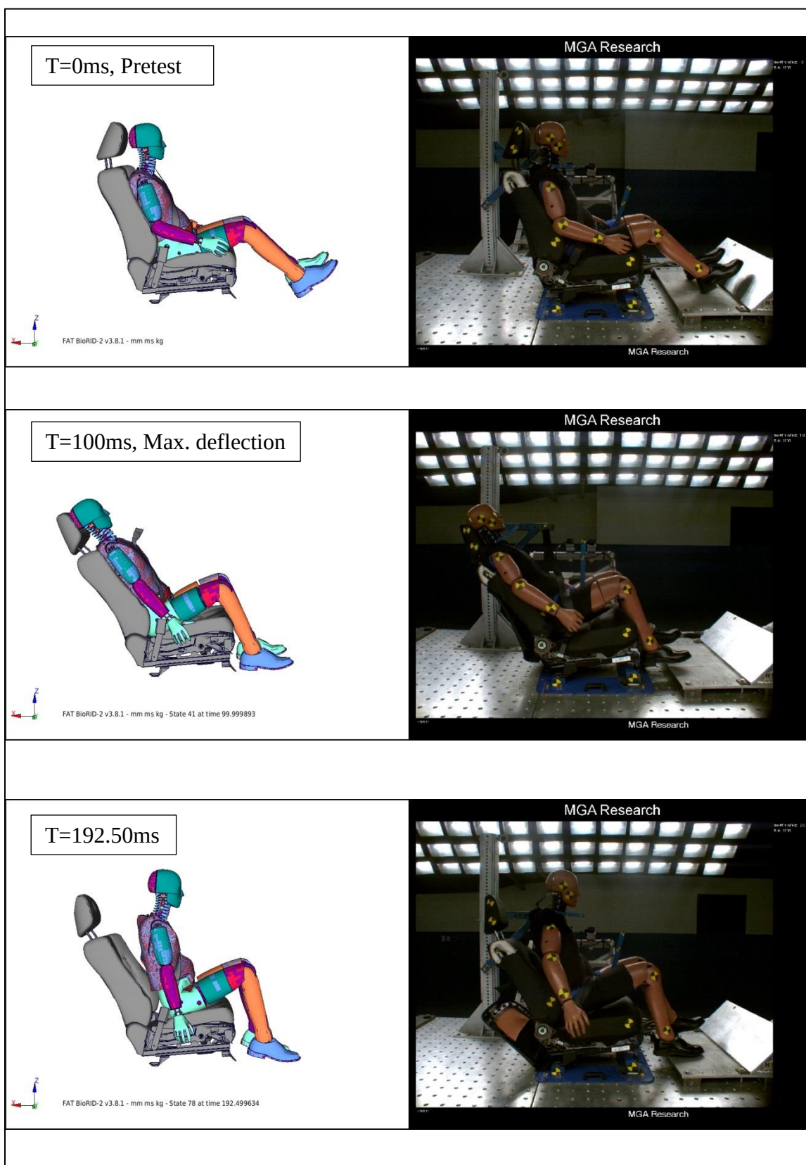
Figure 37: FMVSS301 Sled Test FEA and Test – Power Seat
