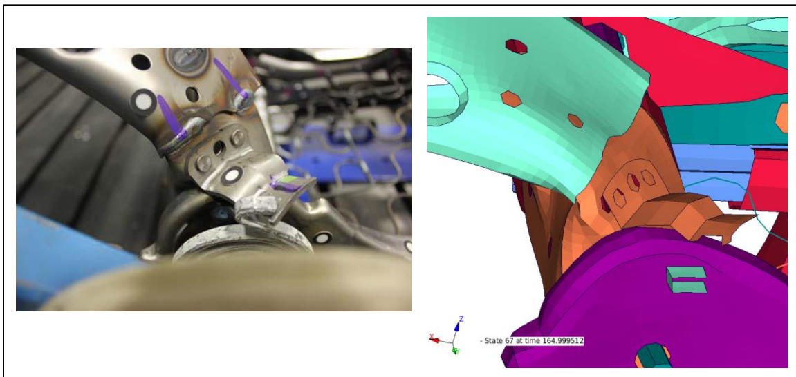
Figure 14: Similar deformation of LHS Seat Frame Test vs FEA – Manual Seat
