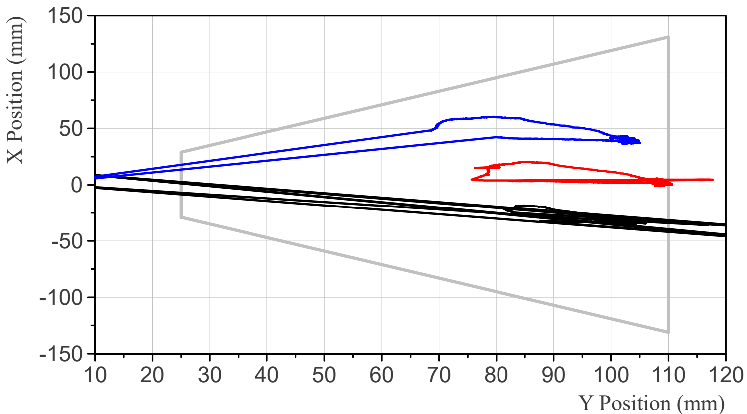
RibEye Measurement Range Plot Thorax Rib 1 Absolute Position, Relative to Thorax Rib 1 Origin
