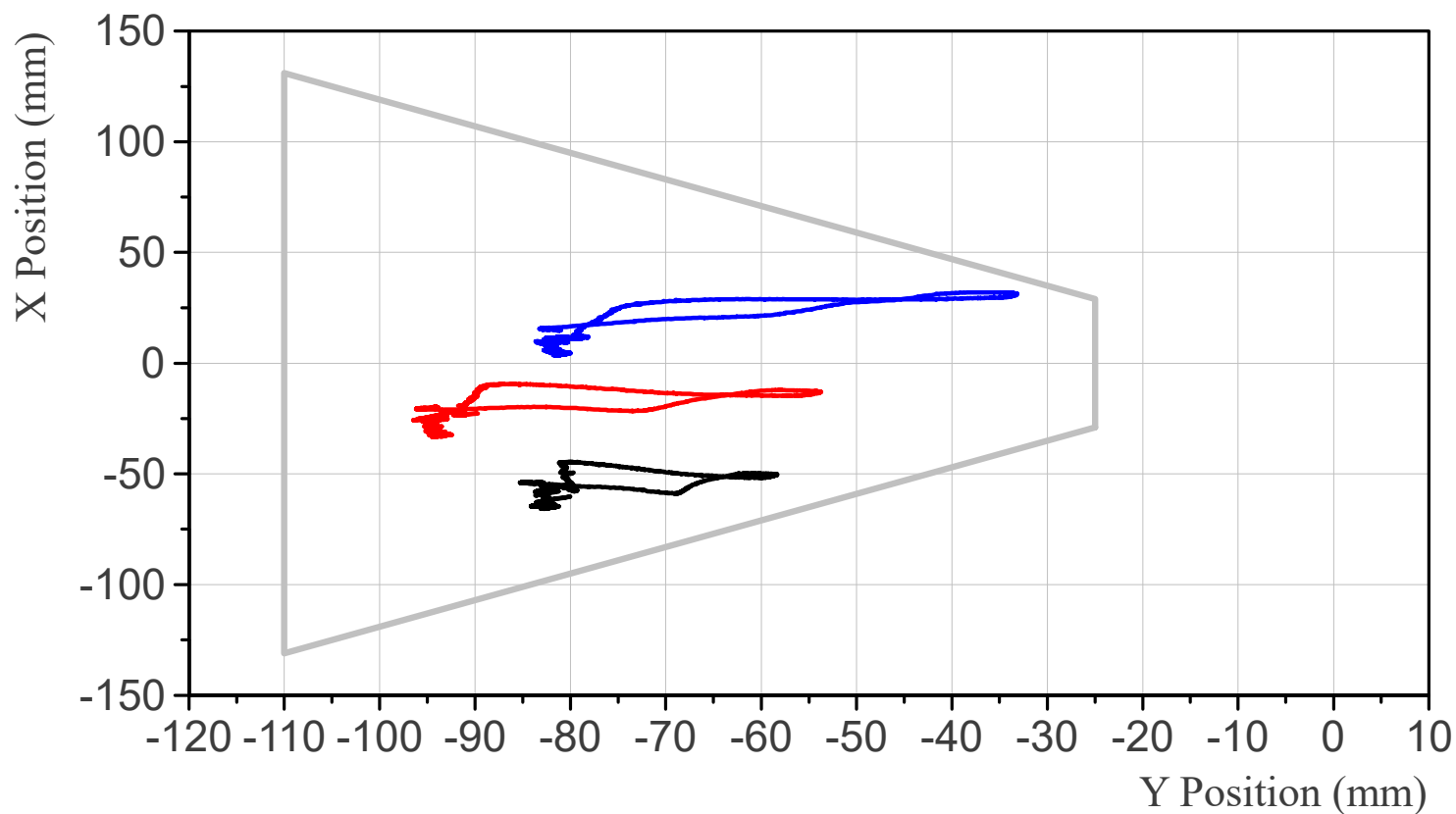
RibEye Measurement Range Plot Shoulder Rib Absolute Position, Relative to Thorax Rib 1 Origin
