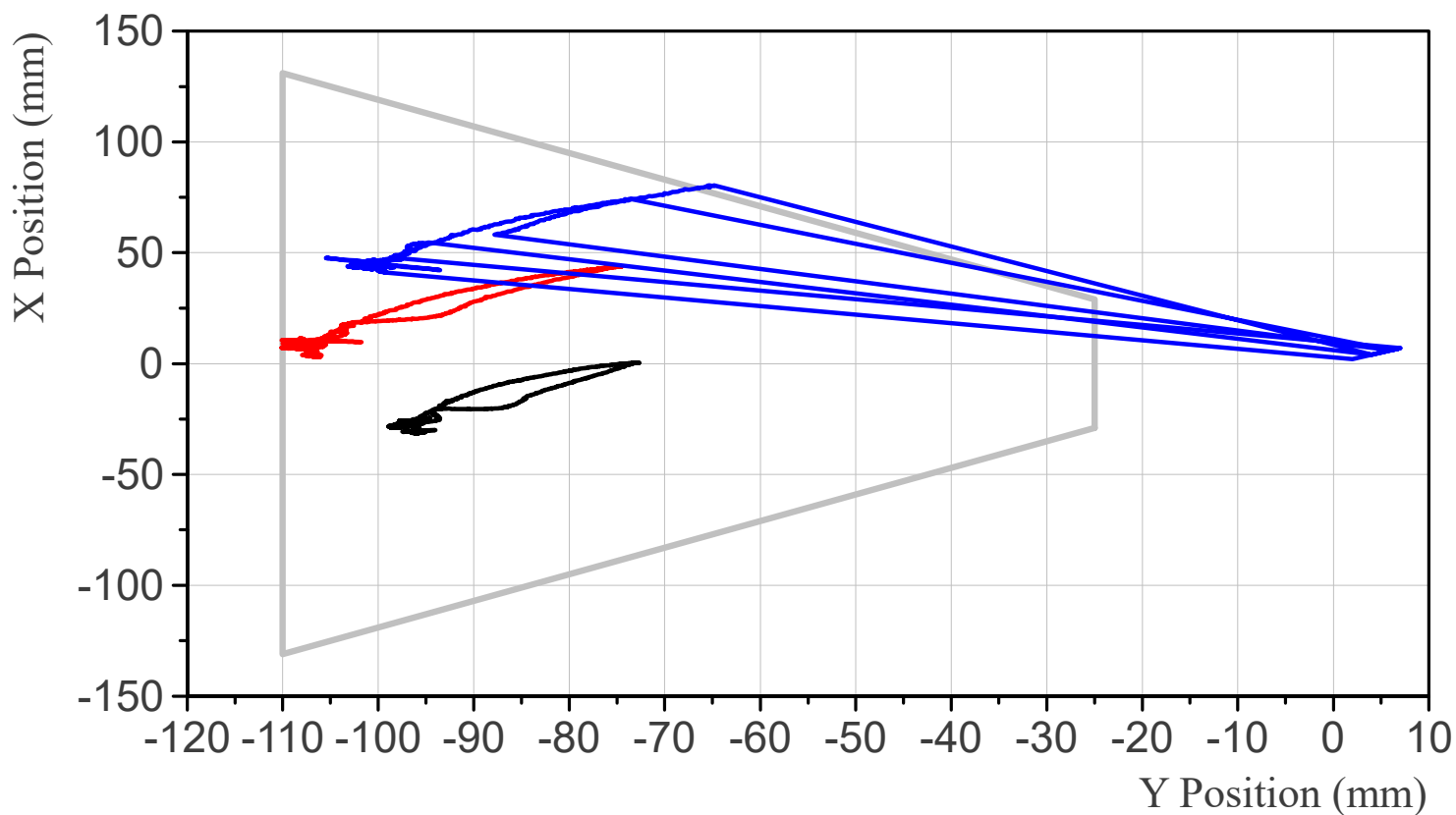
RibEye Measurement Range Plot Thorax Rib 2 Absolute Position, Relative to Thorax Rib 1 Origin
