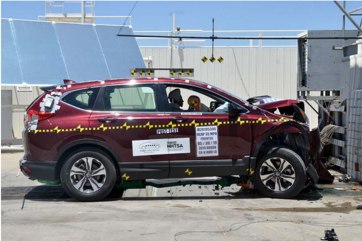
FIGURE 13. Post-Test Right View of Test Vehicle
