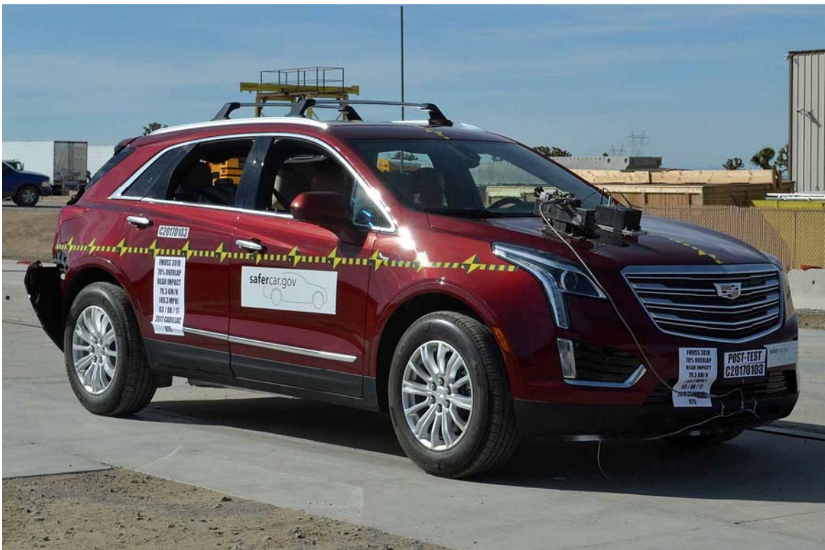
FIGURE 20. Post-Test Right Front \frac{3}{4} View of Test Vehicle
