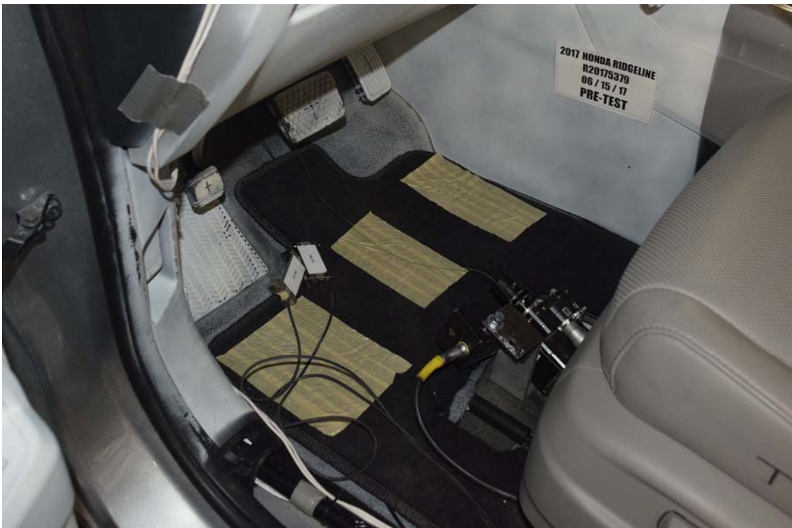
FIGURE 62. Pre-Test View of Driver Floor Pan at Left Sill Level
