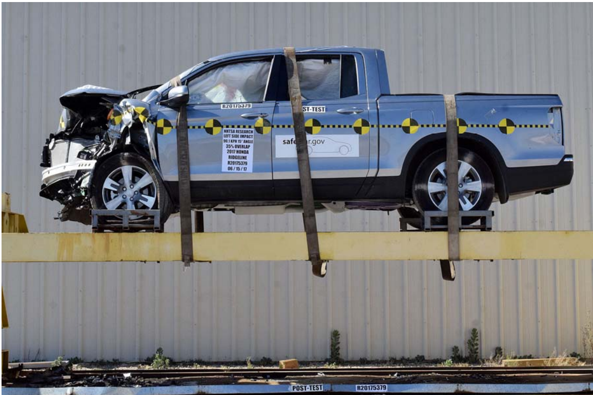
FIGURE 190. Vehicle at 360° on Static Rollover Device
