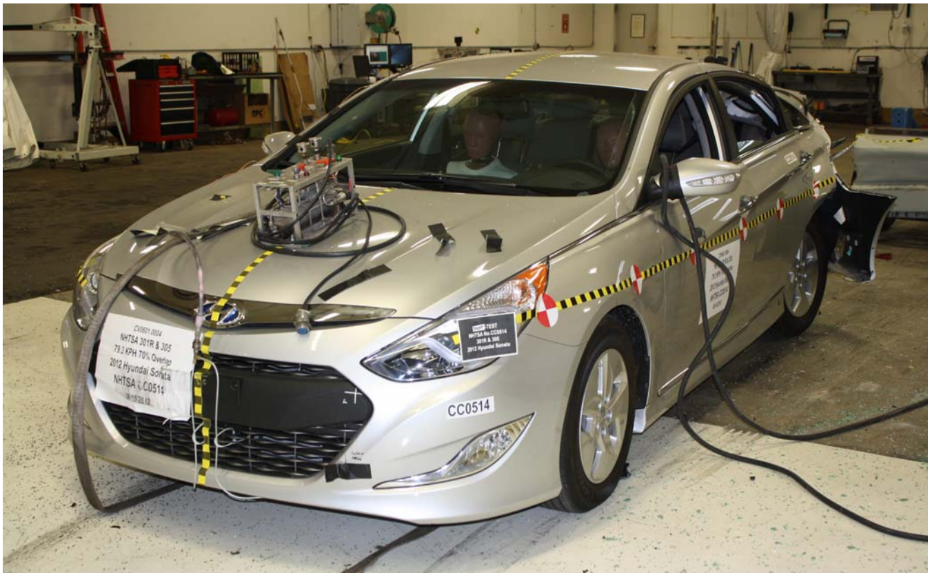
Figure A-12: Post-Test Left Front 3/4 View
