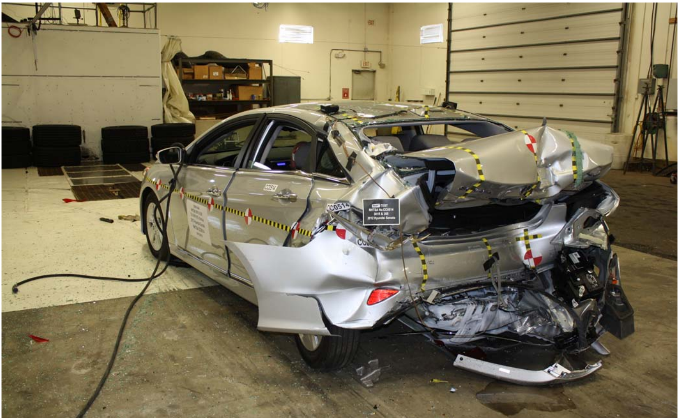
Figure A-16: Post-Test Left Rear 3/4 View
