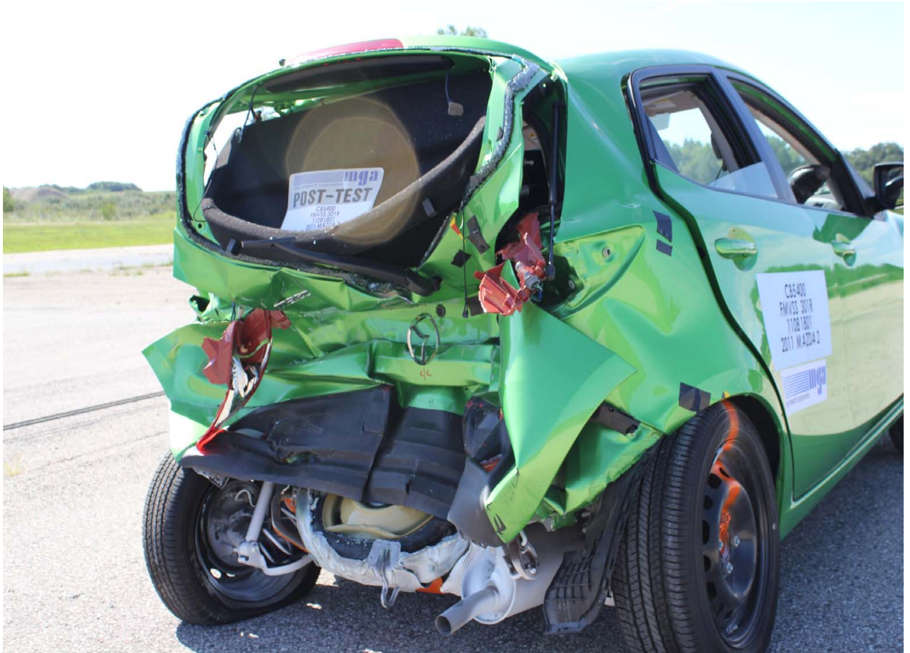
Post-Test Right Rear Close-up View of Vehicle
