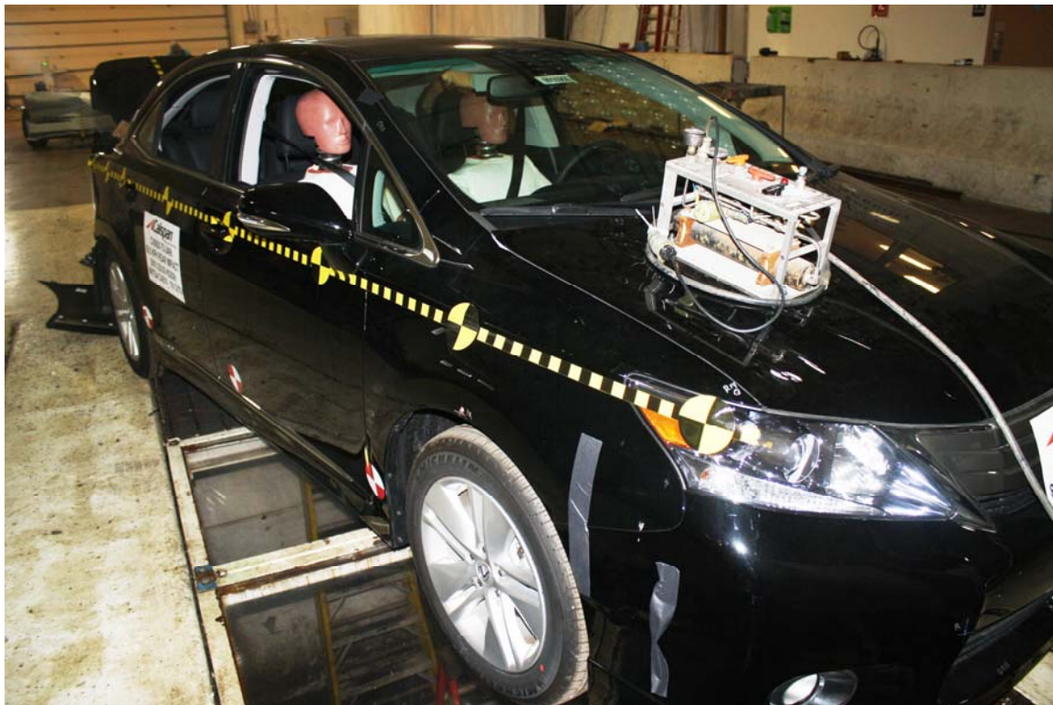
Figure A-12: Post-Test Right Front Three-Quarter View
