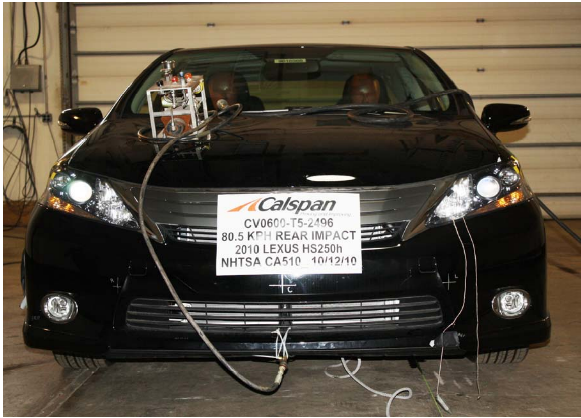
Figure A-3: Pre-Test Front View
