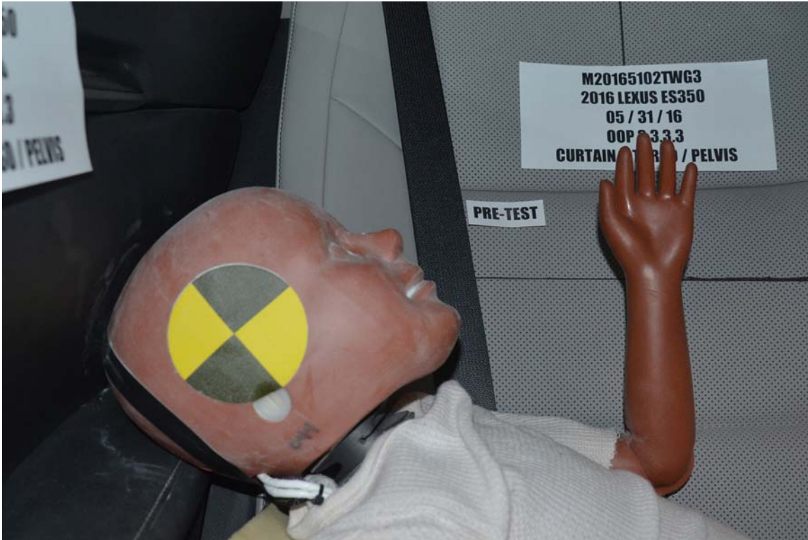
FIGURE 13. Pre-Test Dummy Position, Close-Up Front View
