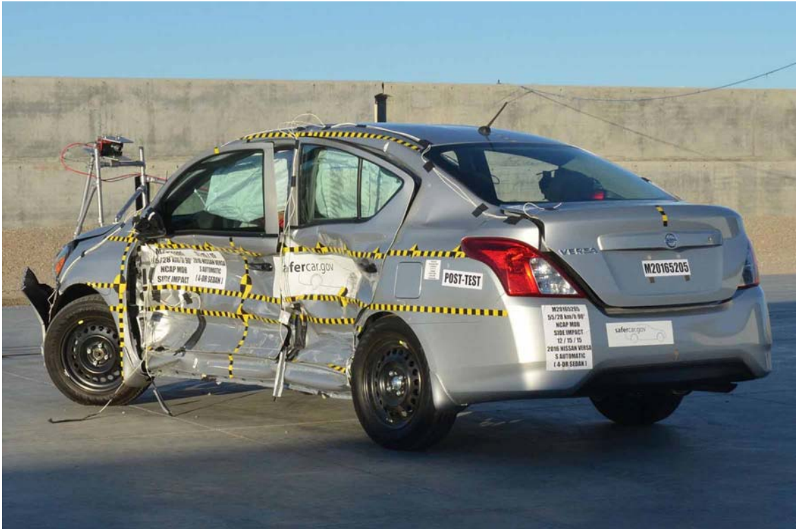
FIGURE 5. Post-Test Left Rear ¾ View of NCAP Side MDB Impact Test
