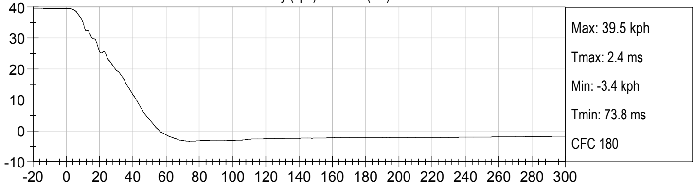
RIGHT REAR SEAT CROSSMEMBER X (G's) vs TIME (ms)
