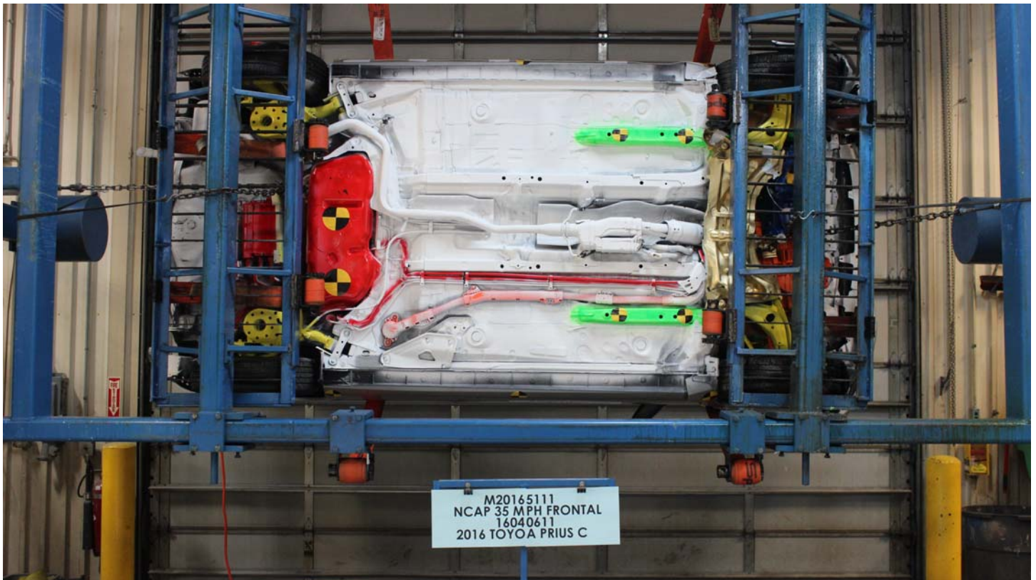
Photo No. 074 - Vehicle at 90 Degrees on Static Rollover Device
