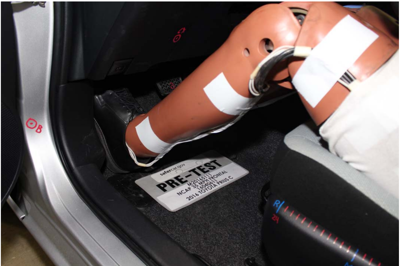
Photo No. 040 - Pre-Test Driver Dummy Feet
