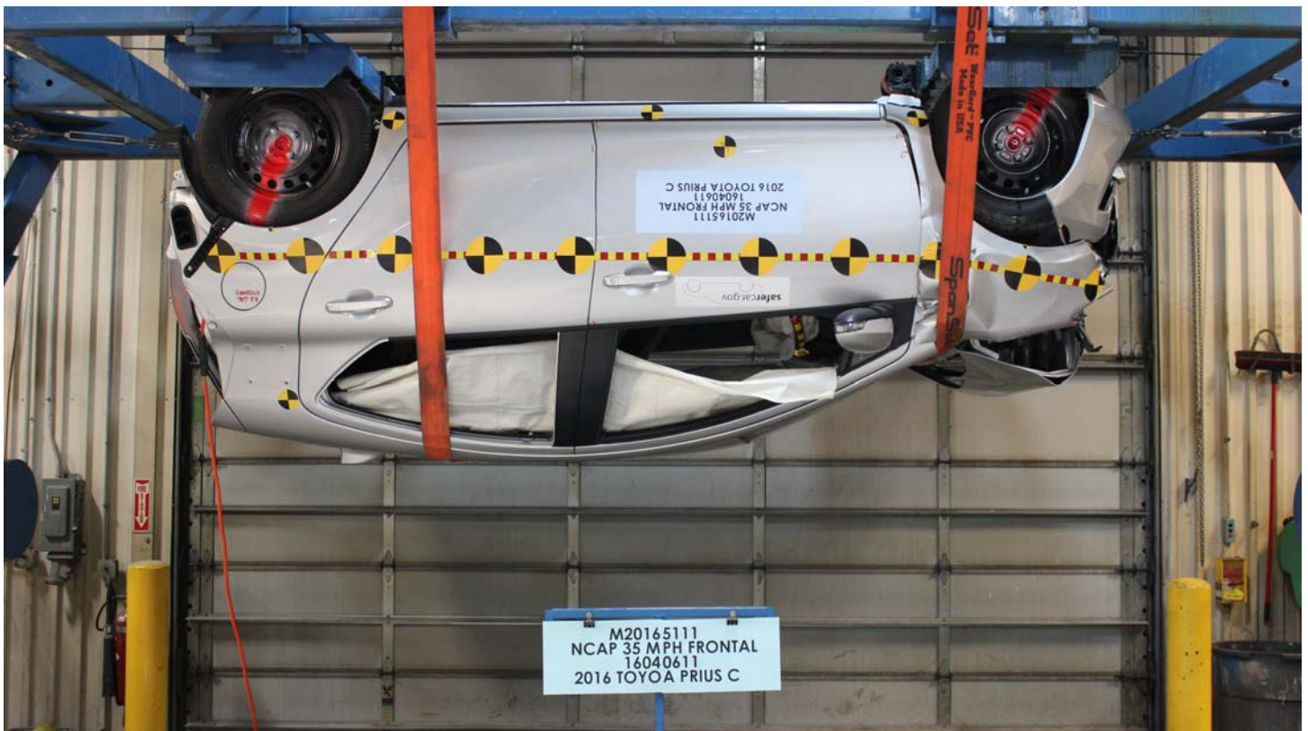
Photo No. 075 - Vehicle at 180 Degrees on Static Rollover Device
