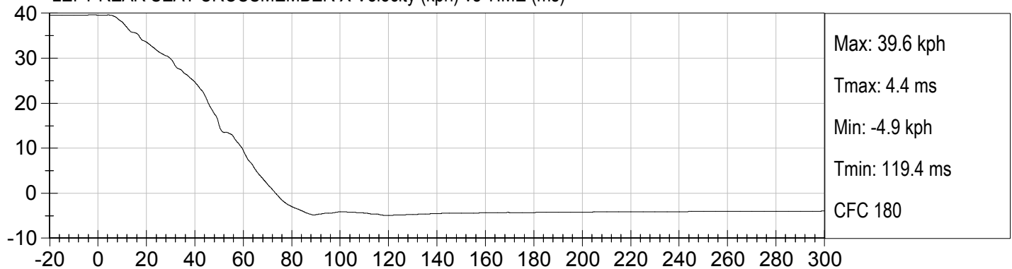
RIGHT REAR SEAT CROSSMEMBER X (G's) vs TIME (ms)
