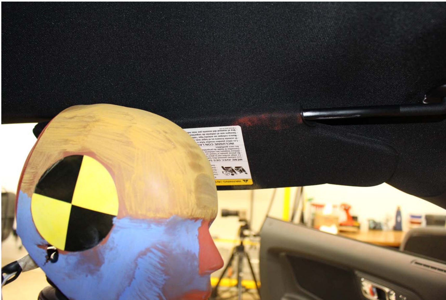
Photo No. 14 - Post-Test 5th Fem. P2 Driver Dummy Head Contact (visor)
