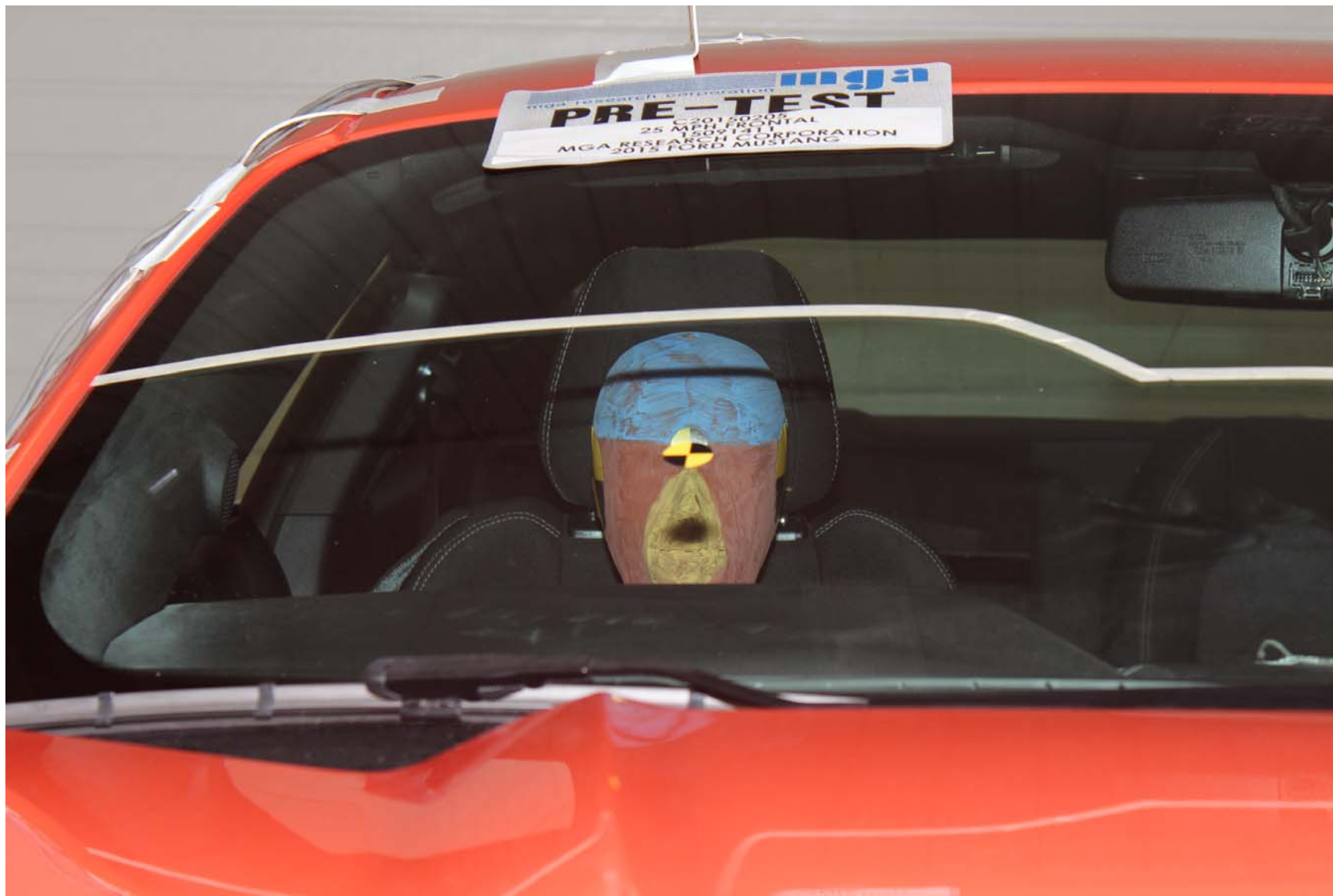
Photo No. 48 - Pre-Test Passenger Dummy Front View (head position)
