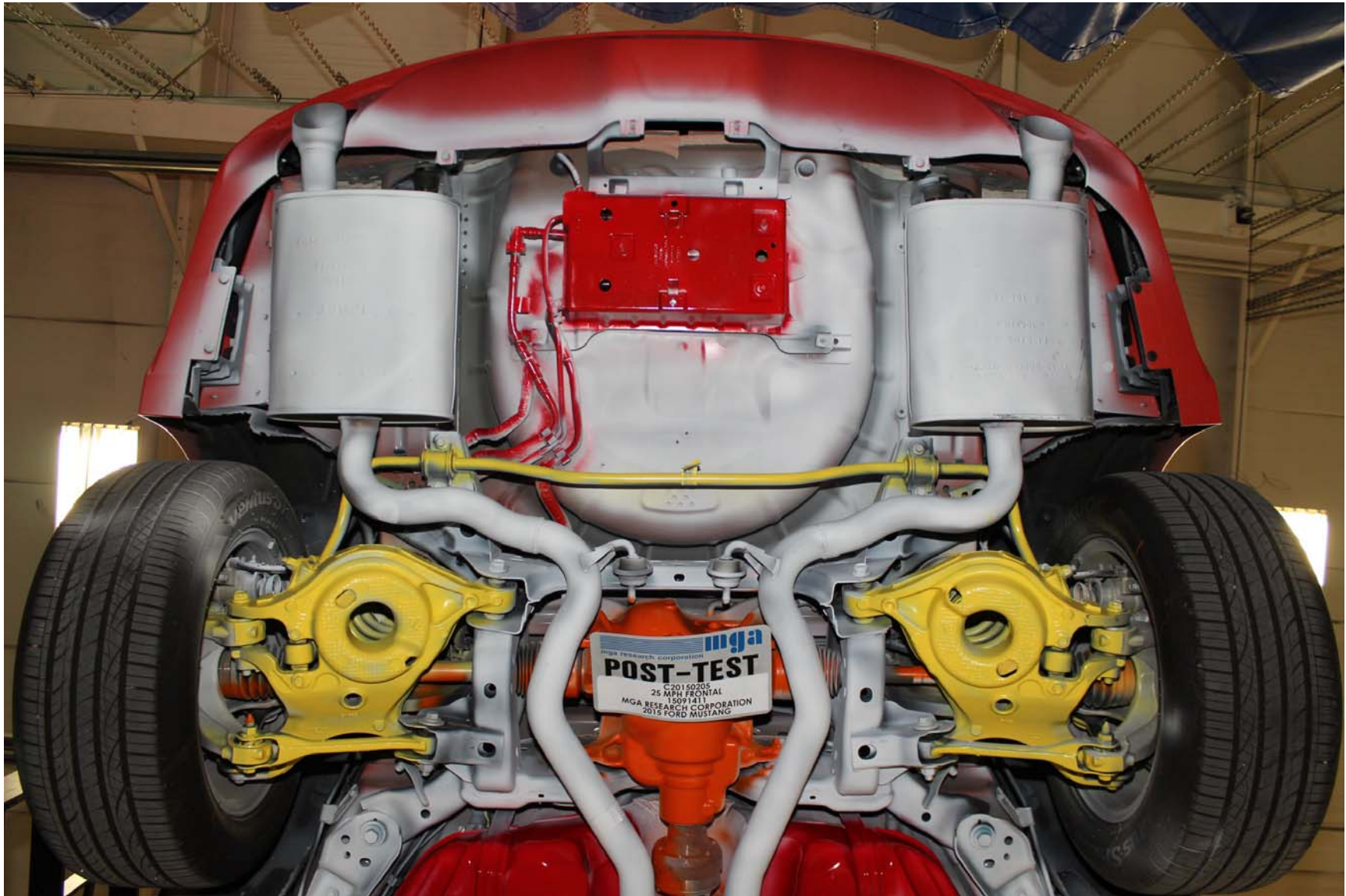
Photo No. 32 - Post-Test Rear Underbody View
