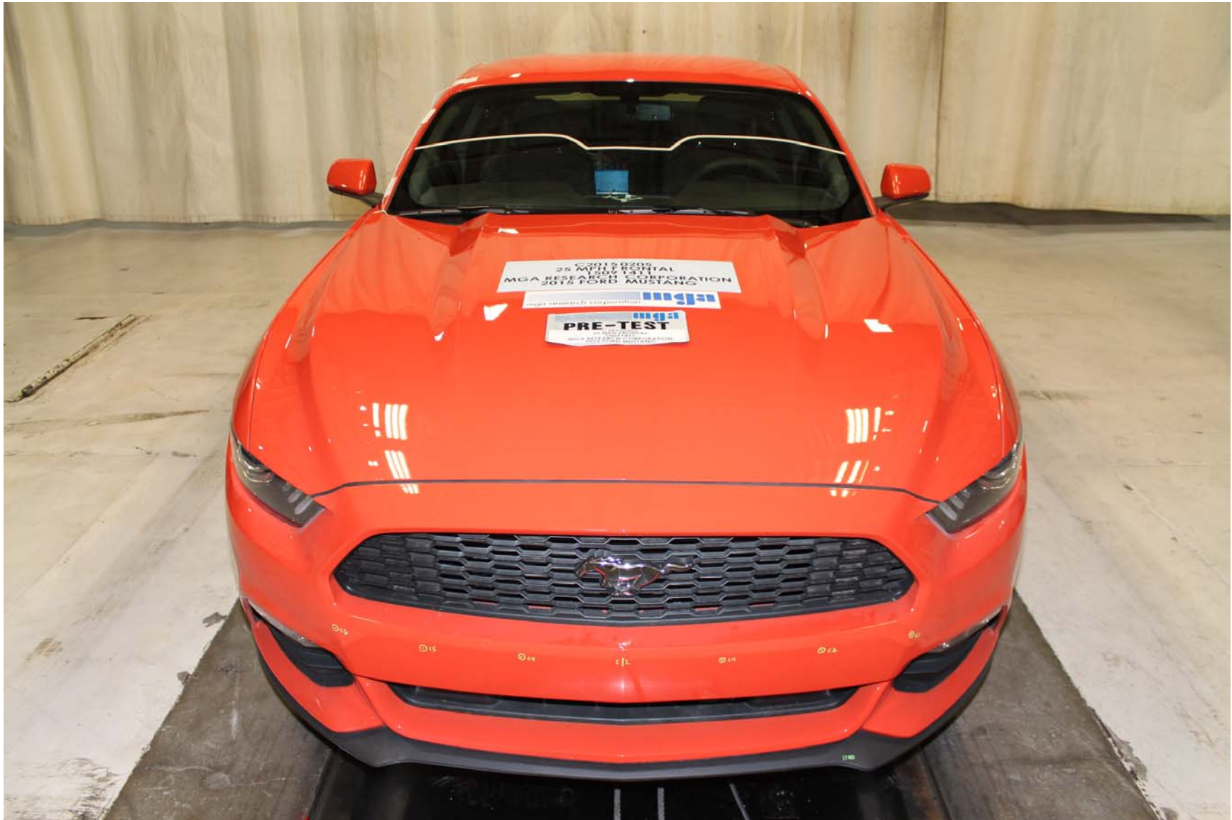
Photo No. 3 - Pre-Test Front View of Test Vehicle
