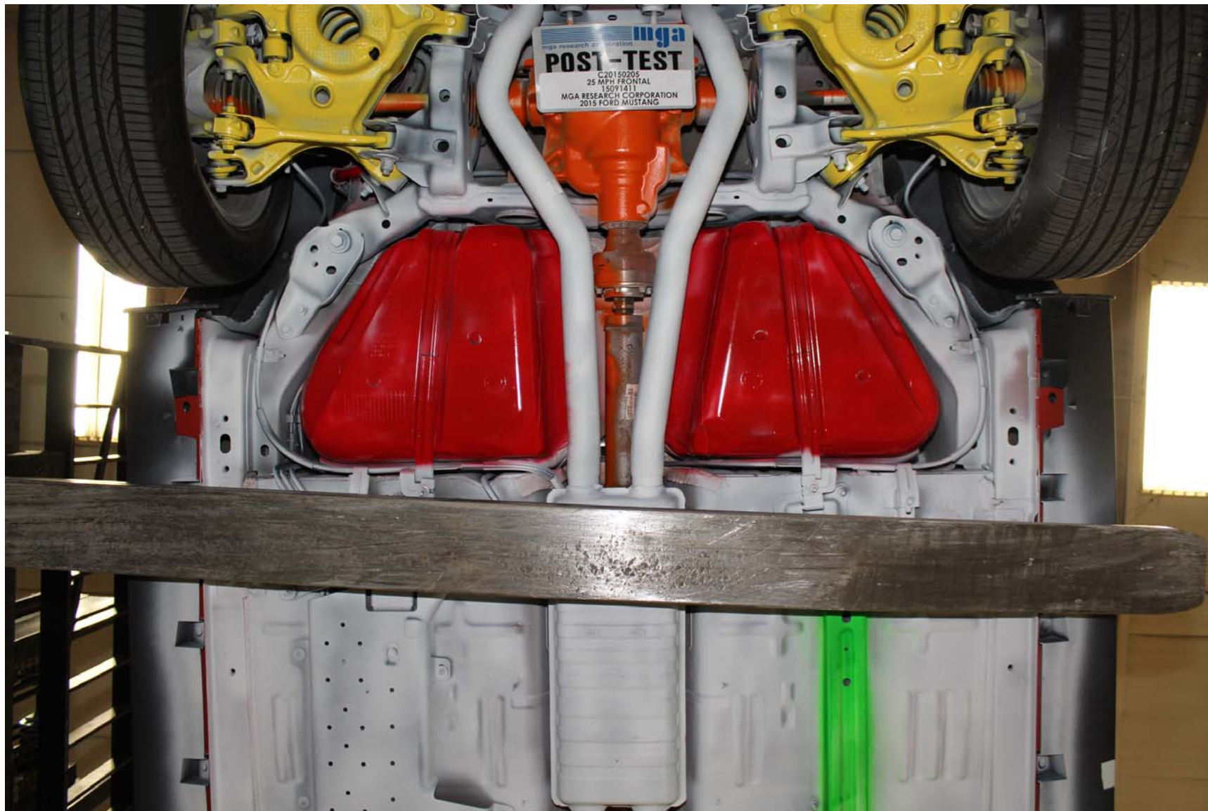
Photo No. 30 - Post-Test Mid Rear Underbody View
