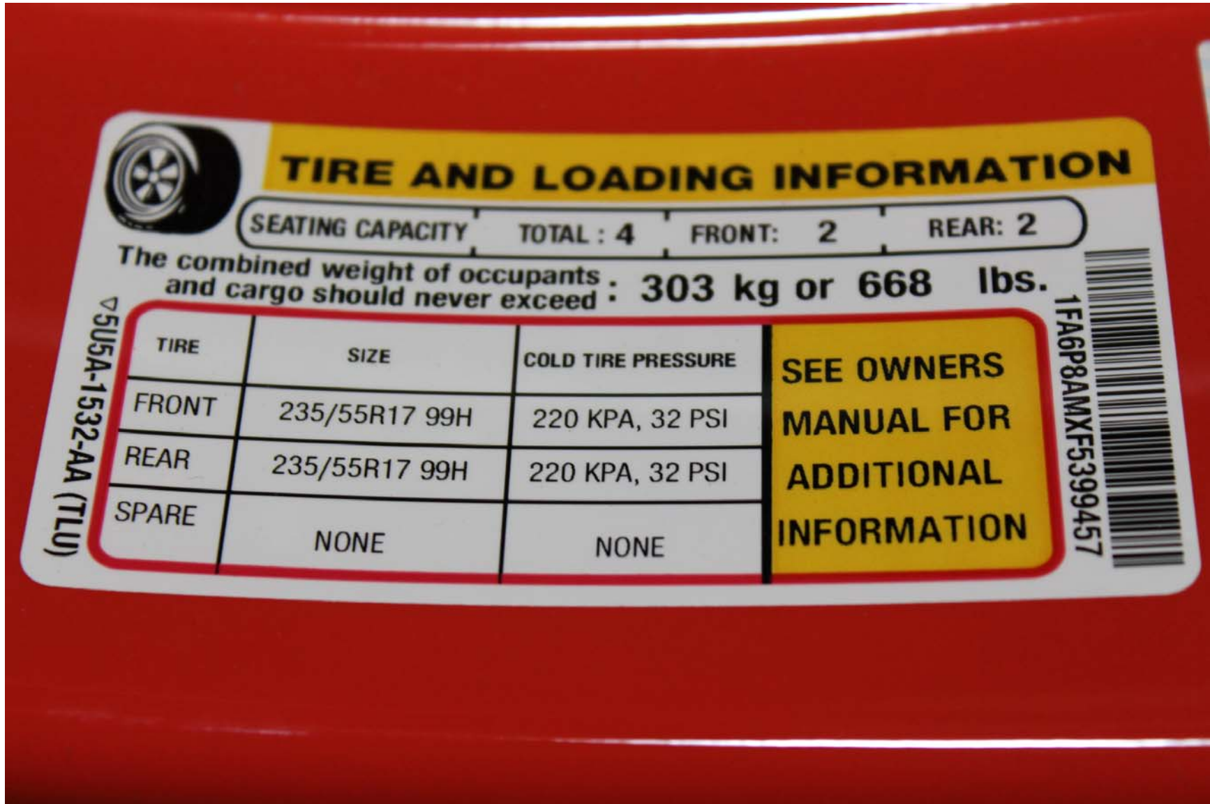
Photo No. 2 - Tire Placard
