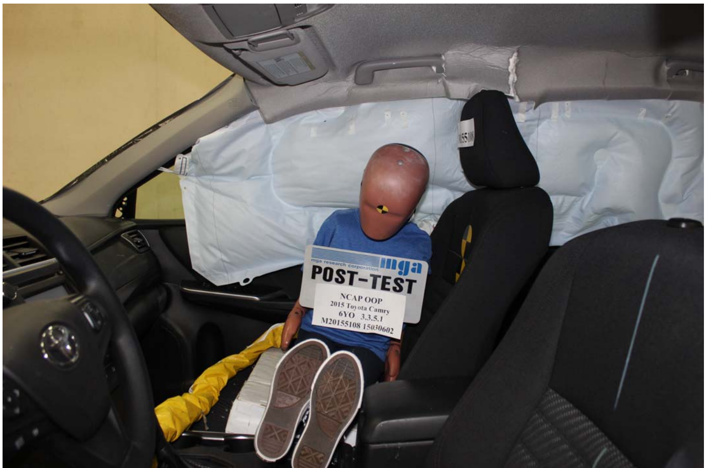
Photo No. 6 - Post-Test 6-Year-Old Child Dummy Left Side View
