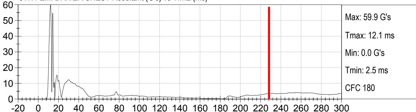
5TH FEM. DRIVER CHEST Resultant (G's) vs TIME (ms)
