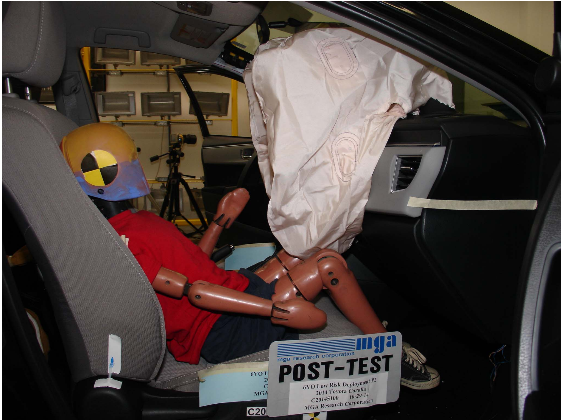
Photo No. 37 - Post-Test 6YO P2 Passenger Dummy Right Side View
