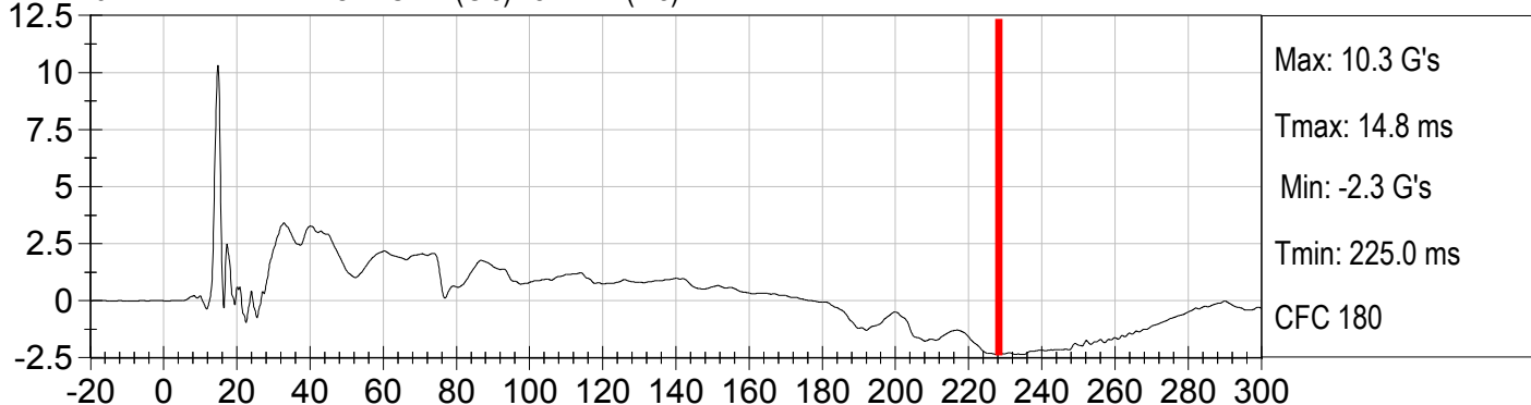
5TH FEM. DRIVER CHEST Resultant (G's) vs TIME (ms)
