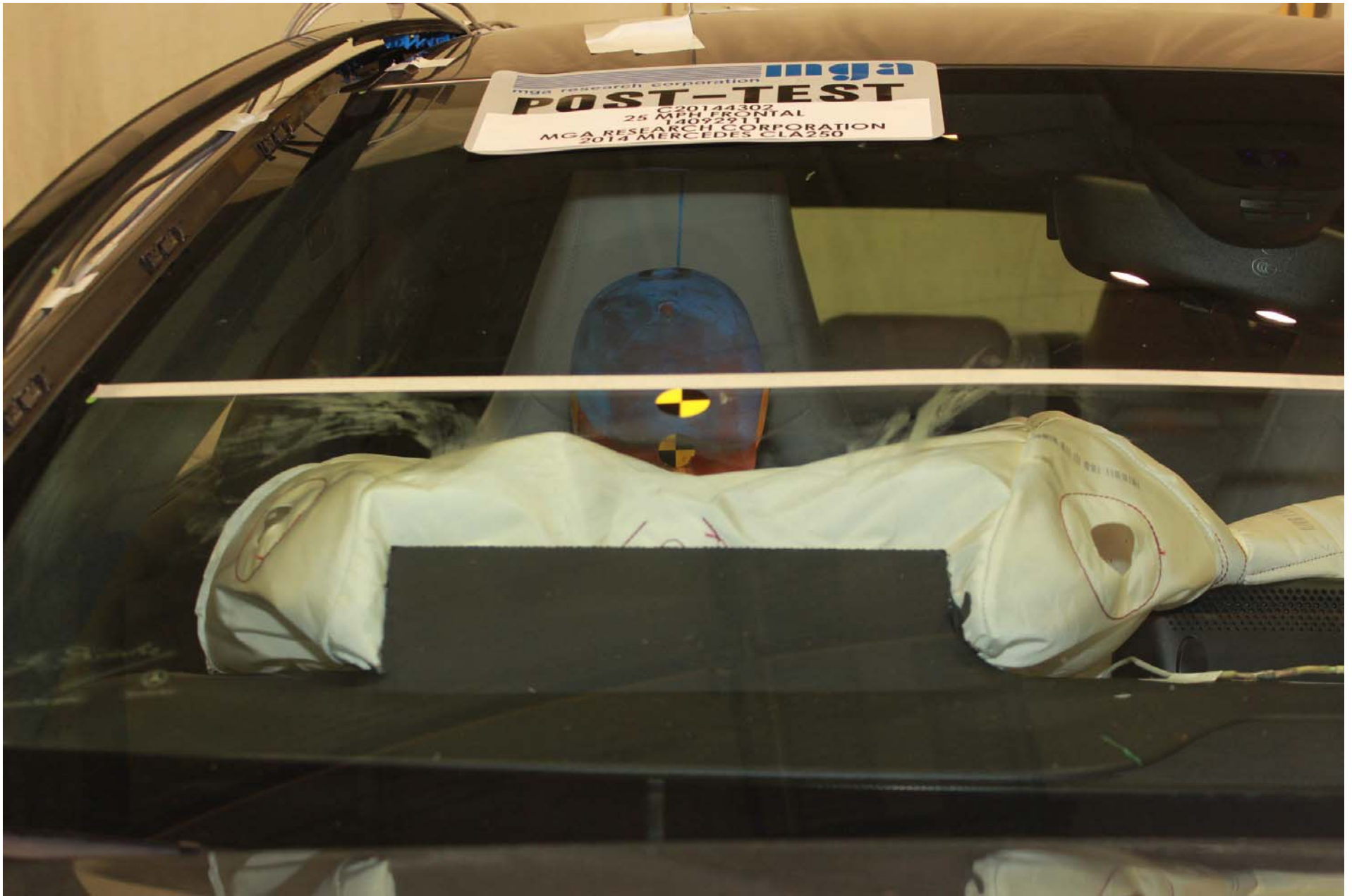
Photo No. 50 - Post-Test Passenger Dummy Front View (head position)
