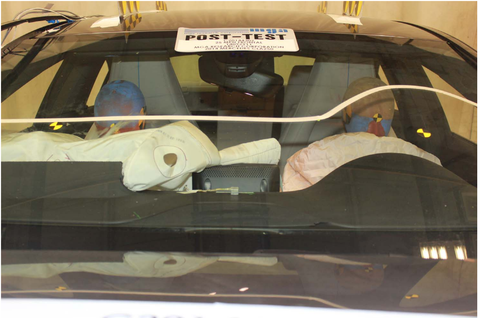
Photo No. 20 - Post-Test Windshield View
