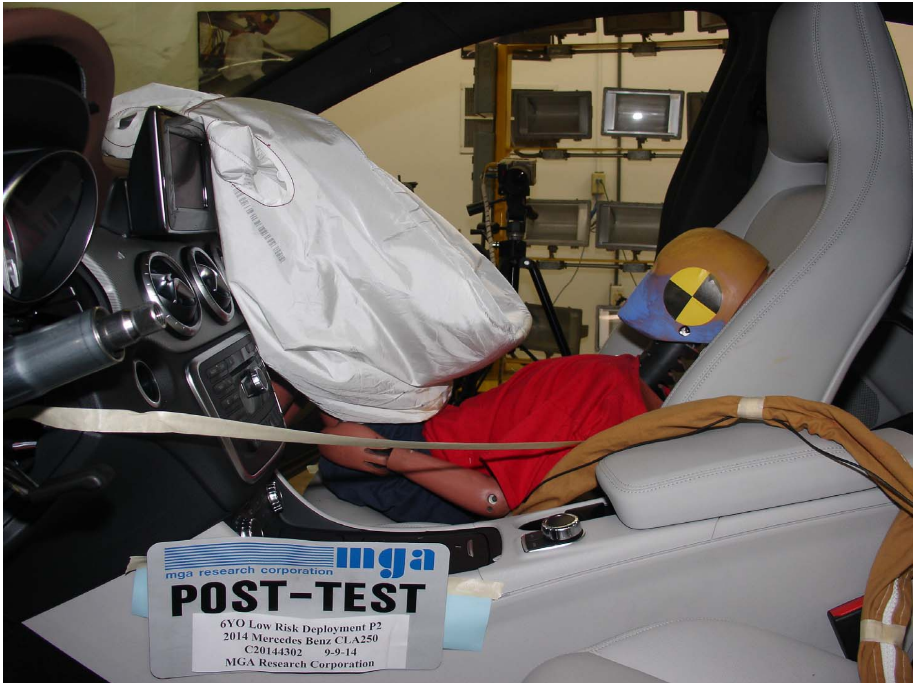
Photo No. 34 - Post-Test 6YO P2 Passenger Dummy Left Side View
