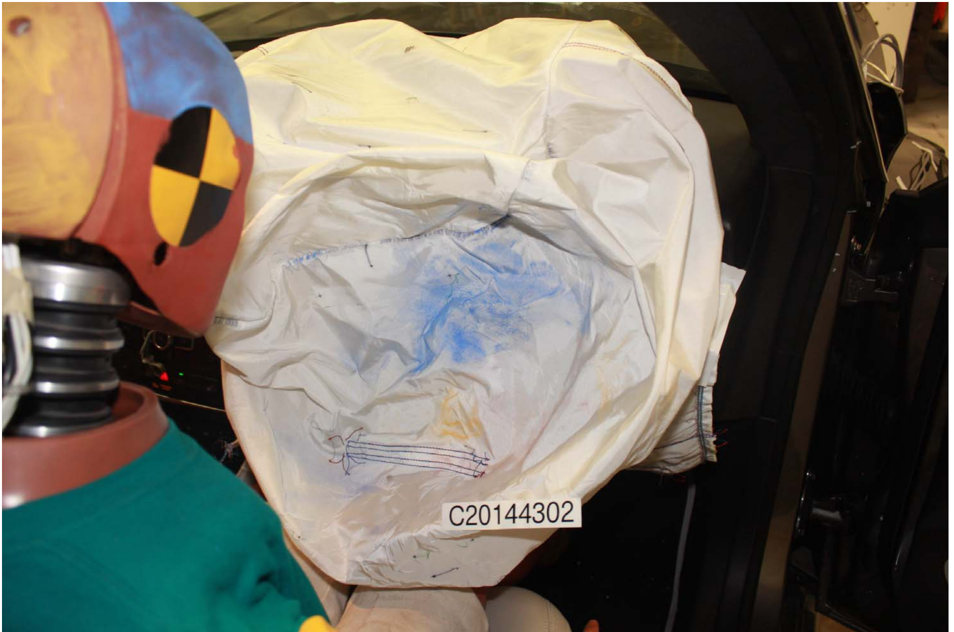
Photo No. 61 - Post-Test Passenger Dummy Airbag Contact
