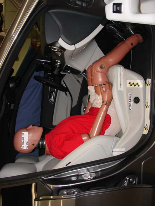
Unbelted 5th Percentile Female Dummy Reactivation, Forward Seat Track
