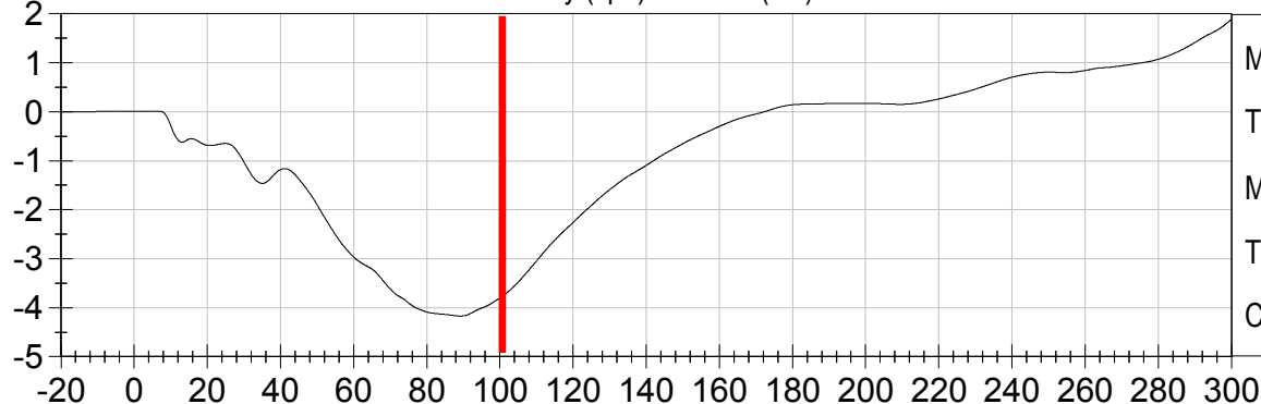
6YR OLD PASSENGER CHEST X Velocity (kph) vs TIME (ms)
