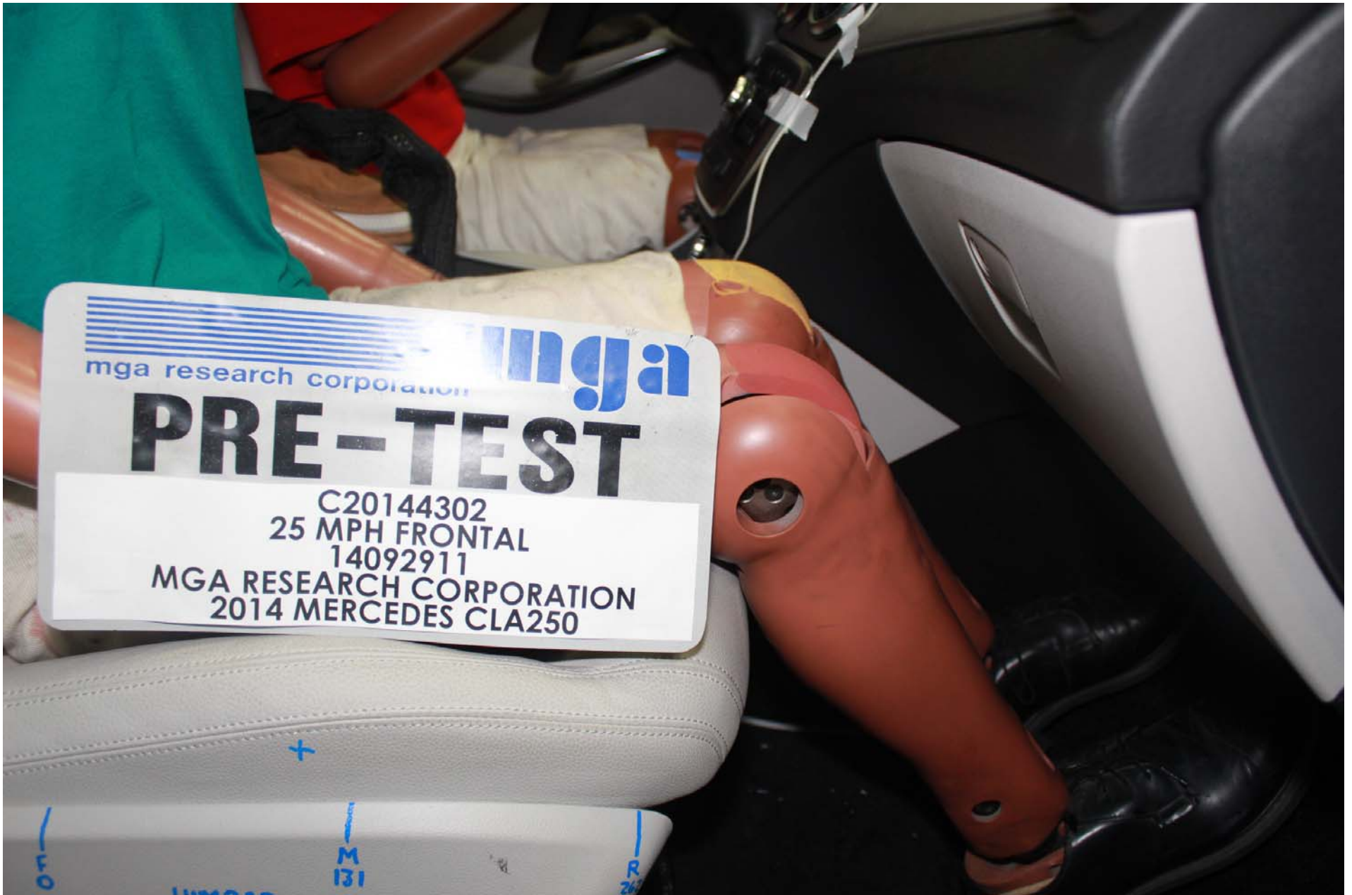
Photo No. 59 - Pre-Test Passenger Side Knee Bolster View
