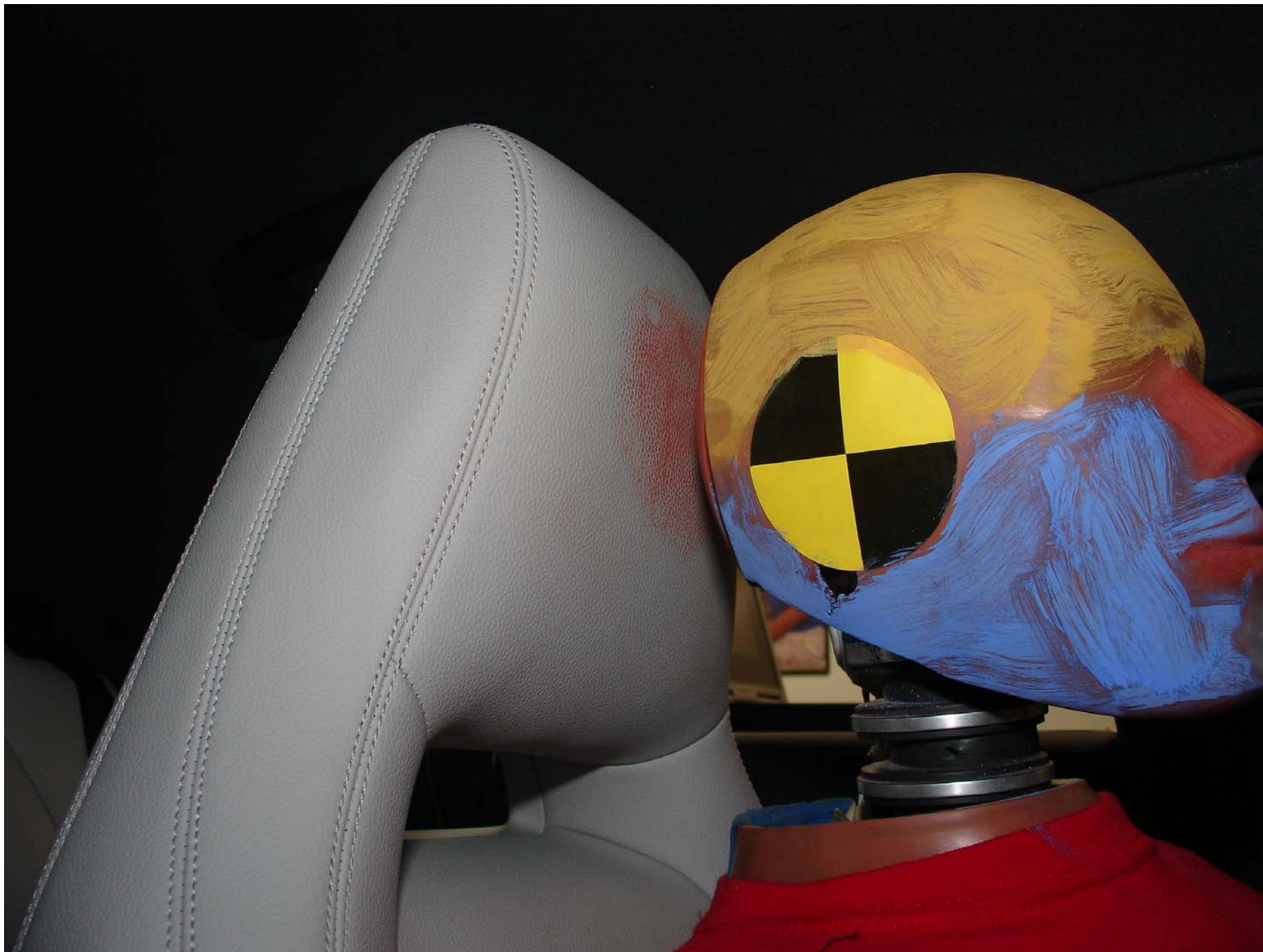
Photo No. 15 - Post-Test 5th Fem. P2 Driver Dummy Head Contact (headrest)
