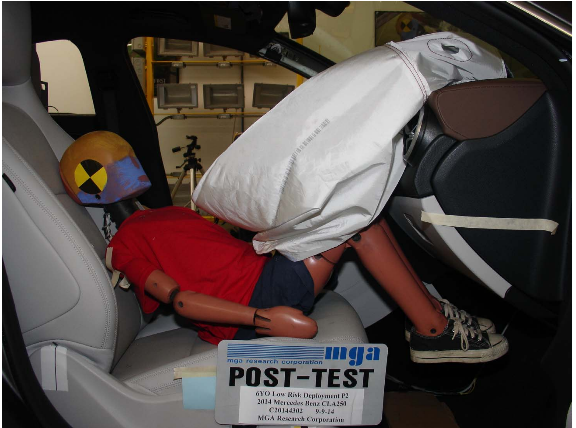
Photo No. 36 - Post-Test 6YO P2 Passenger Dummy Right Side View
