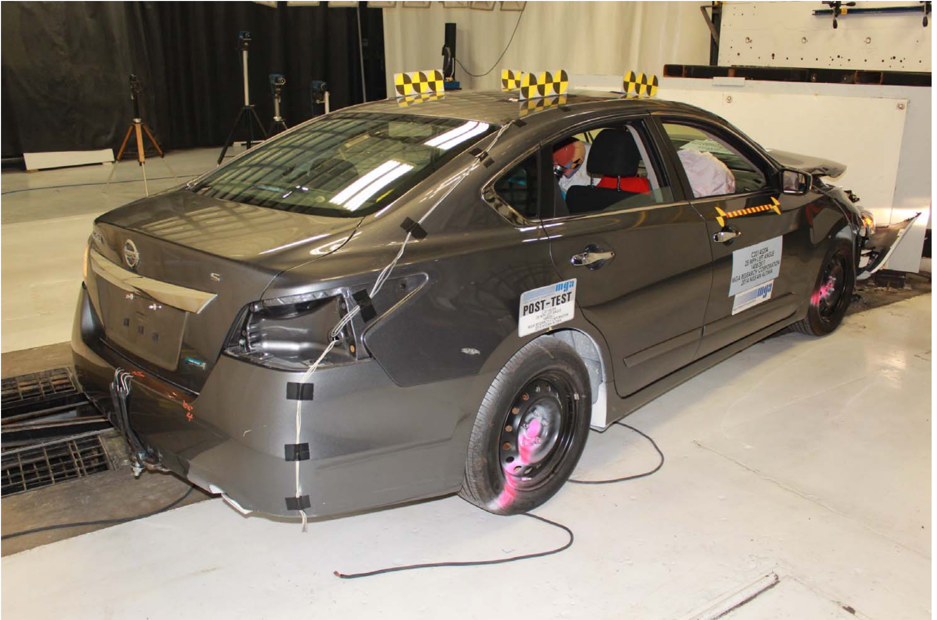
Photo No. 14 - Post-Test Right Rear Three-Quarter View of Test Vehicle
