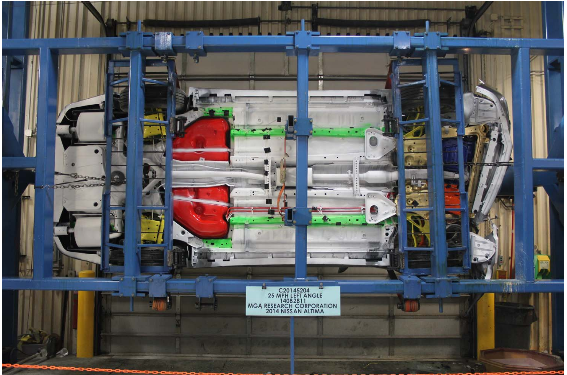
Photo No. 66 - Rollover 90 Degrees
