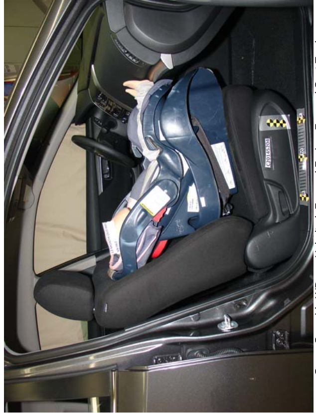
Graco Snuggly WBBase, Unbelted, Forward Facing, Forward Seat Track
