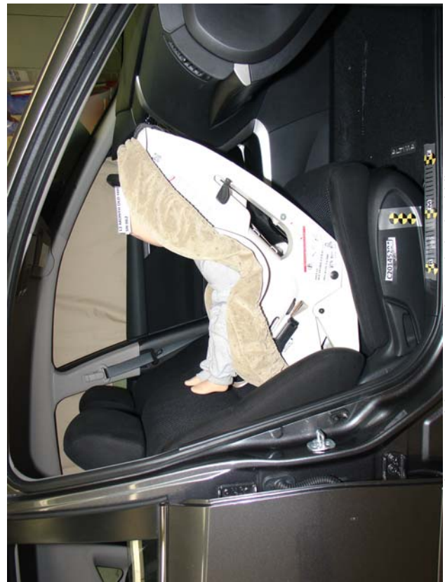
Britax Roundabout Rear Facing, Belted, Rearward Seat Track
