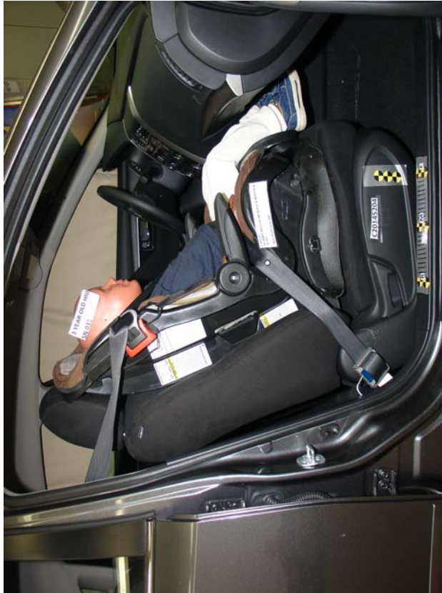
3-Year-Old Cosco Summit Deluxe Belted, Forward Seat Track
