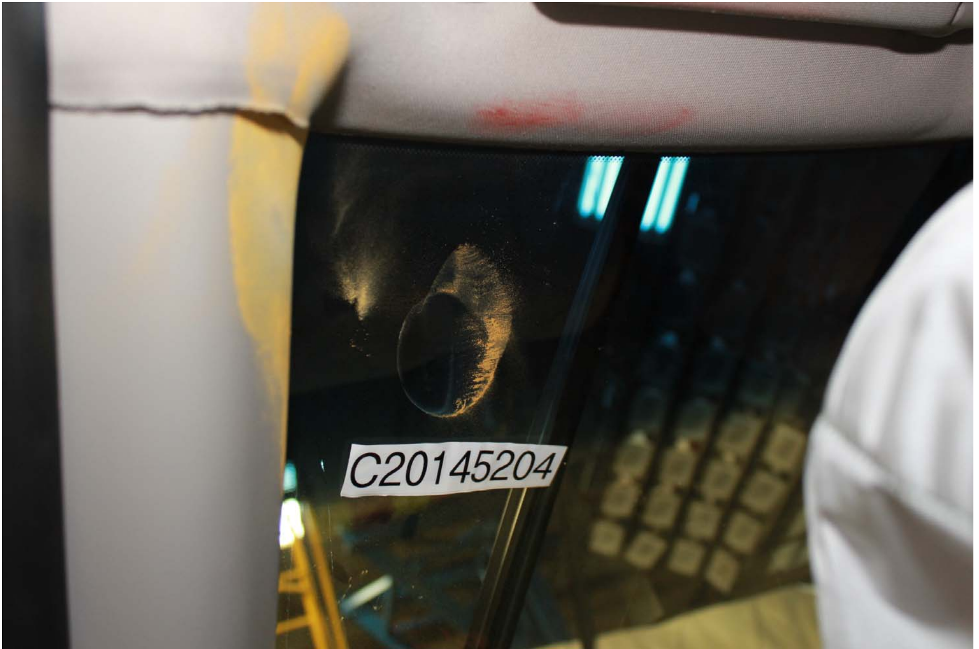
Photo No. 48 - Post-Test Driver Dummy Head Contact (windshield)
