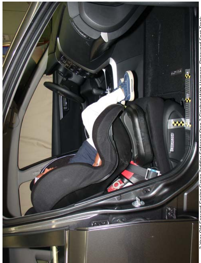
3-Year-Old Forward Facing Graco Toddler Safeseat Step 2 Cinched With Harness, Rearward Seat Track
