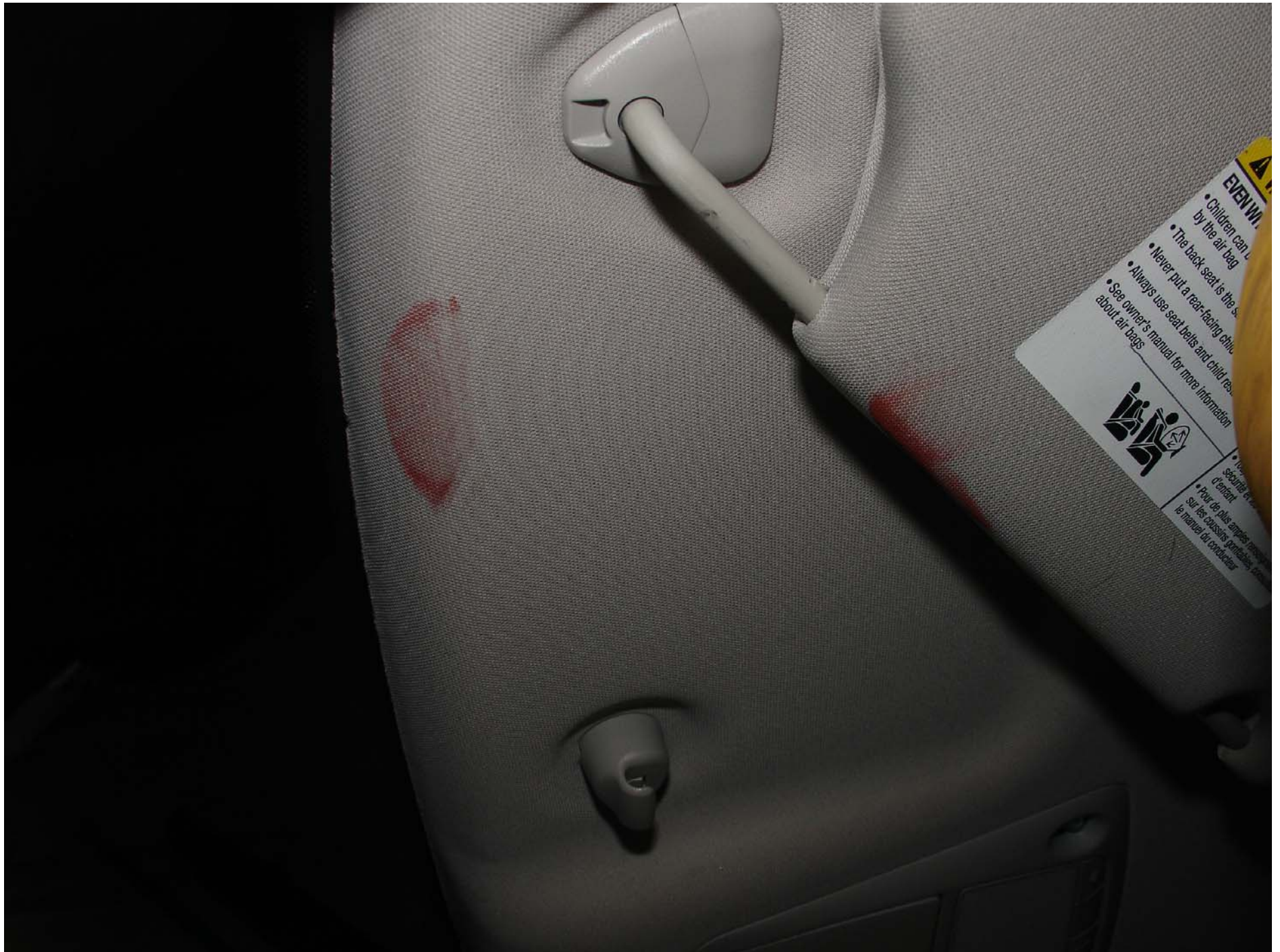
Photo No. 15 - Pot-Test 5th Fem. P2 Driver Dummy Head Contact (headliner-visor)
