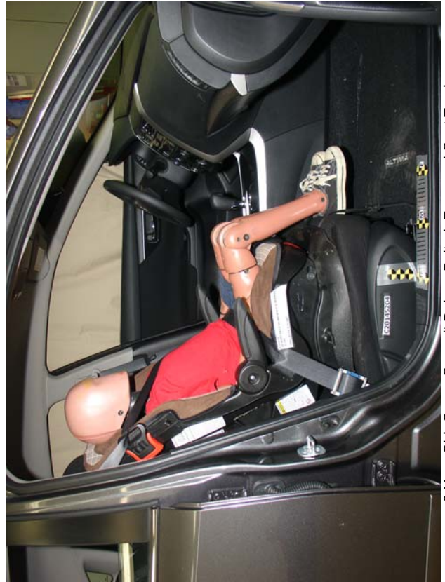
6-Year-Old Cosco Summit Deluxe Belted, Rearward Seat Track
