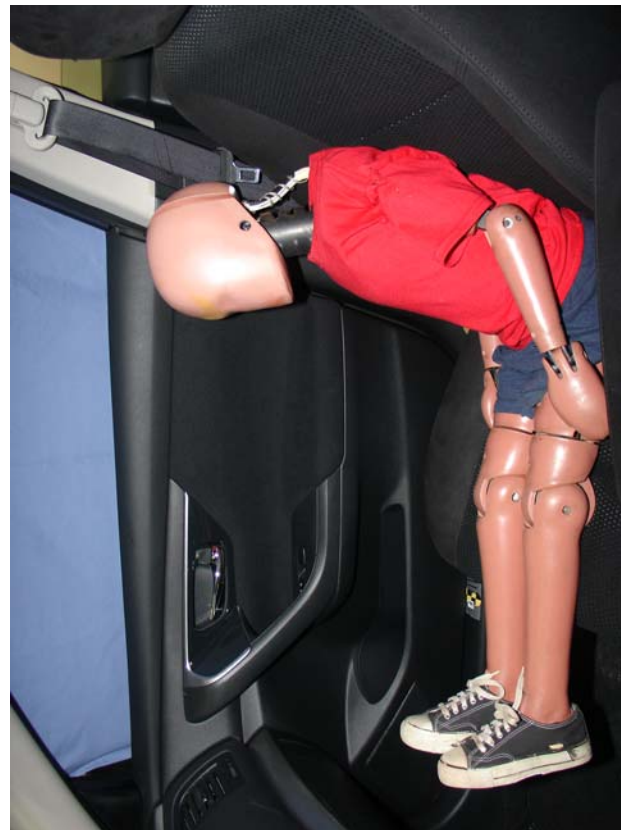
6-Year-Old Unbelted, Rearward Seat Track Position 4
