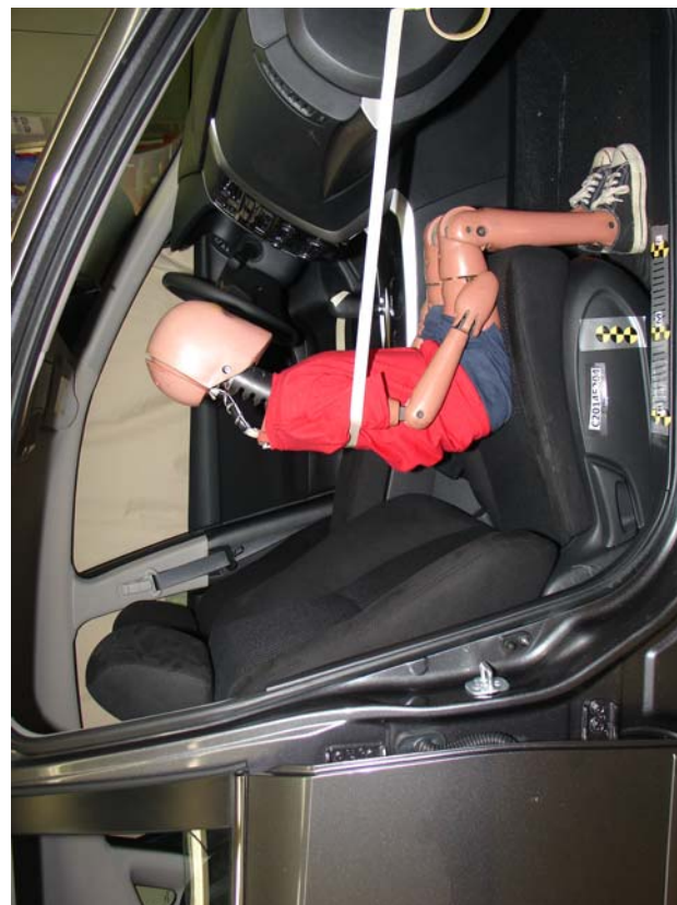
6-Year-Old Unbelted, Middle Seat Track Position 3
