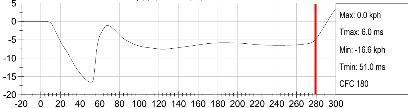
5TH FEM. DRIVER HEAD X Velocity (kph) vs TIME (ms)
