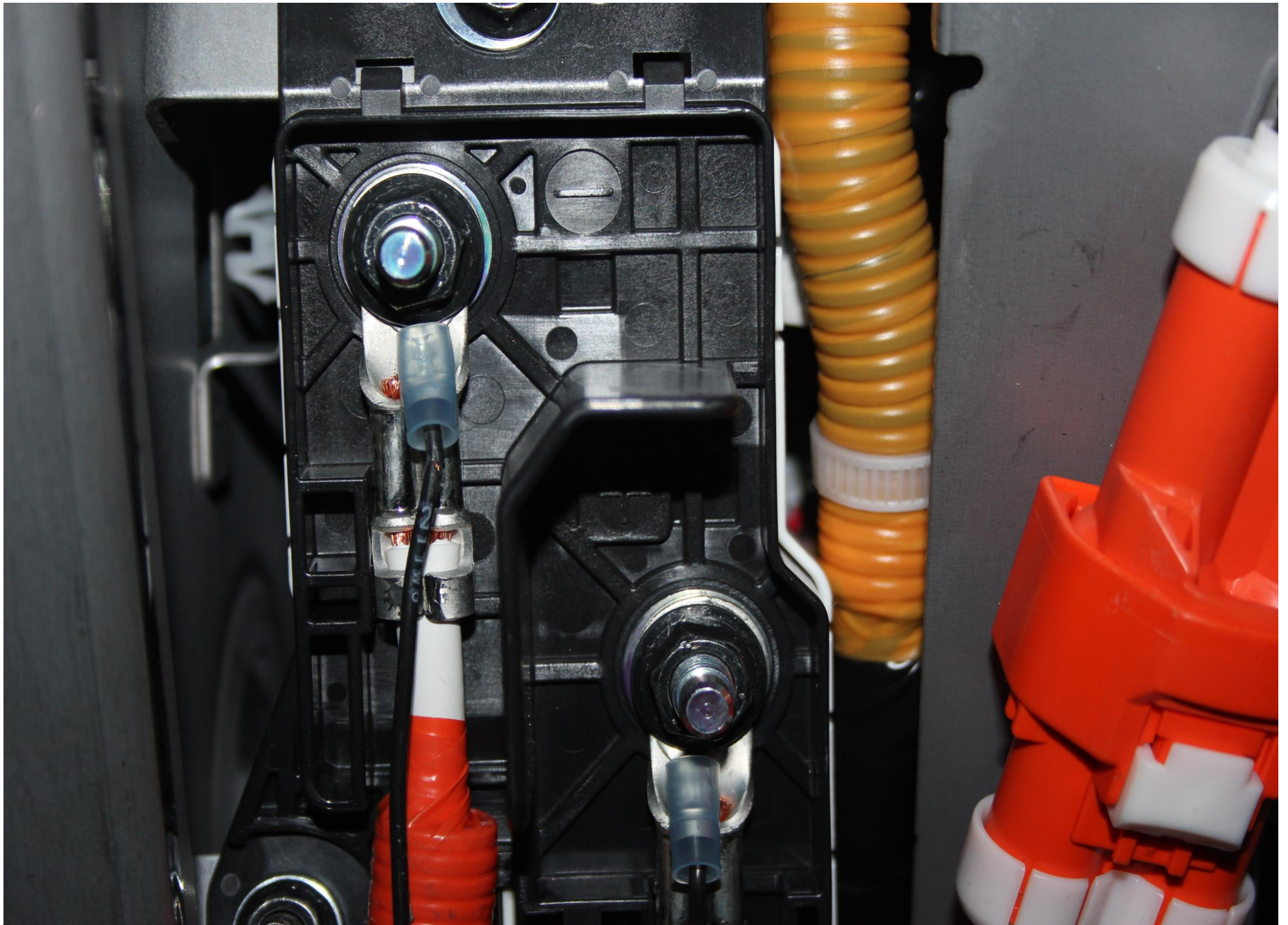
Pre-Test Positive and Negative Attachment Point to the Propulsion Battery System
