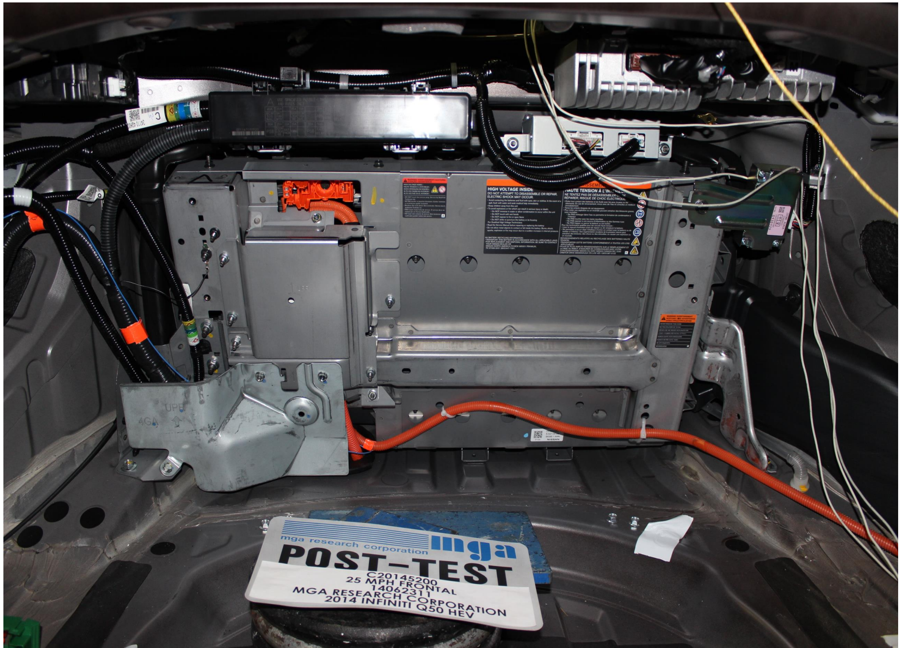
Post-Test View of Vehicle's Passenger Compartment Adjacent to Electric Energy Storage Conversion System Rear View
