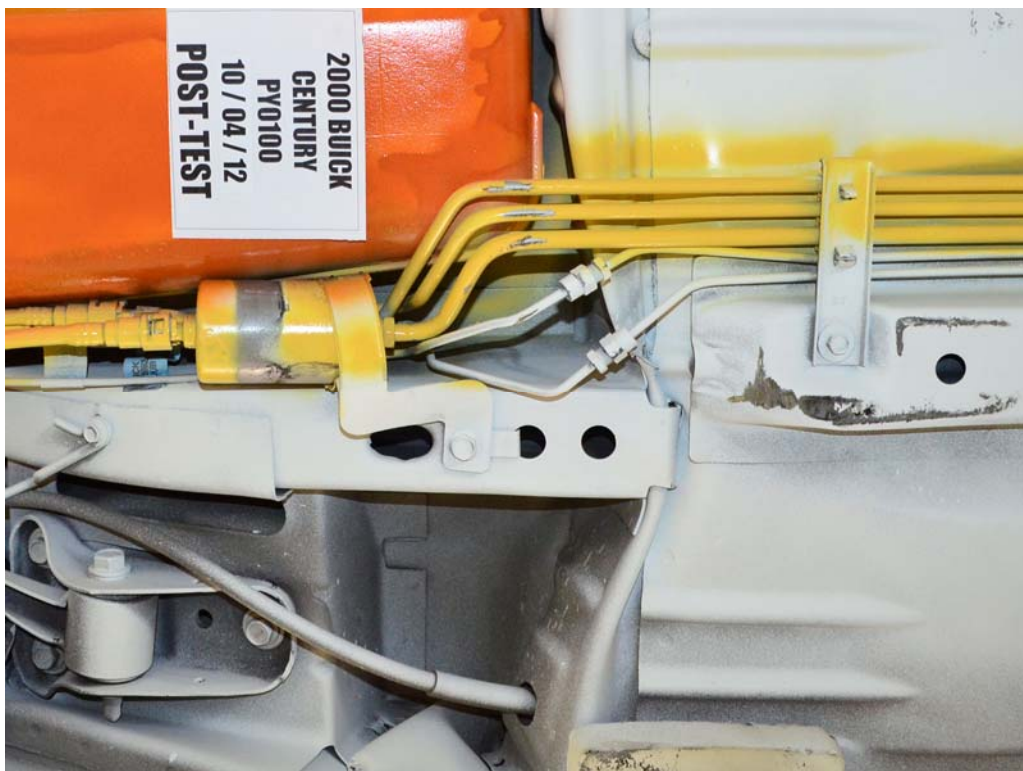
FIGURE 24. Post-Test Underbody, Fuel Line Location
