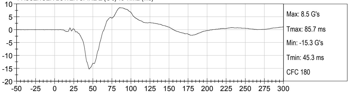
PASSENGER LOWER SPINE Resultant (G's) vs TIME (ms)
