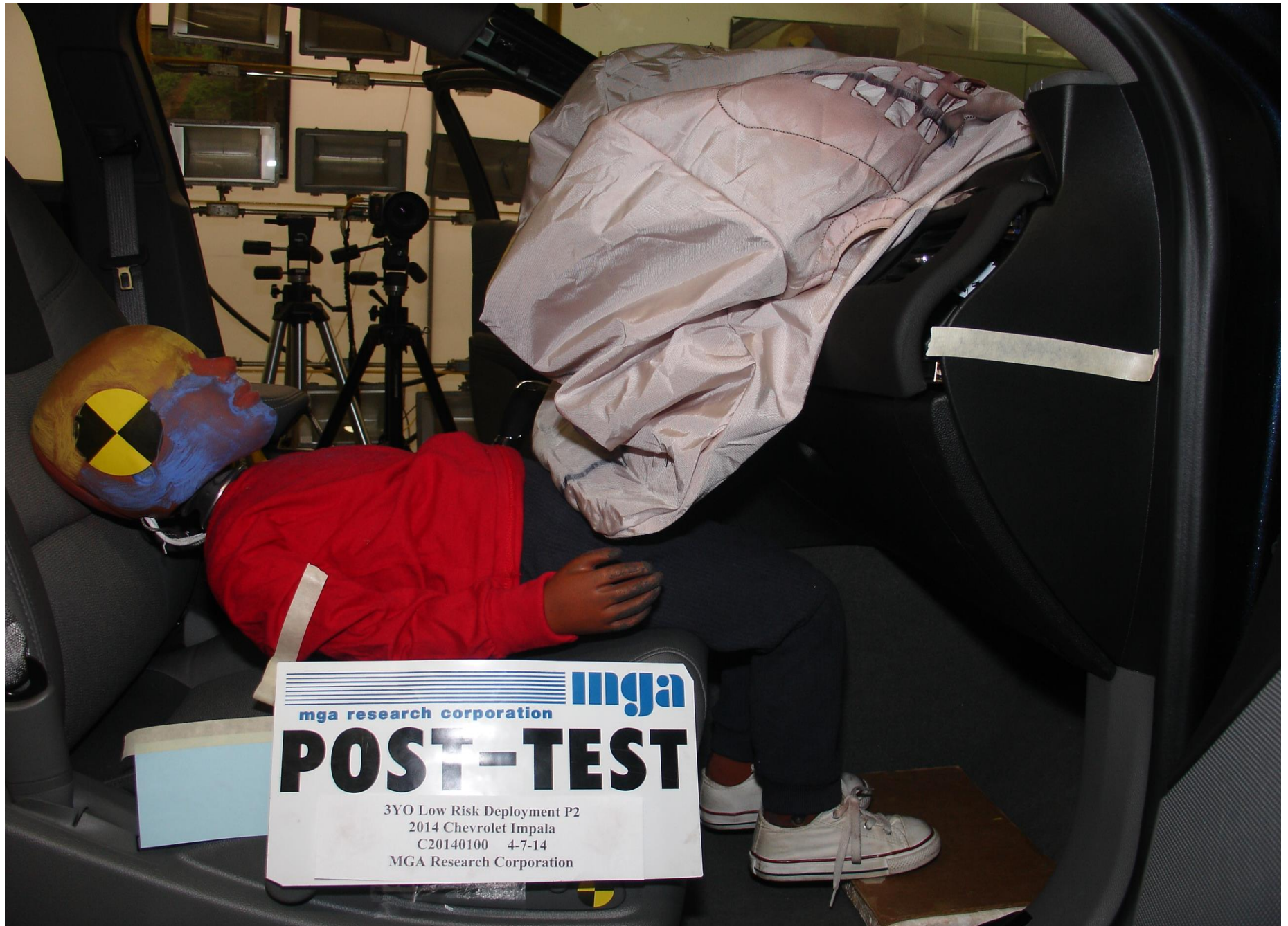
Post-Test 3YO P2 Passenger Dummy Right Side View
