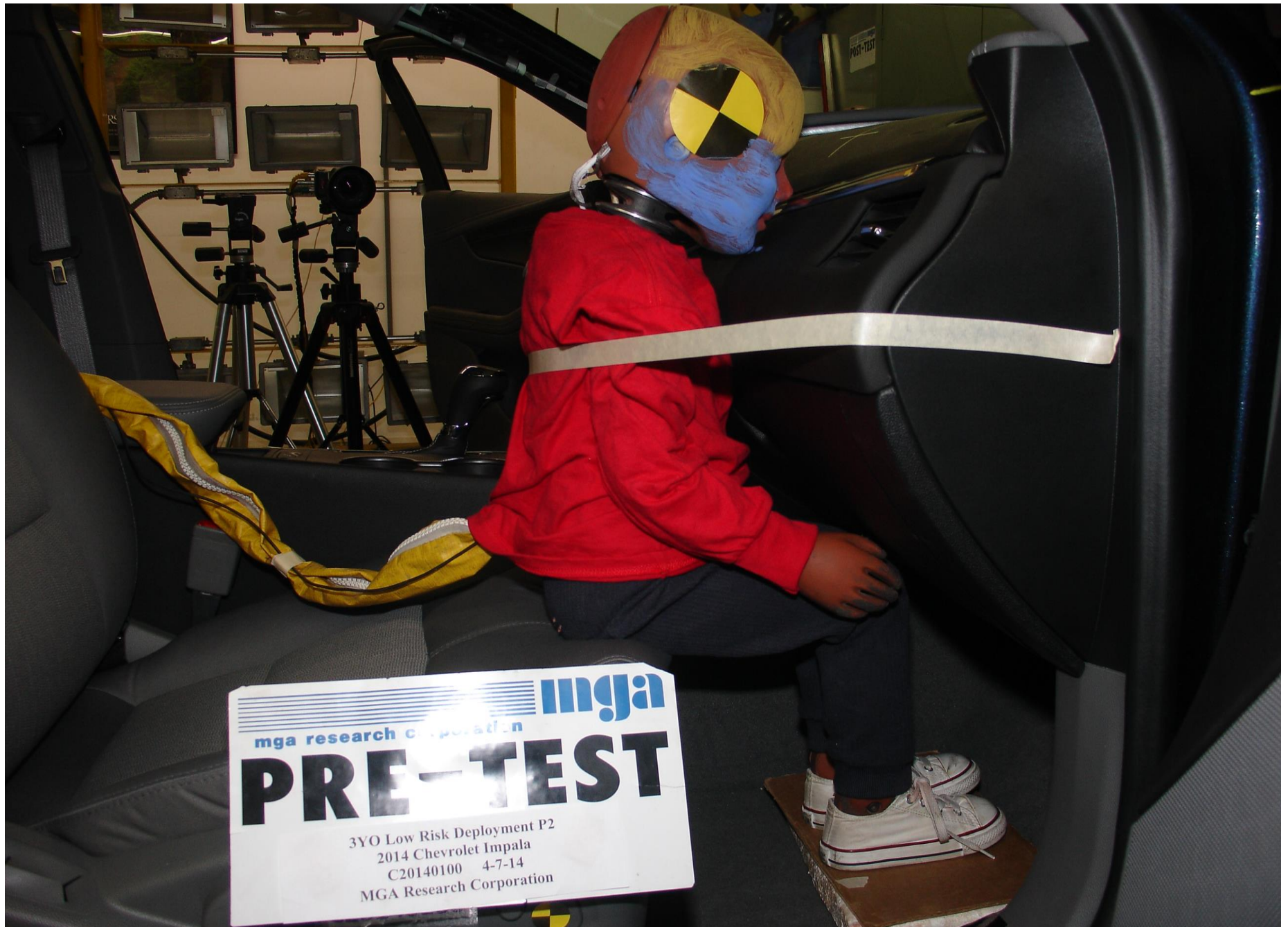
Pre-Test 3YO P2 Passenger Dummy Right Side View
