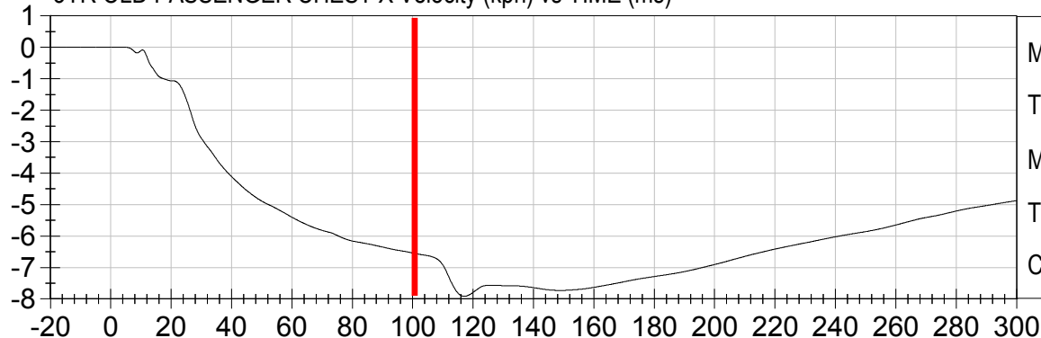
3YR OLD PASSENGER CHEST Y Velocity (kph) vs TIME (ms)
