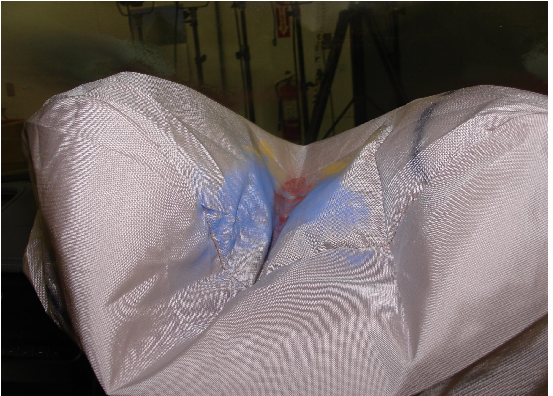
Post-Test 3YO P1 Passenger Dummy Airbag Right Side View
