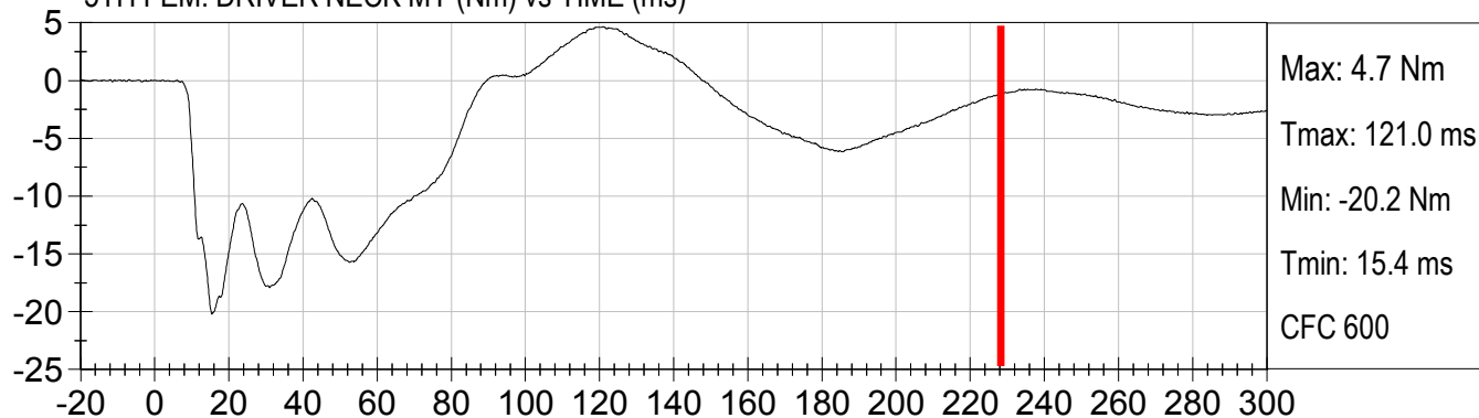
5TH FEM. DRIVER NECK MZ (Nm) vs TIME (ms)
