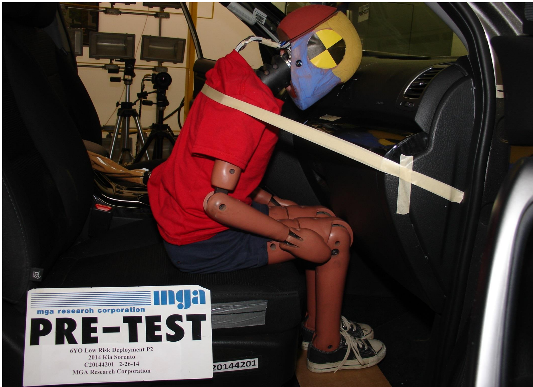
Pre-Test 6YO P2 Passenger Dummy Right Side View
