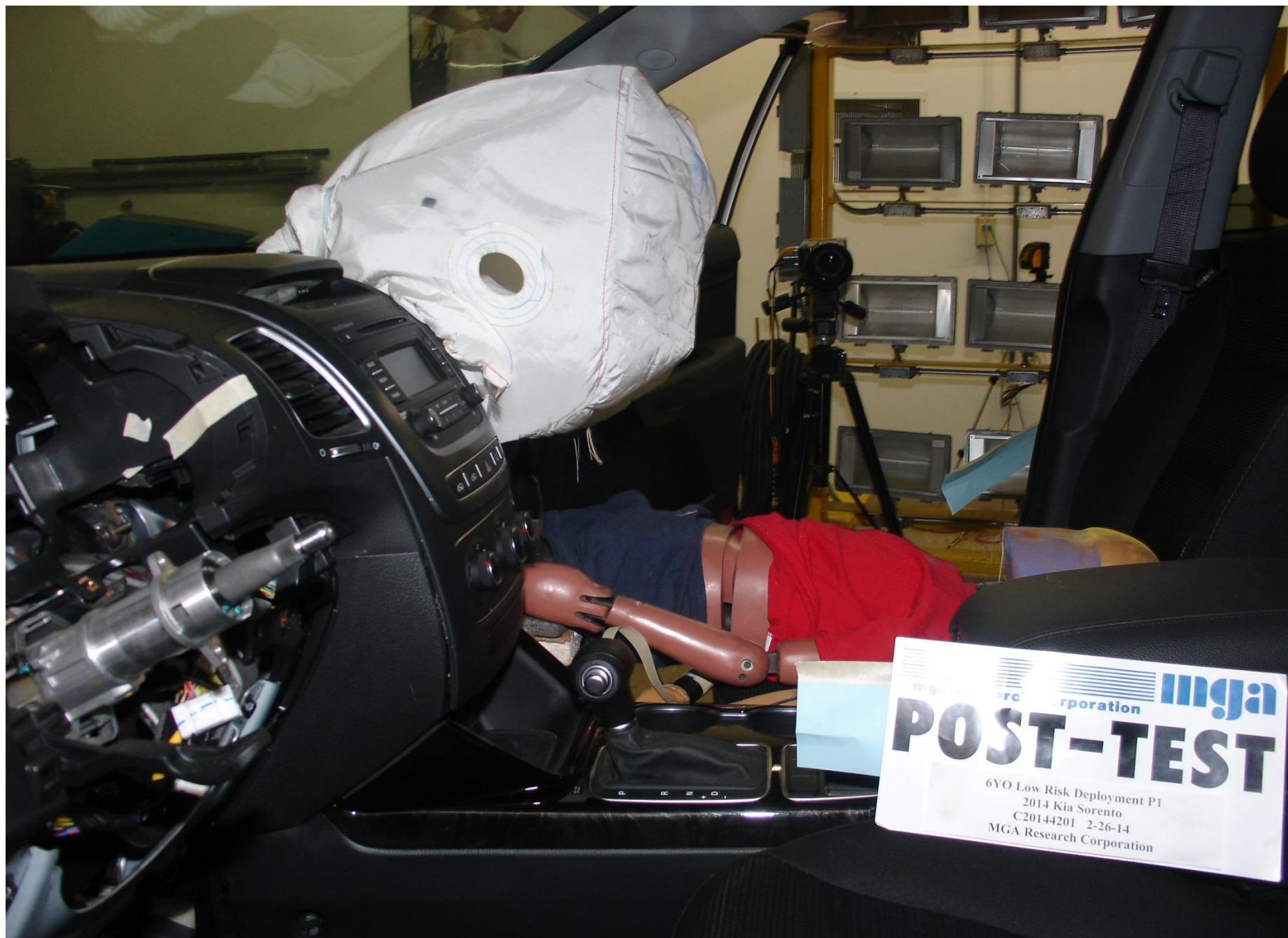
Post-Test 6YO P1 Passenger Dummy Left Side View
