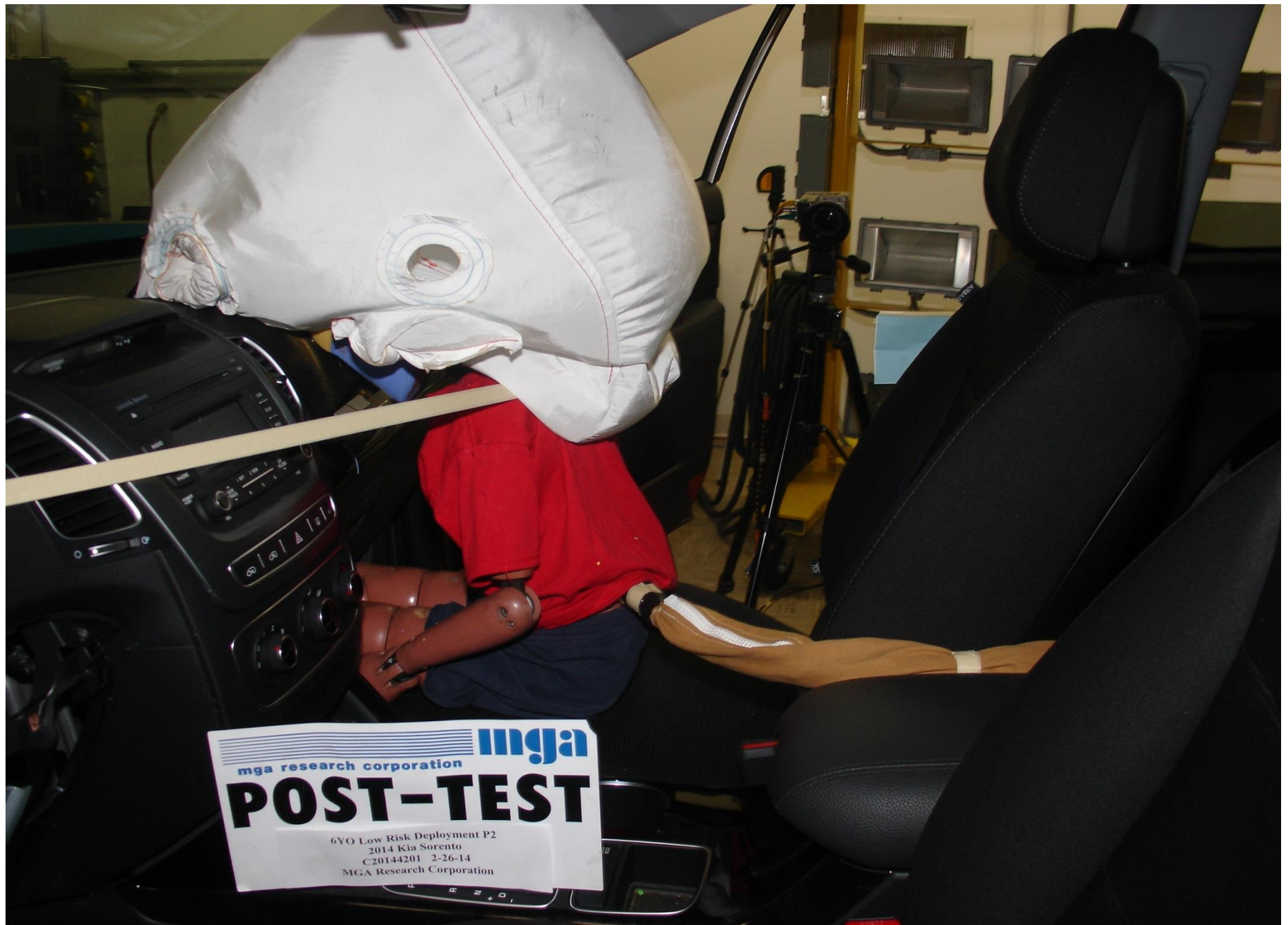
Post-Test 6YO P2 Passenger Dummy Left Side View
