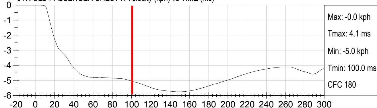
6YR OLD PASSENGER CHEST Y Velocity (kph) vs TIME (ms)
