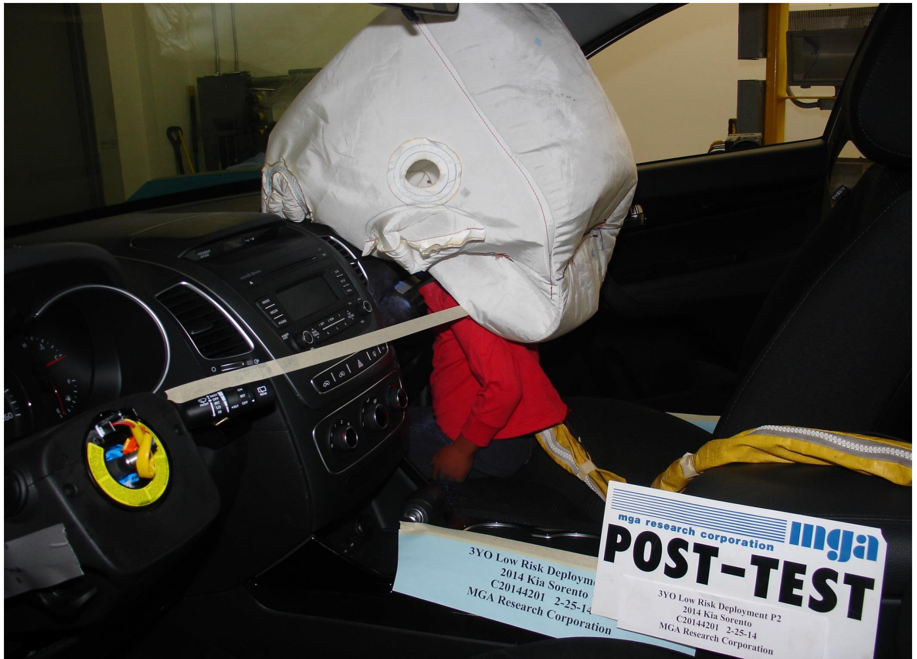
Post-Test 3YO P2 Passenger Dummy Left Side View
