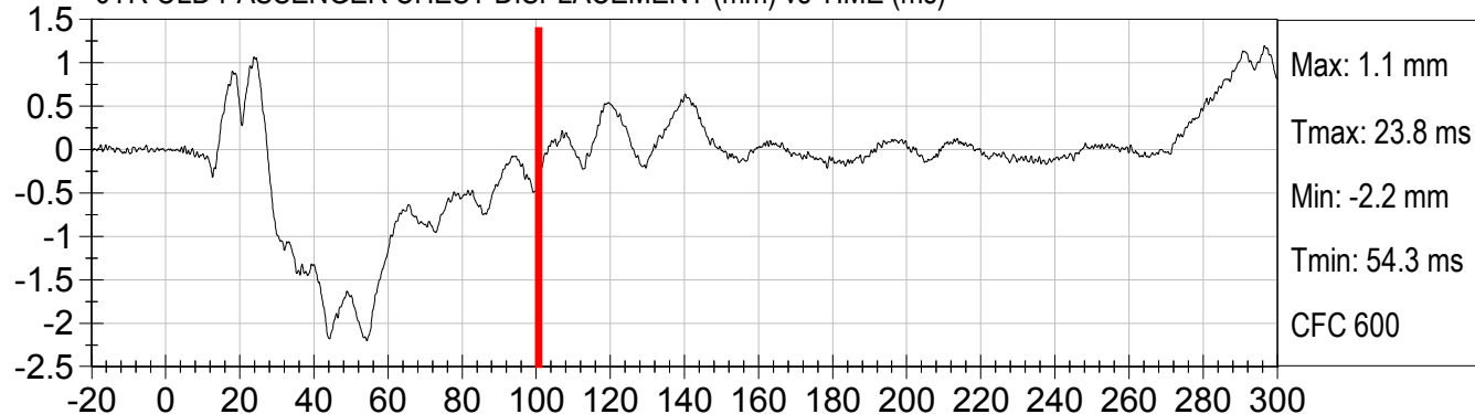
6YR OLD PASSENGER CHEST DISPLACEMENT (mm) vs TIME (ms)
