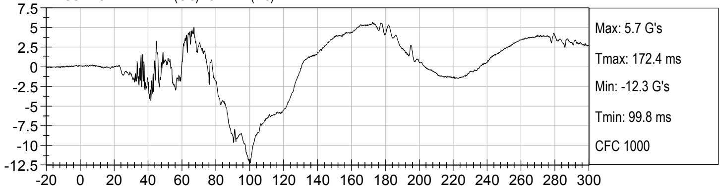
PASSENGER HEAD Resultant (G's) vs TIME (ms)
