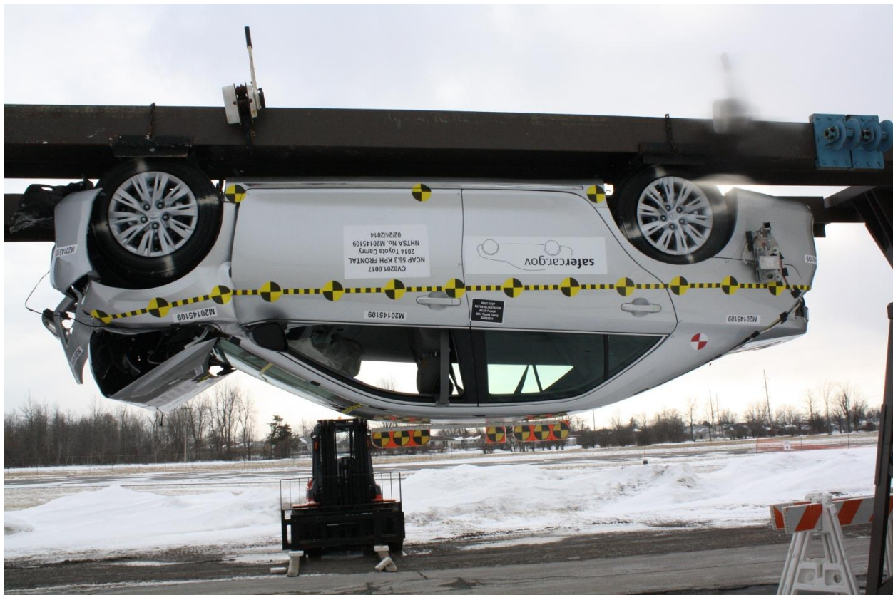
Figure A-74: Vehicle at 180° on Static Rollover Device
