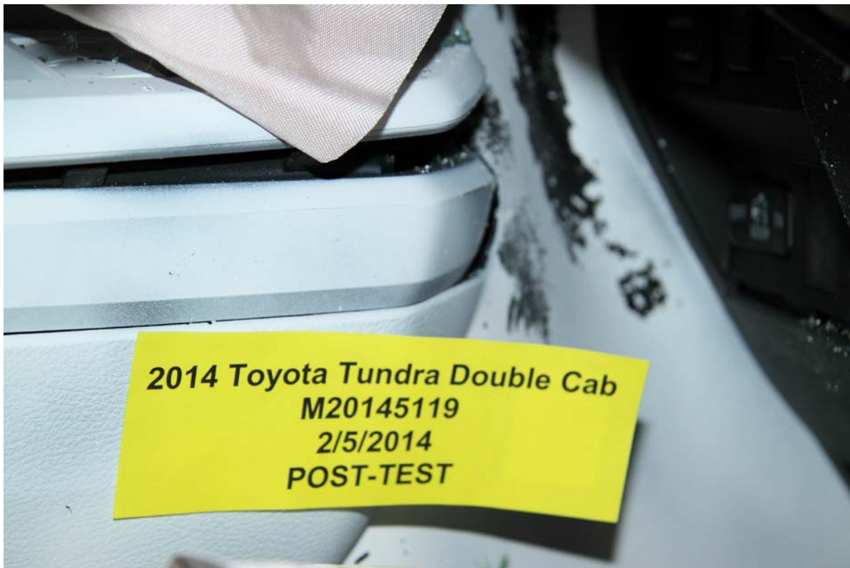
071 Post-Test View of Shattered Vehicle Inner Door Panel
