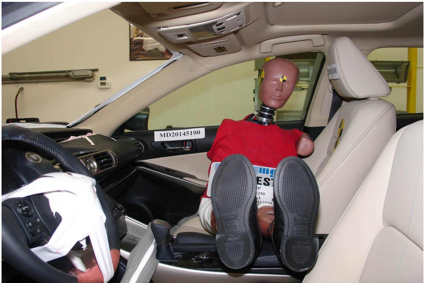
Pre-Test SID-IIs Dummy Left Side View
