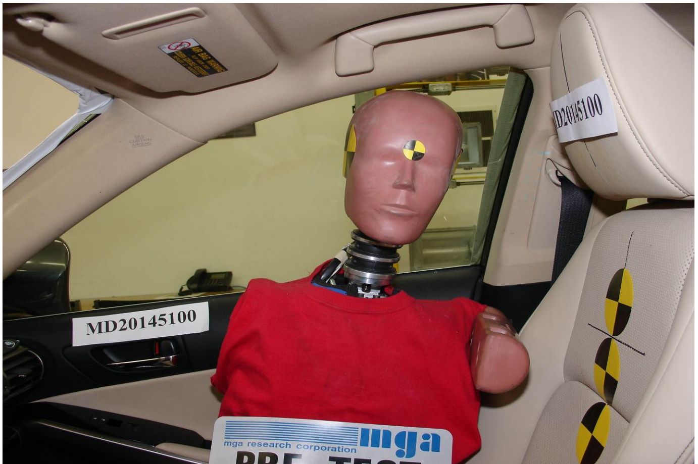
Pre-Test SID-IIs Dummy Left Side Closeup View
