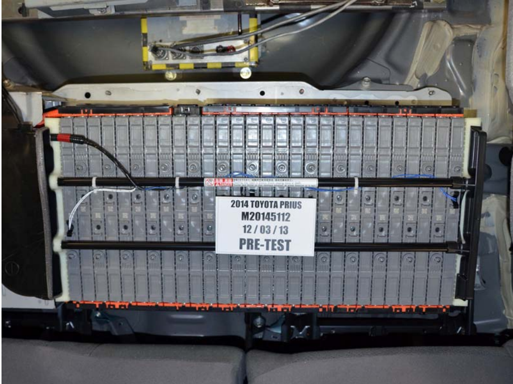
FIGURE 14. Pre-Impact View of Propulsion Battery Modules
