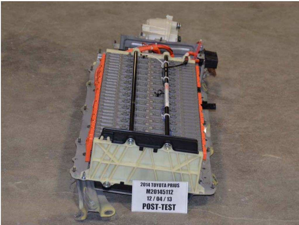
FIGURE 15d. Post-Impact View of Propulsion Battery Modules
