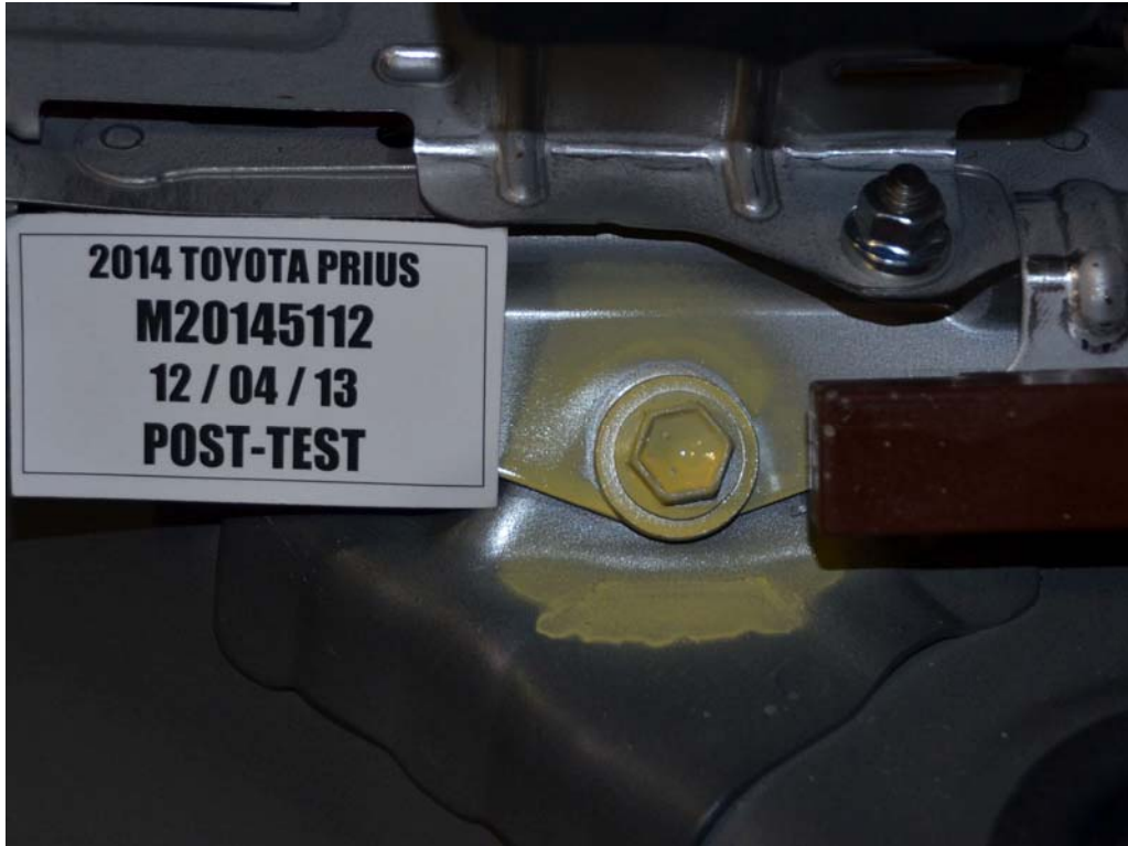
FIGURE 37. Post-Impact View of Battery Module Movement or Retention Loss
