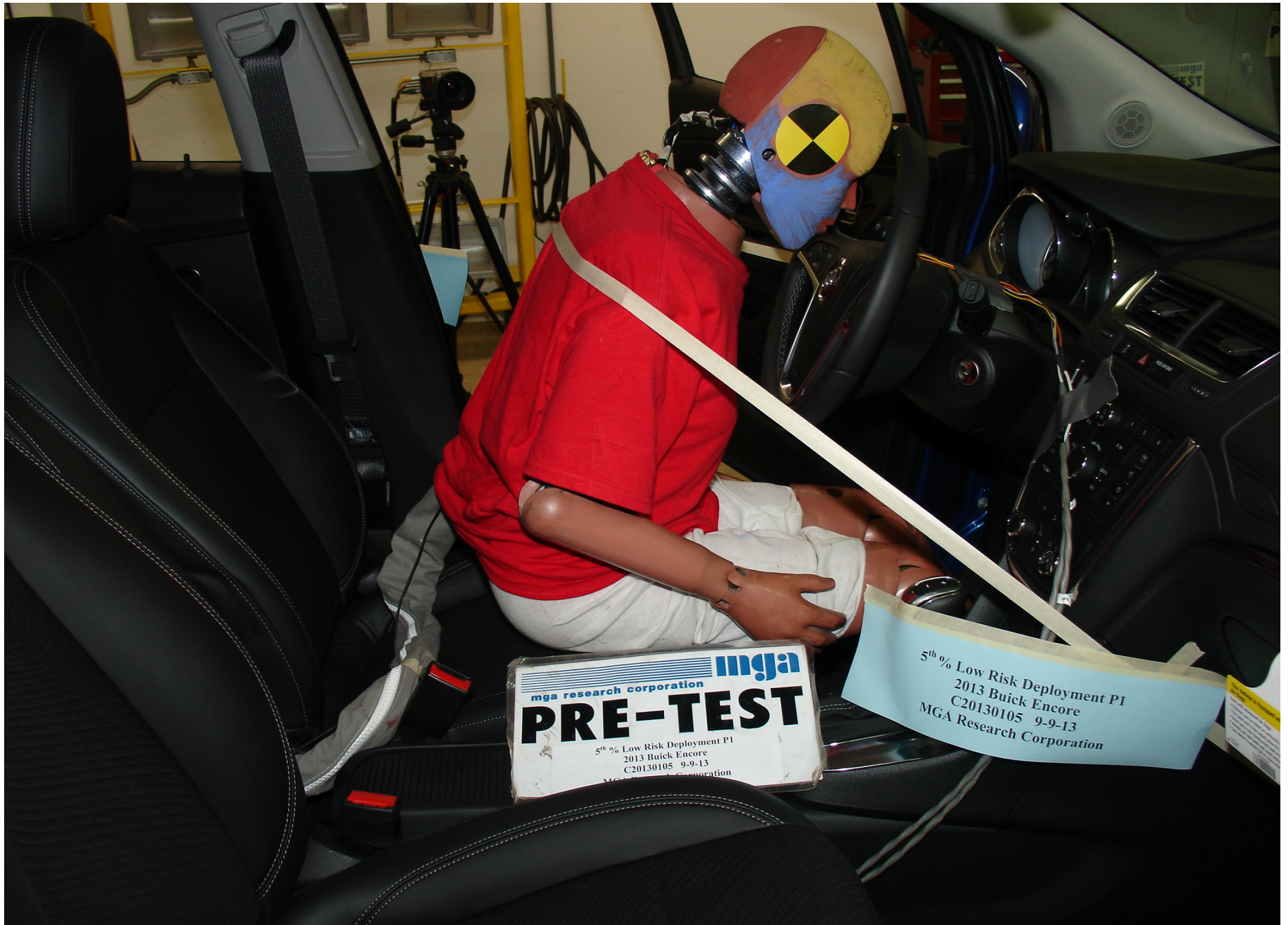
Pre-Test 5th Fem. P1 Driver Dummy Right Side View
