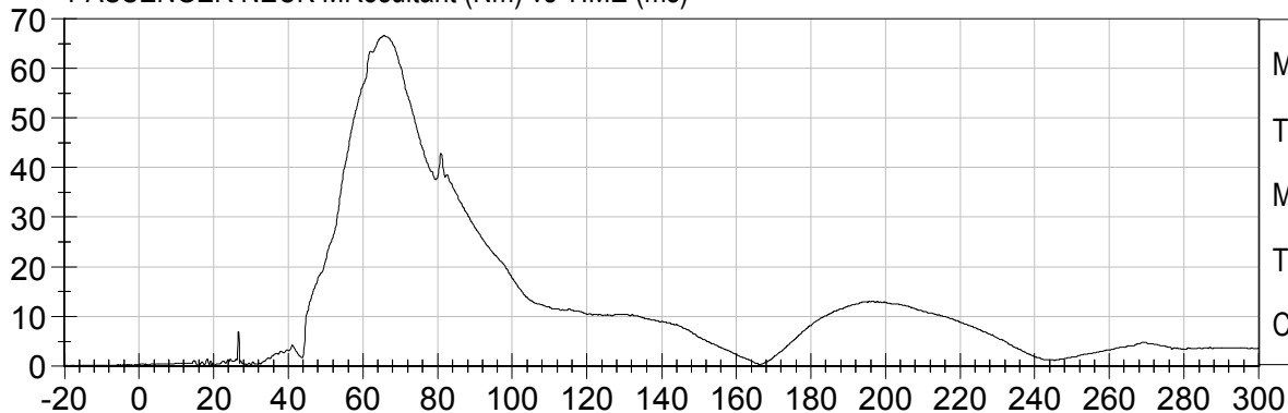
PASSENGER NECK MResultant (Nm) vs TIME (ms)
