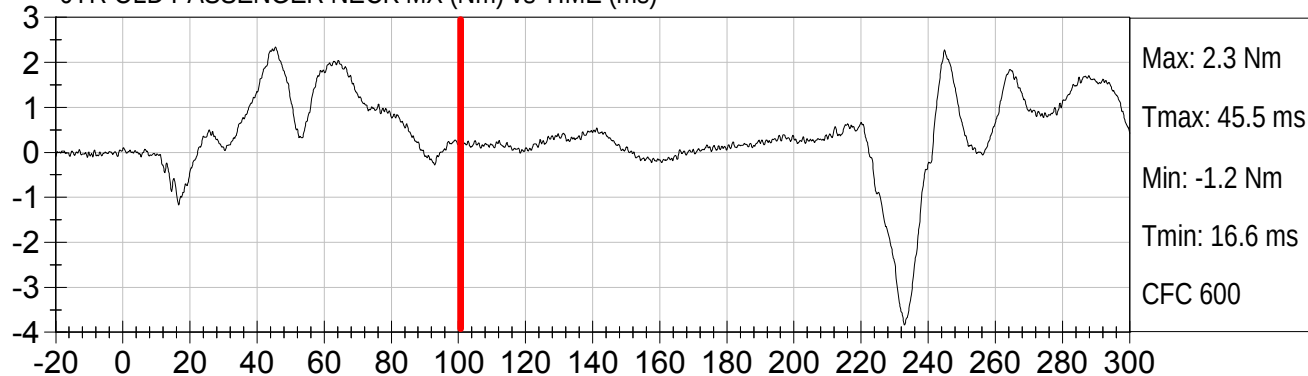
6YR OLD PASSENGER NECK MY (Nm) vs TIME (ms)
