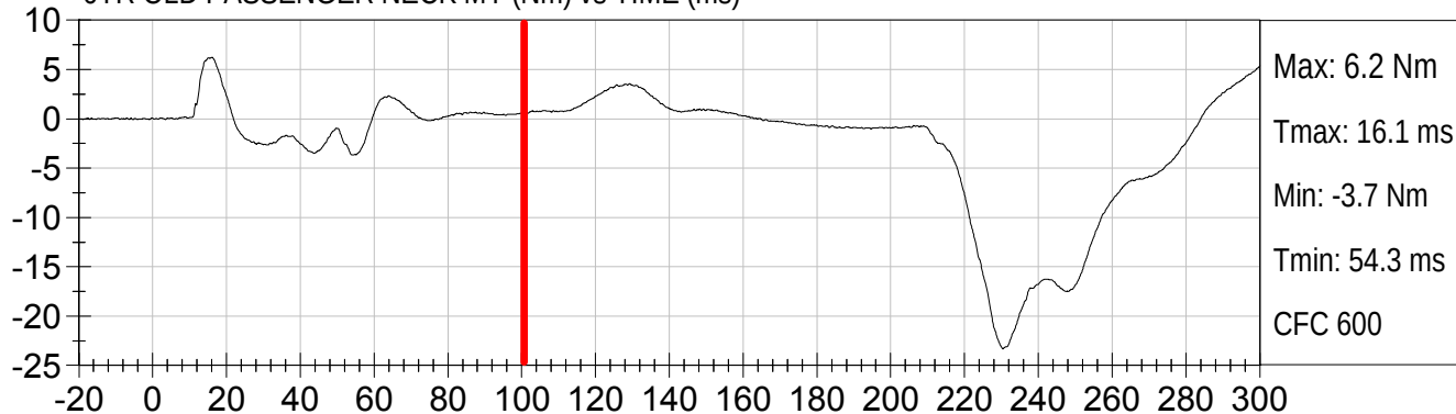
6YR OLD PASSENGER NECK MZ (Nm) vs TIME (ms)
