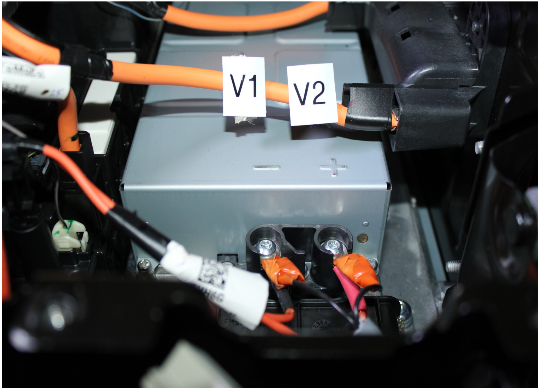
Pre-Test Voltage Monitoring Leads Attached to Electric Energy Storage System
