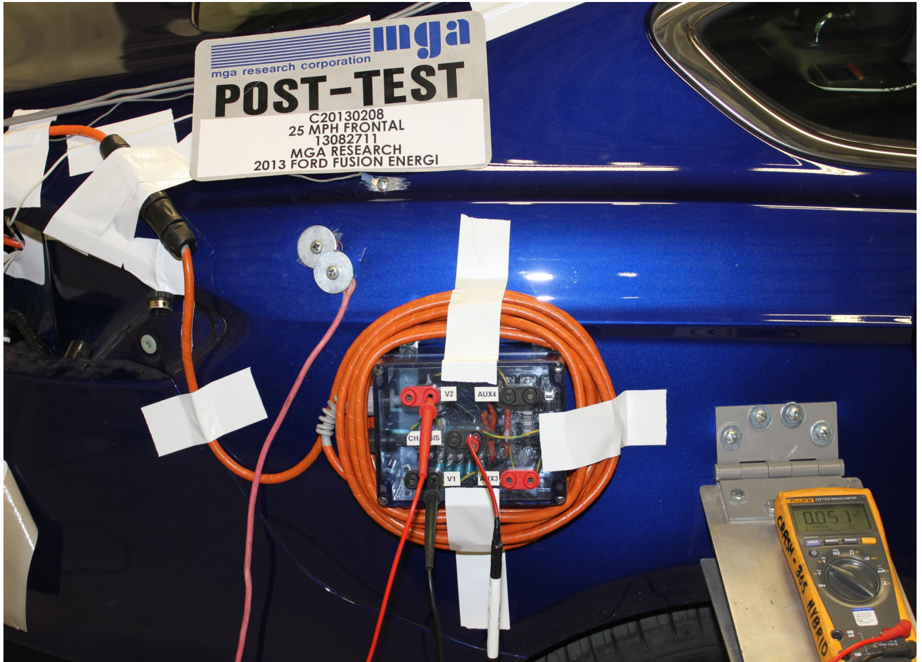
Post-Test View of Installed Isolation Interface Port
