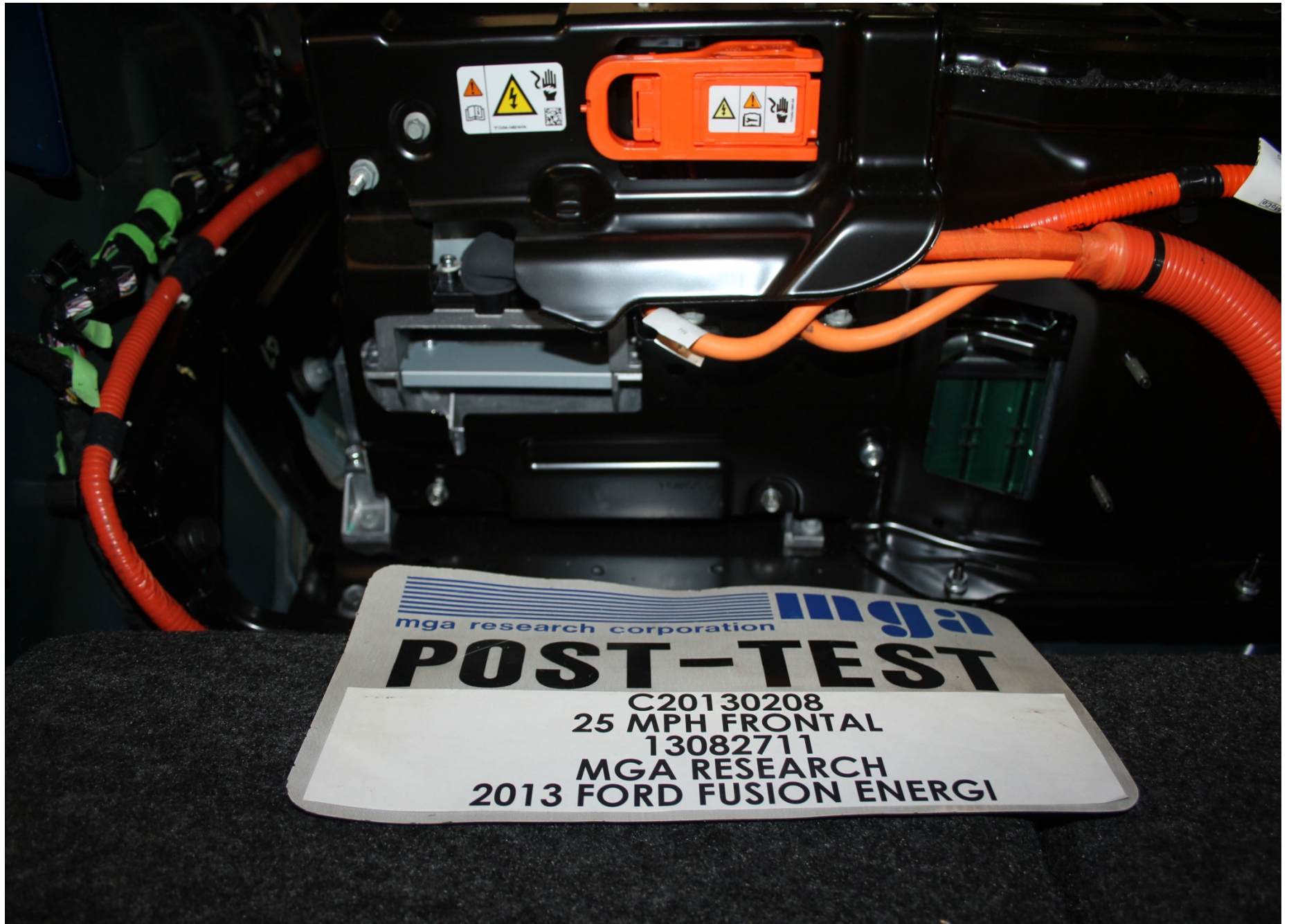
Post-Test Manual High Voltage Service Disconnect in Place
