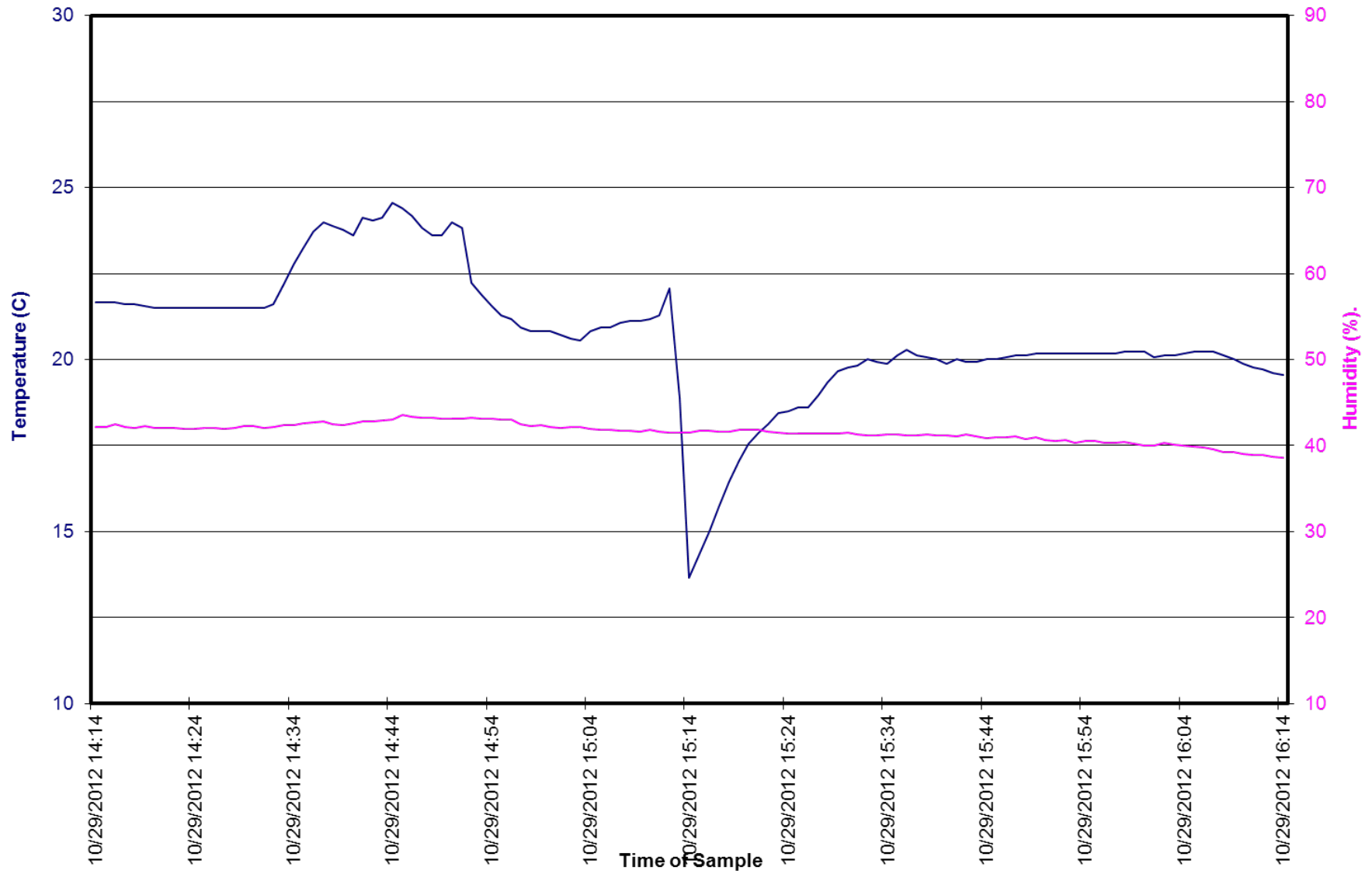
FMVSS 214 Side Impact 2011 Hyundai Tucson 121029; Test Time 16:14
