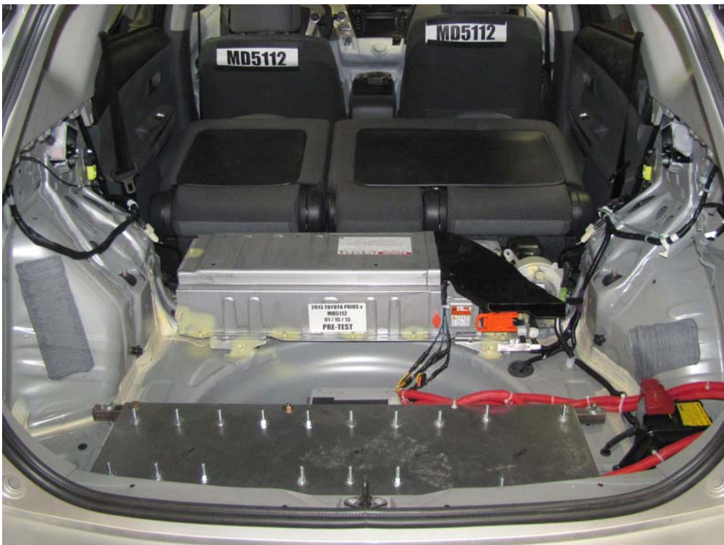
FIGURE 33a. Pre-Impact View of Vehicle Passenger Compartment Adjacent to Propulsion Battery
