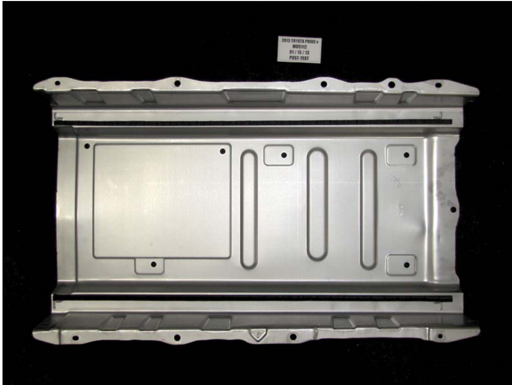
FIGURE 13c. Post-Impact View of Battery Box or Container Which Hold Individual Battery Modules
