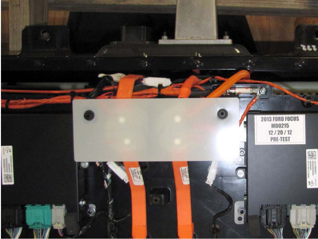
FIGURE 22a. Pre-Impact View of High Voltage Leads Attached
