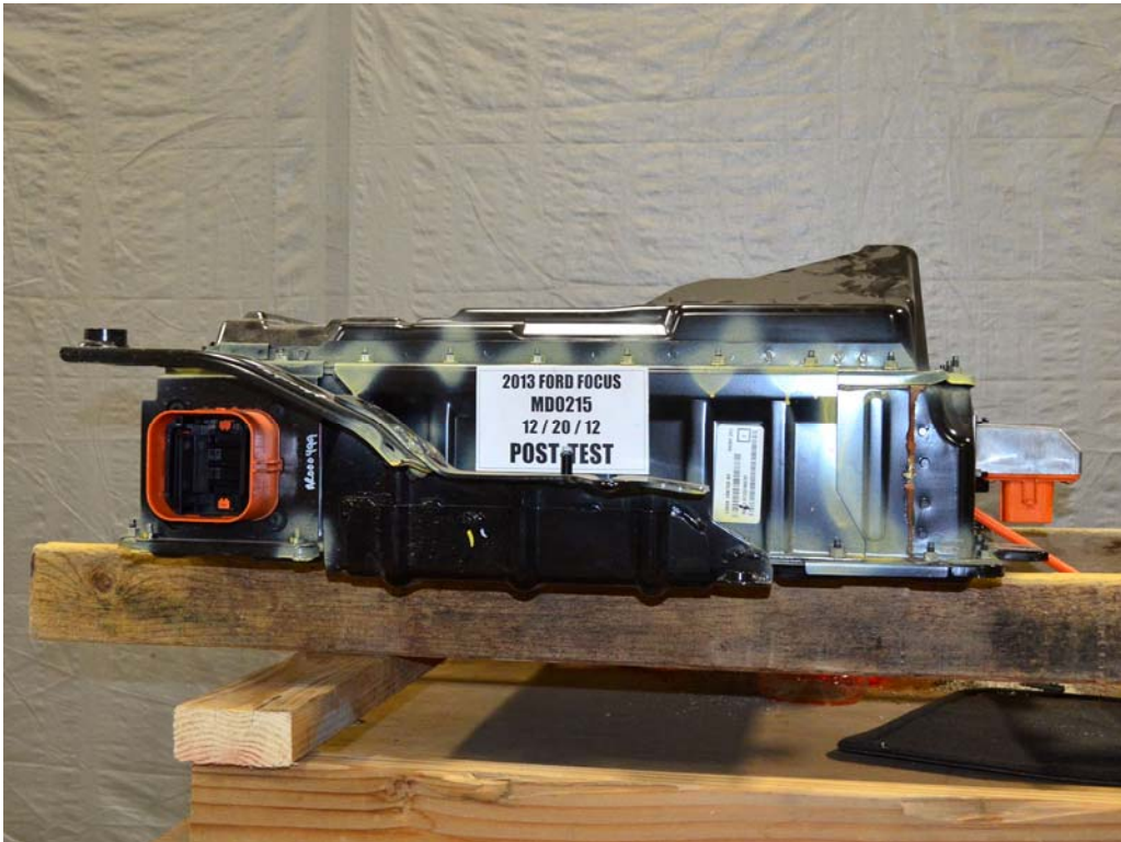
FIGURE 13e. Post-Impact View of Battery Box or Container Which Hold Individual Battery Modules
