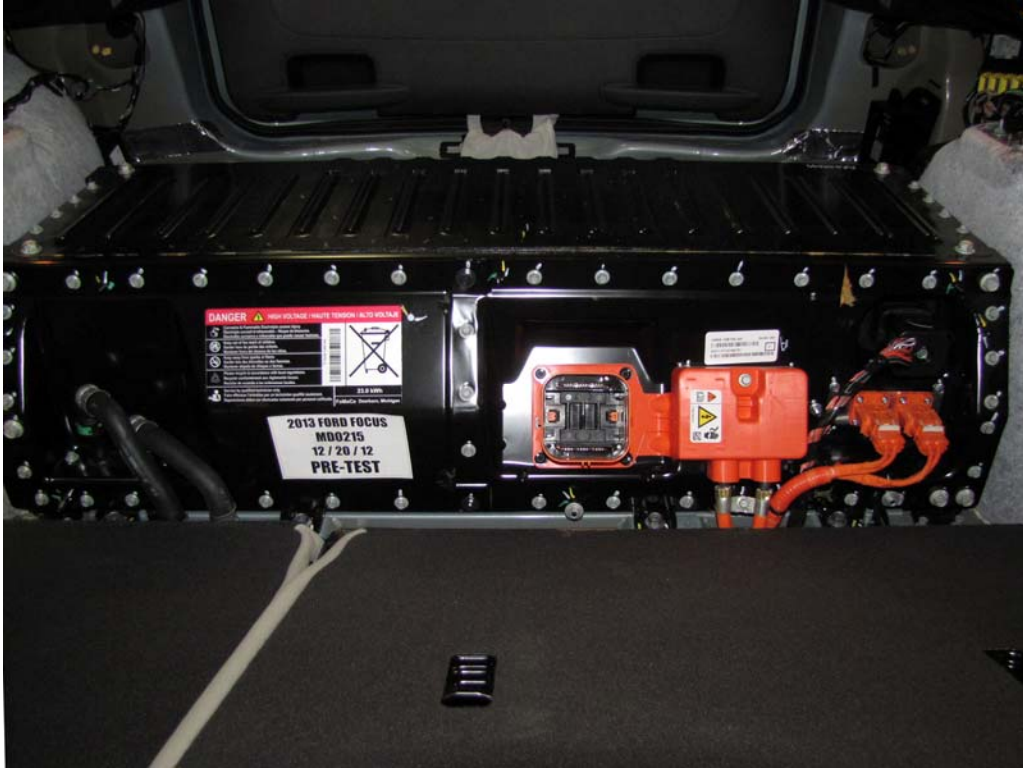
FIGURE 33. Pre-Impact View of Vehicle Passenger Compartment Adjacent to Propulsion Battery
