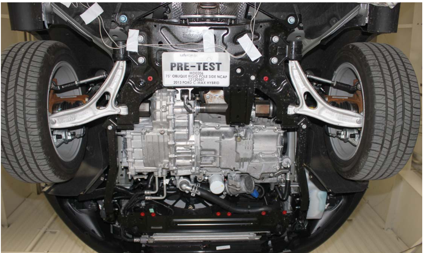
No. 020 Pre-Impact View of Other Visible Electric Propulsion Components
