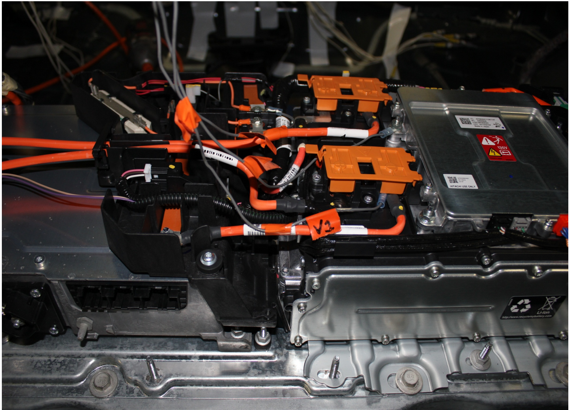
Post-Test Positive and Negative Attachment Point to the Propulsion Battery System
