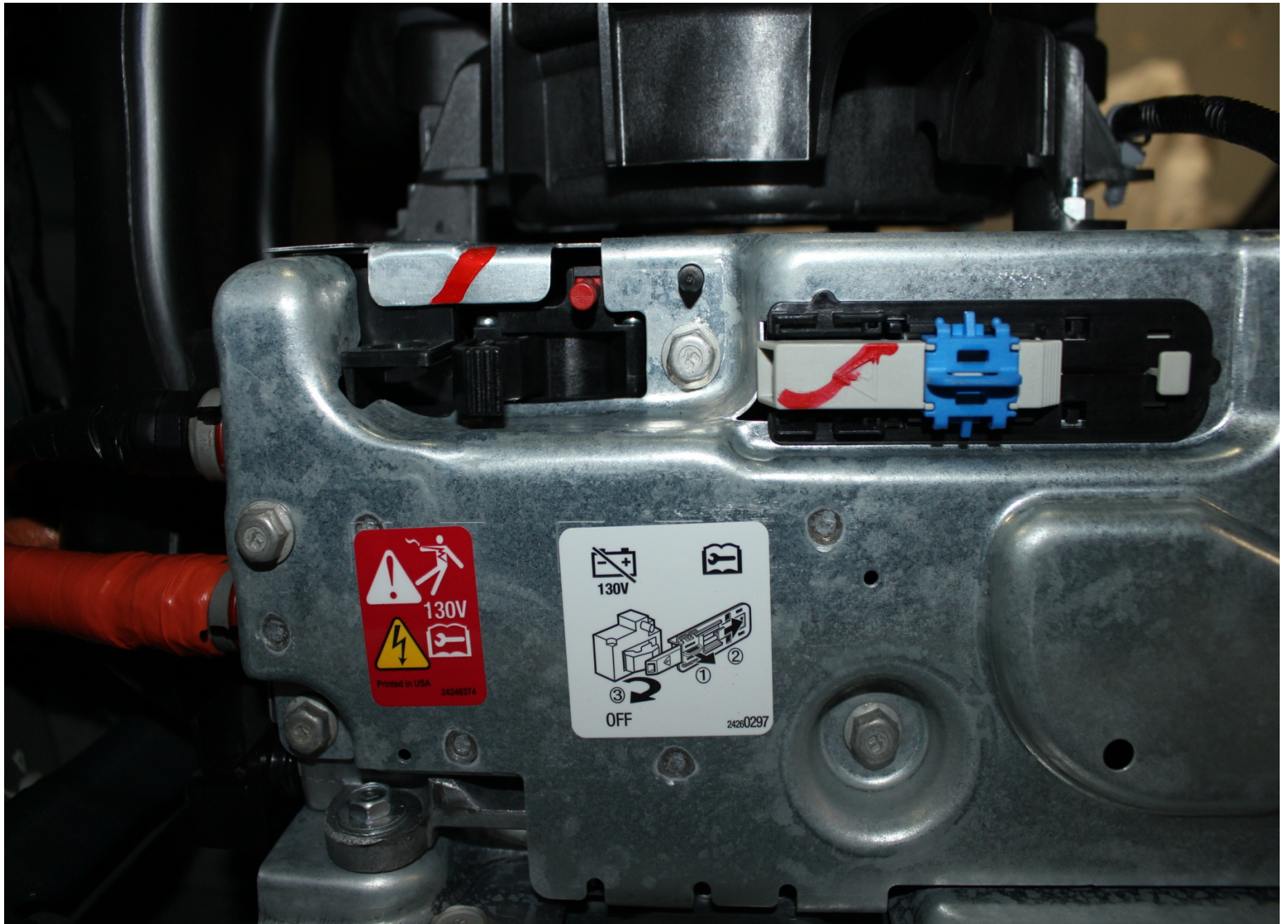
Pre-Test Manual High Voltage Service Disconnect Plug
