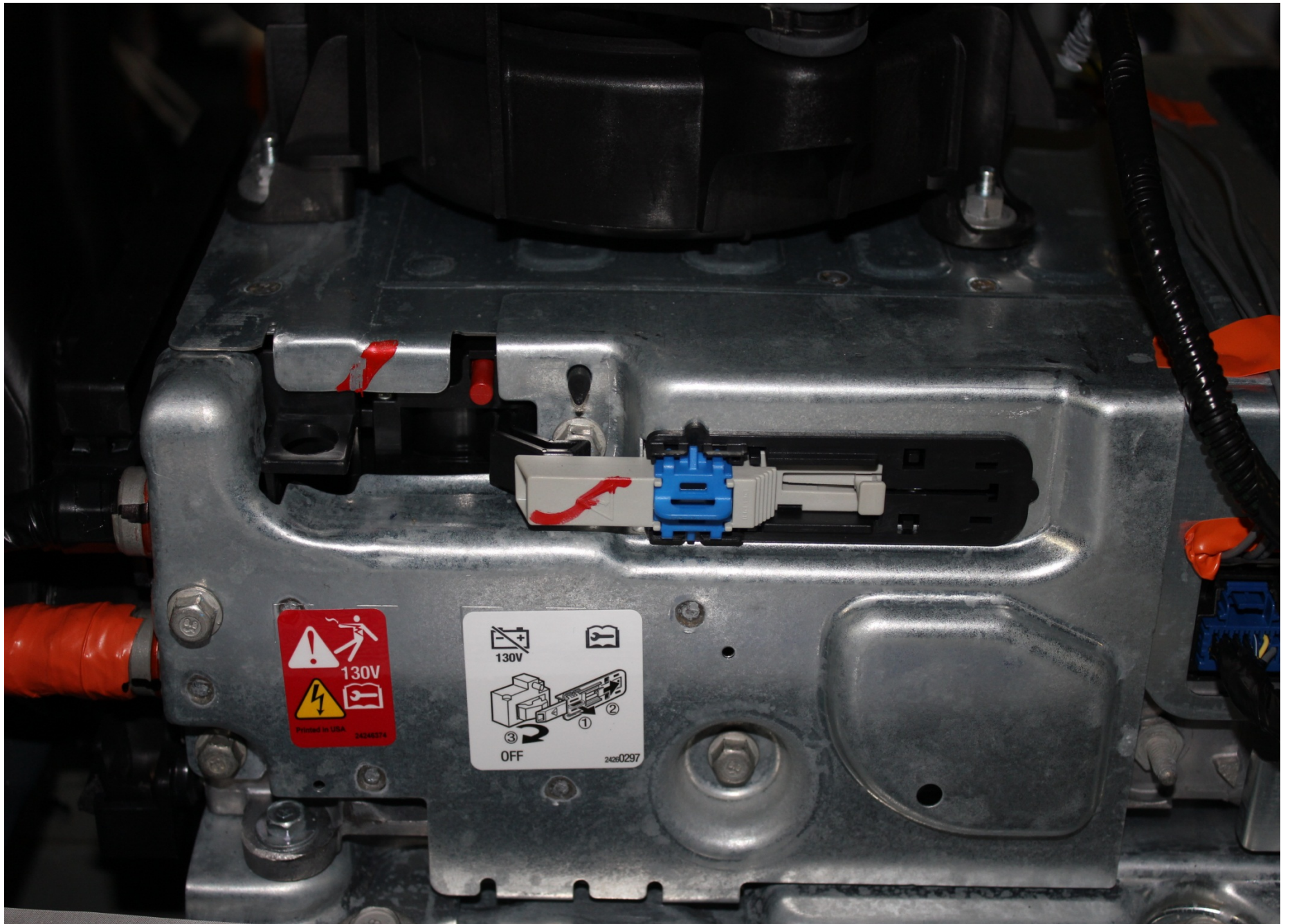
Post-Test Manual High Voltage Service Disconnect Plug
