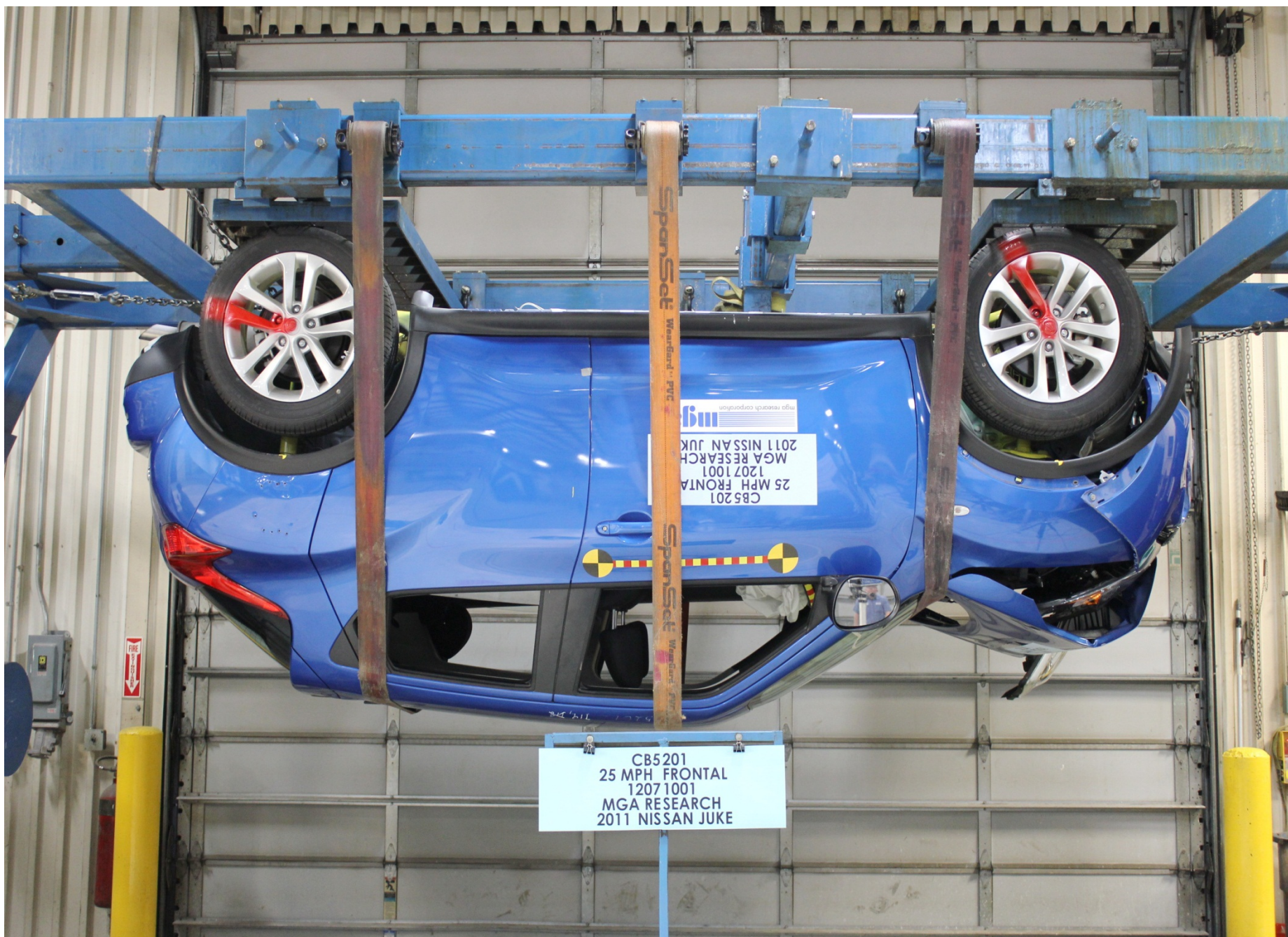
Rollover 180 Degrees
