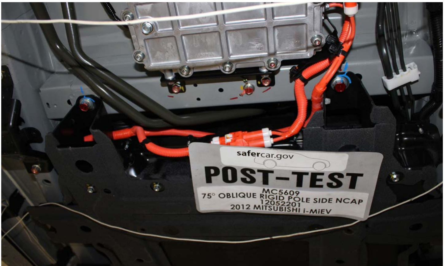
No. 036c Post-Impact View of Battery Module Movement or Retention Loss
