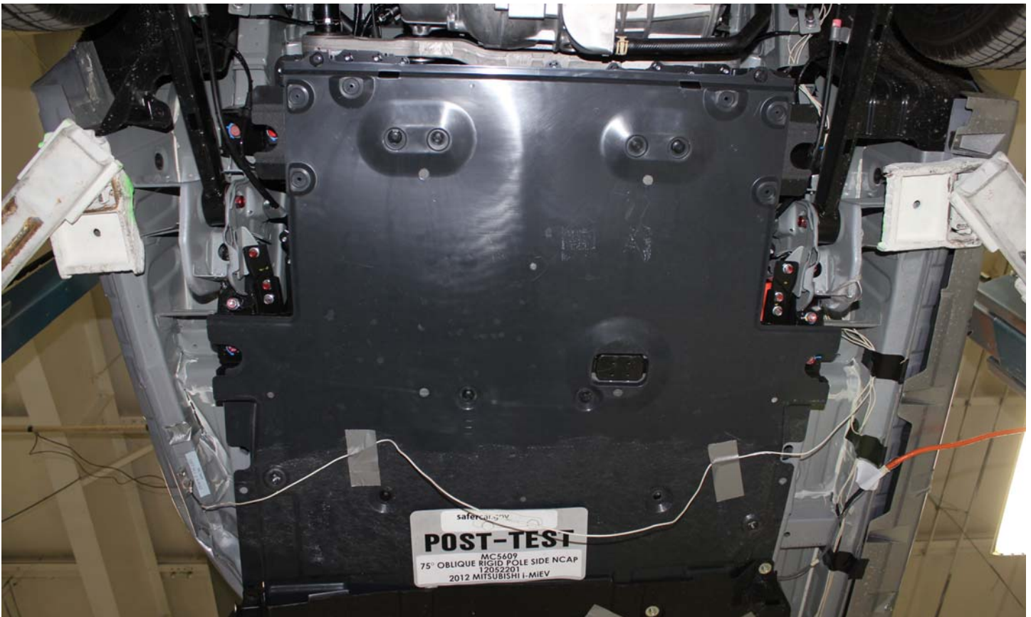
No. 013a Post-Impact View of Battery Box(s) or Container(s) Which Holds Individual Battery Modules
