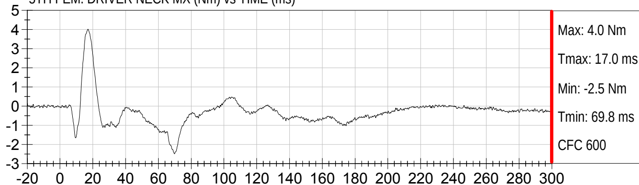
5TH FEM. DRIVER NECK MY (Nm) vs TIME (ms)
