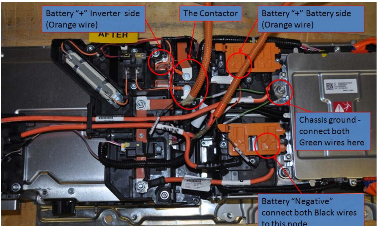
No. 043 Electric Energy Storage-Conversion Test Points
