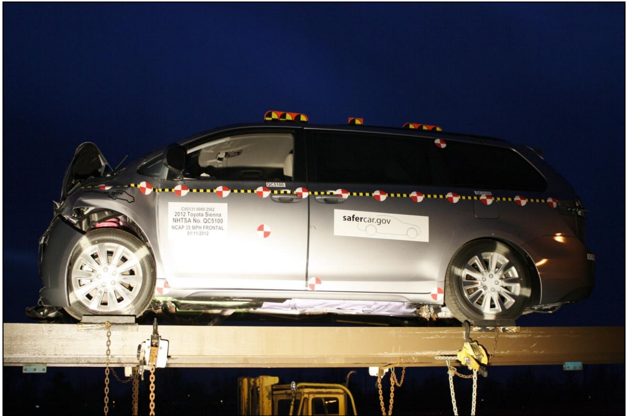
Figure A-66: Vehicle at 0° on Static Rollover Device
